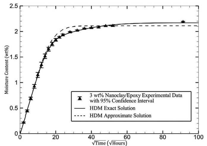
Figure 1. Comparison between the experimental moisture absorption results for a 3wt% nanoclay/epoxy composite, and the predictions obtained from the exact and approximate solutions of the hindered diffusion model (HDM).
