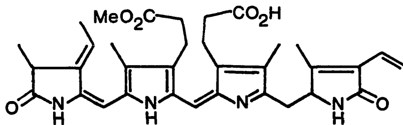
90 alysiaviolin
