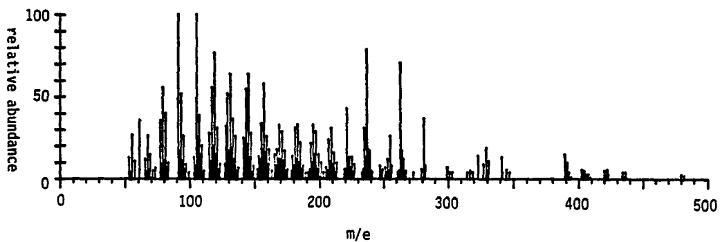
Mass Spectrum of 118
