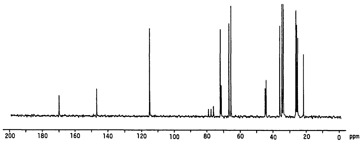
Figure 15. 22.50 MHz ^{13}\text{C} -NMR ( \text{CDCl}_3 ) Spectrum of Isoobtusol Acetate ( 108 ).
