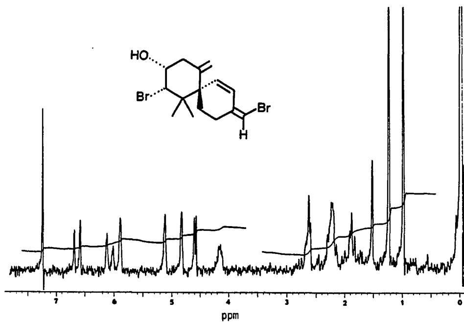
100 MHz PMR Spectrum of 104a in CDCl 3
