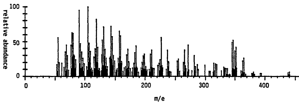
Mass Spectrum of 121
