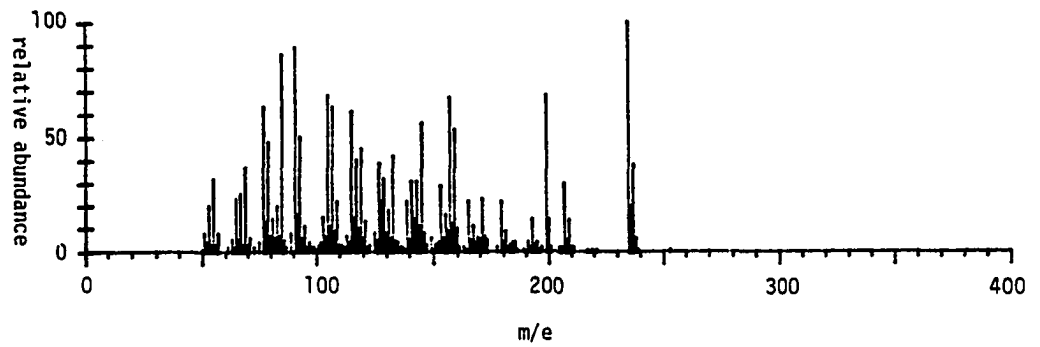
Mass Spectrum of Elatol Acetate
