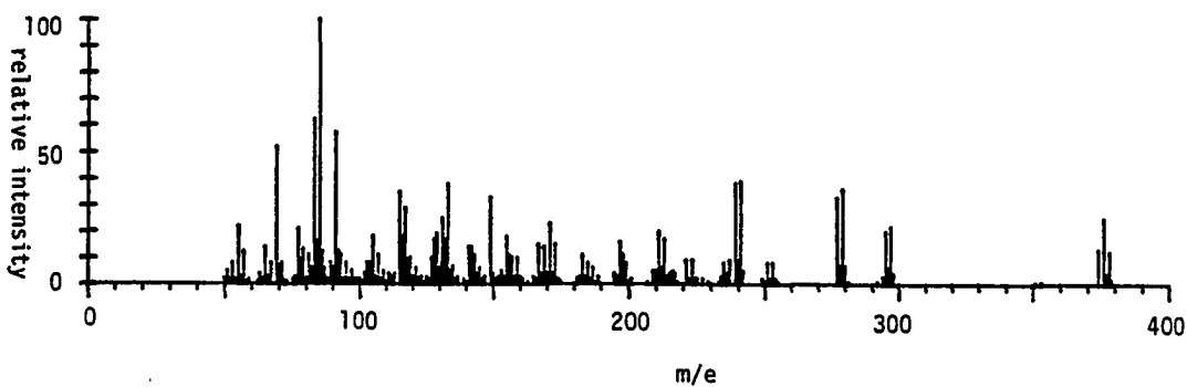
Mass Spectrum of 105a
