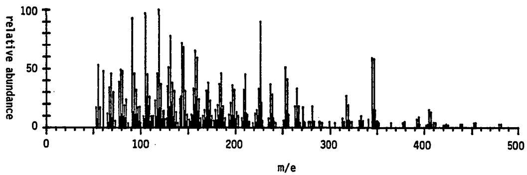
Mass Spectrum of 123
