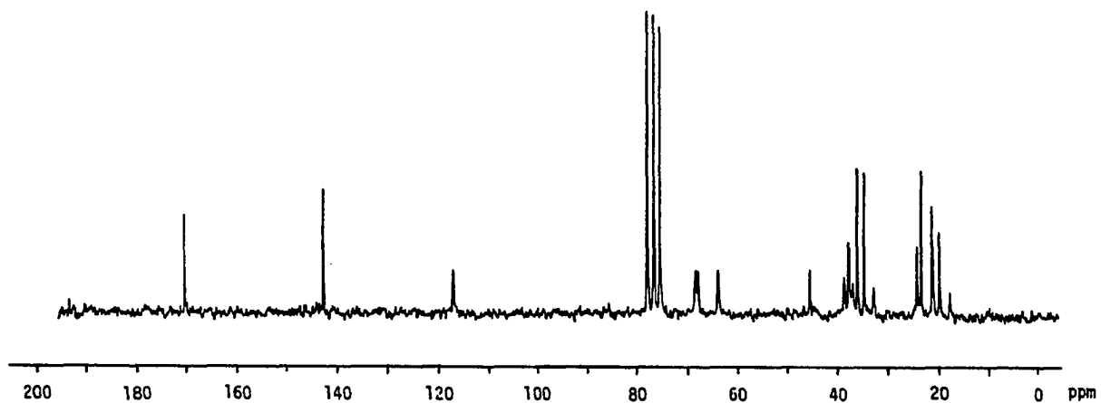
25.05 MHz ^{13}\text{C} -NMR ( \text{CDCl}_3 ) Spectrum of Parguerol ( 109 ).
