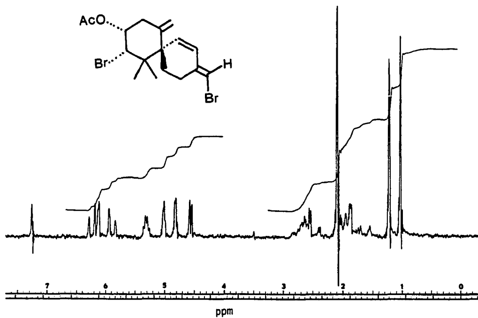
100 MHz PMR Spectrum of 105b in CDCl 3
