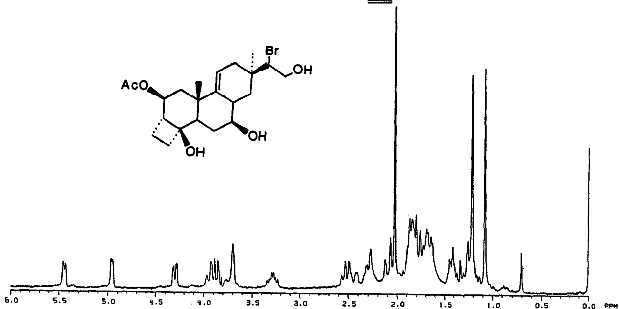
270 MHz PMR Spectrum of 121 in CDCl 3
