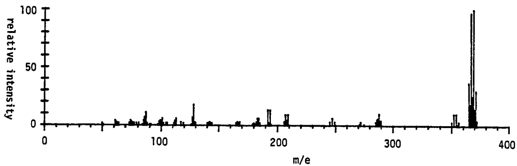
Mass Spectrum of 99
