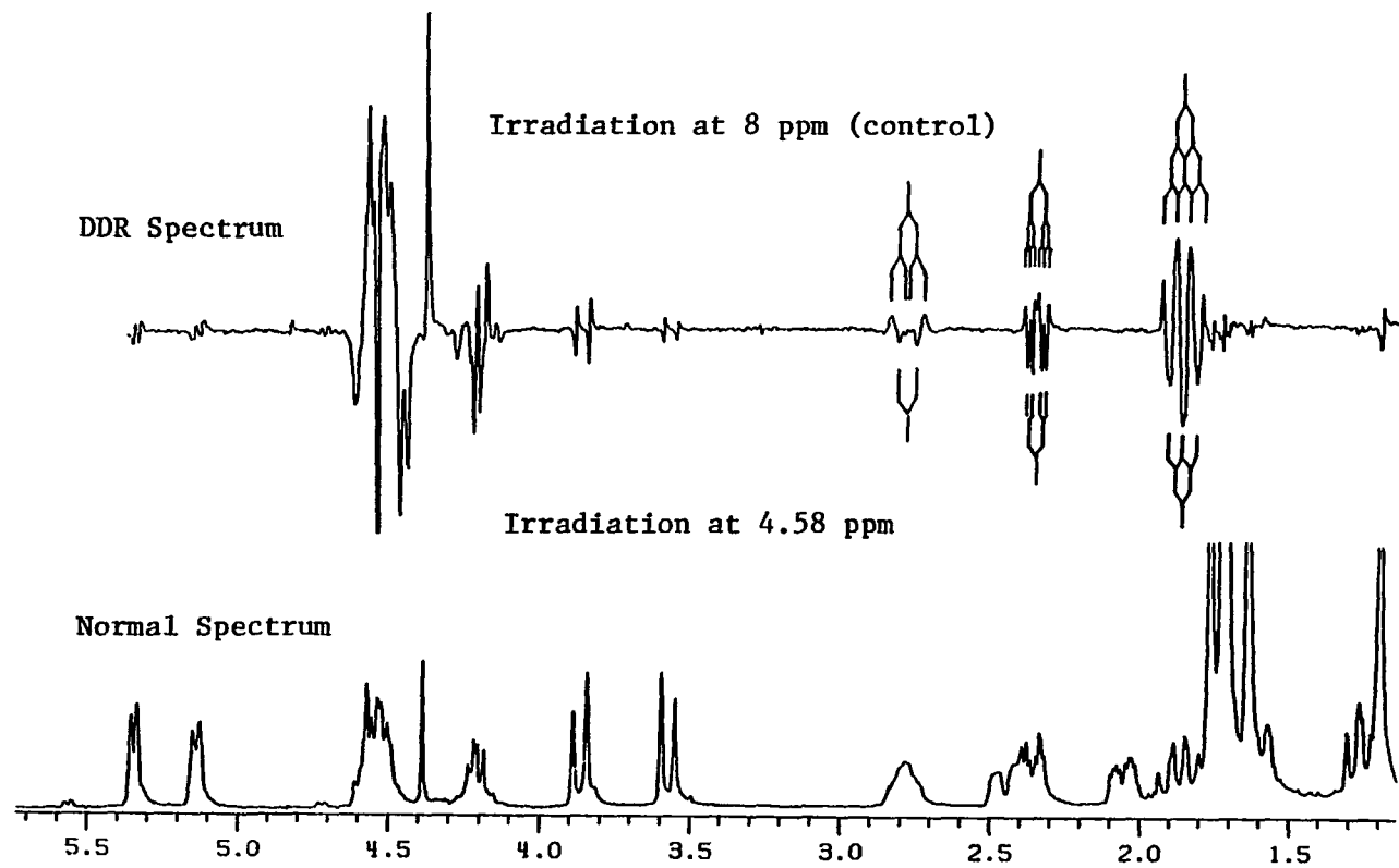
Figure 23. DDR Spectrum of Parguerol acetate ( 110a ) in benzene-d 6 .
