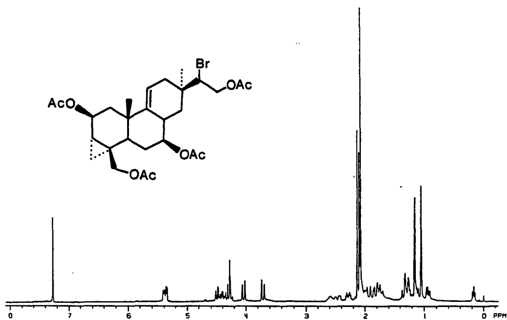
270 MHz PMR Spectrum of 110a in CDCl 3
