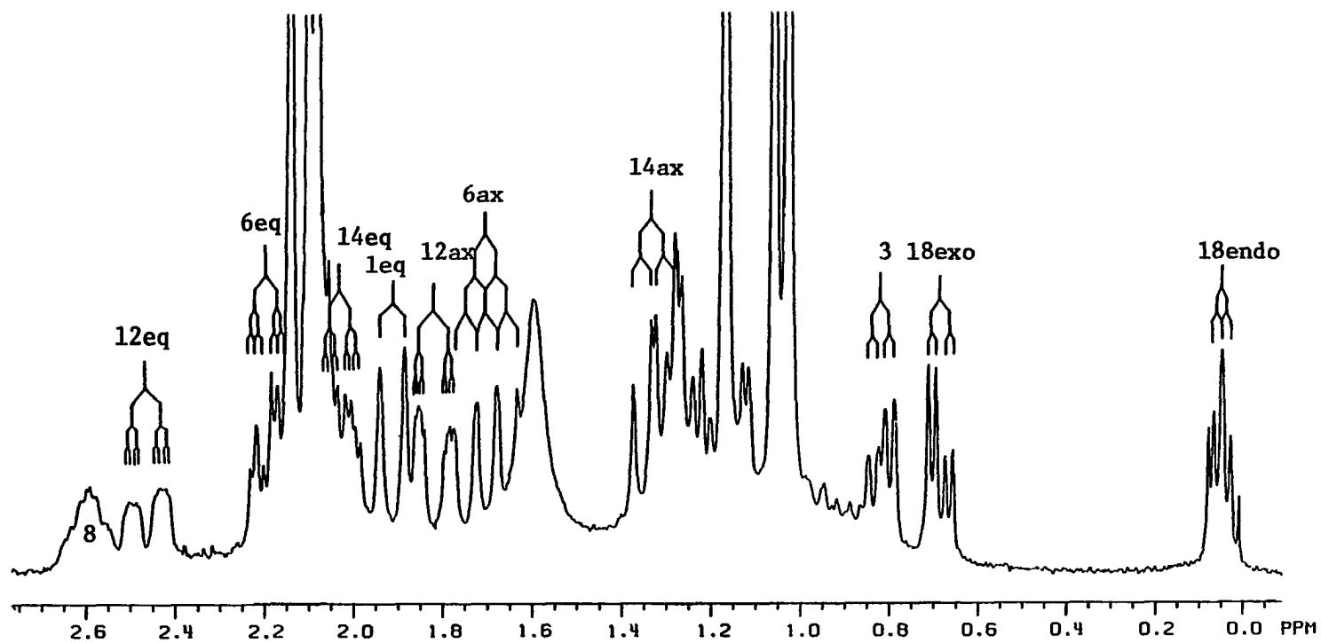
Figure 28. High Field Portion of the 270 MHz PMR Spectrum of 120 in \text{CDCl}_3 .
