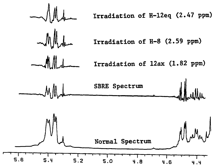
Figure 22. SBRE of parguerol acetate ( 110a ) at 360 MHz.
