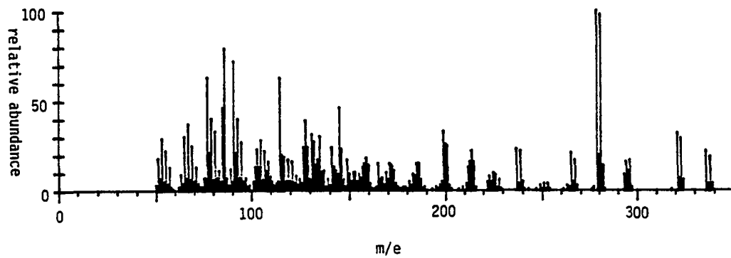
Mass Spectrum of 101
