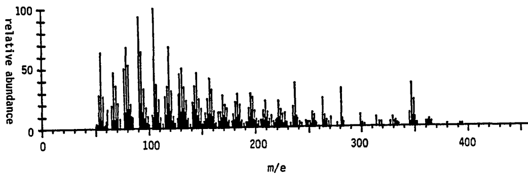
Mass Spectrum of 109
