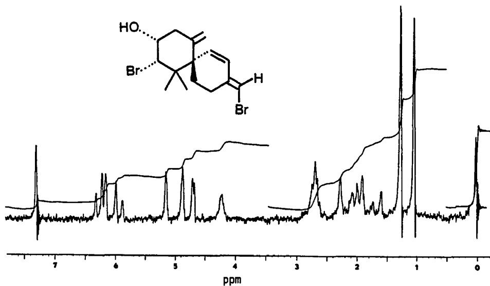
100 MHz PMR Spectrum of 105a in CDCl 3
