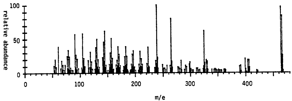
Mass Spectrum of 120
