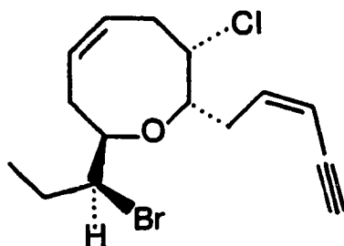
9 cis-dihydrorhodophytin
