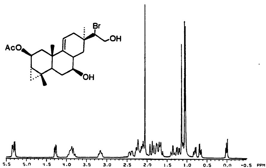
270 MHz PMR Spectrum of 119 in CDCl 3
