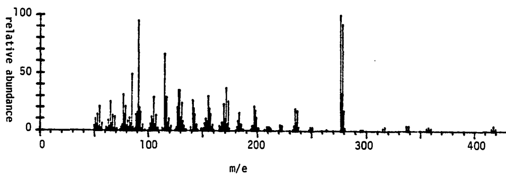
Mass Spectrum of 105b
