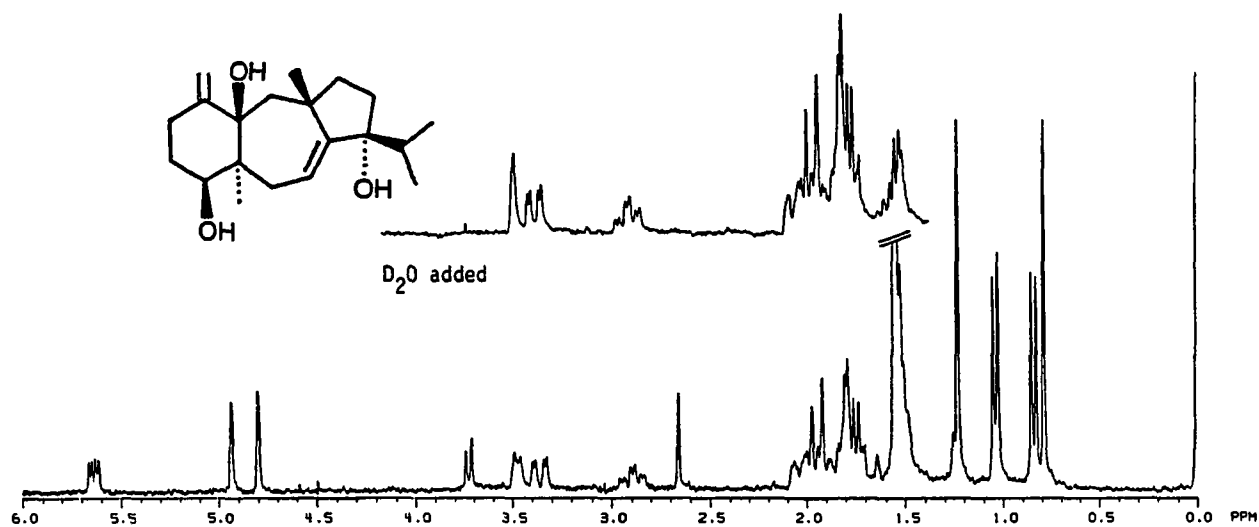
270 MHz PMR Spectrum of 124 in CDCl 3
