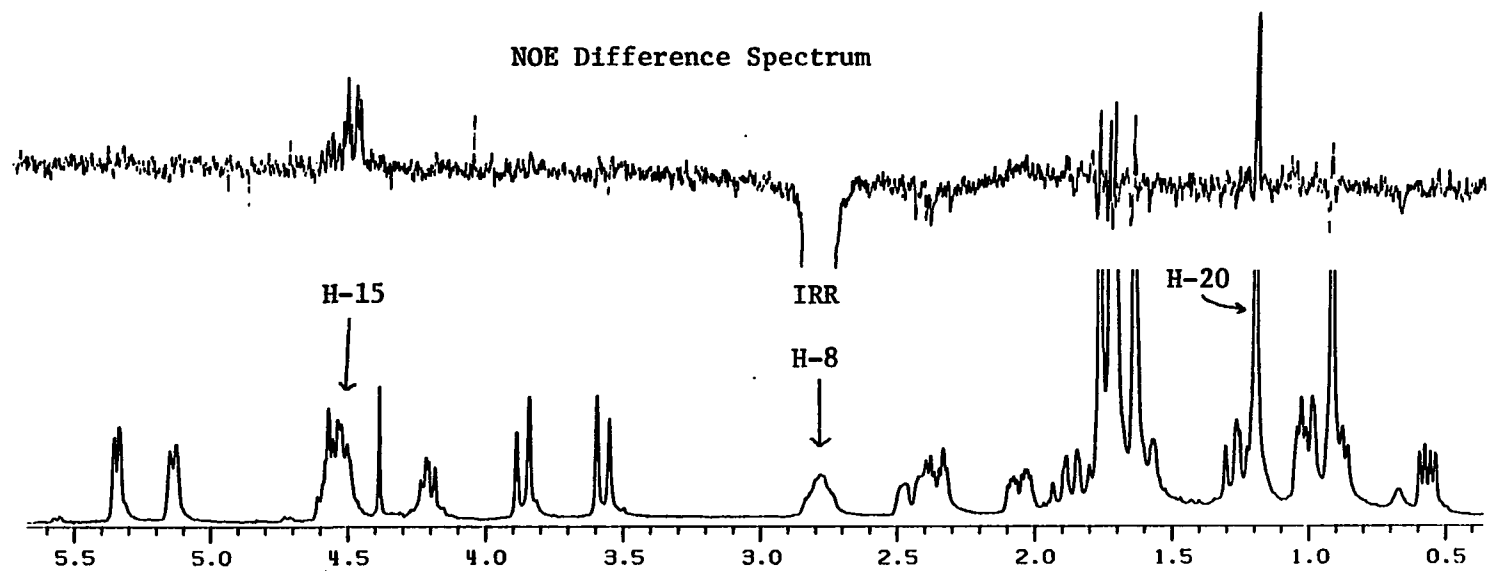
Figure 24. NOE Difference Spectrum of Parguerol Acetate ( 110a ).
