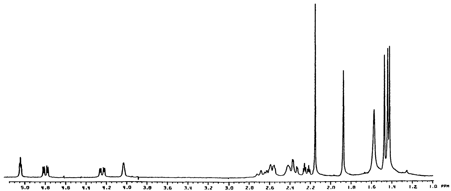
Figure 35. 360 MHz PMR Spectrum of Dihydroxydeodactol Monoacetate (32)
