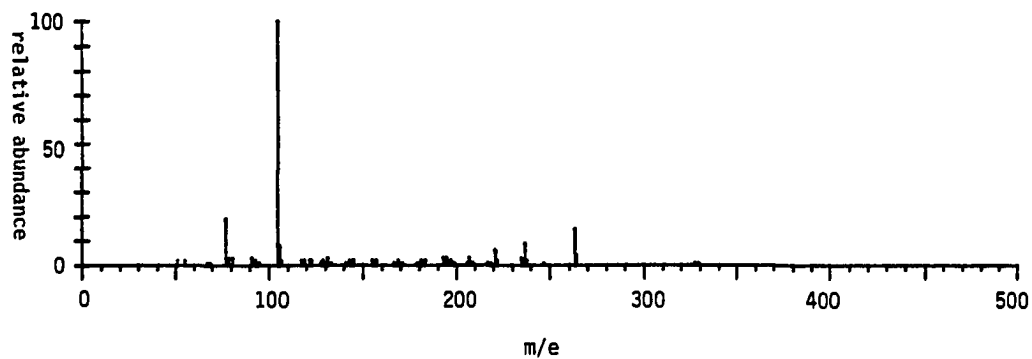
Mass Spectrum of 110b
