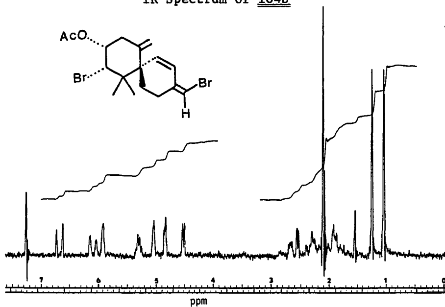
100 MHz PMR Spectrum of 104b in CDCl 3
