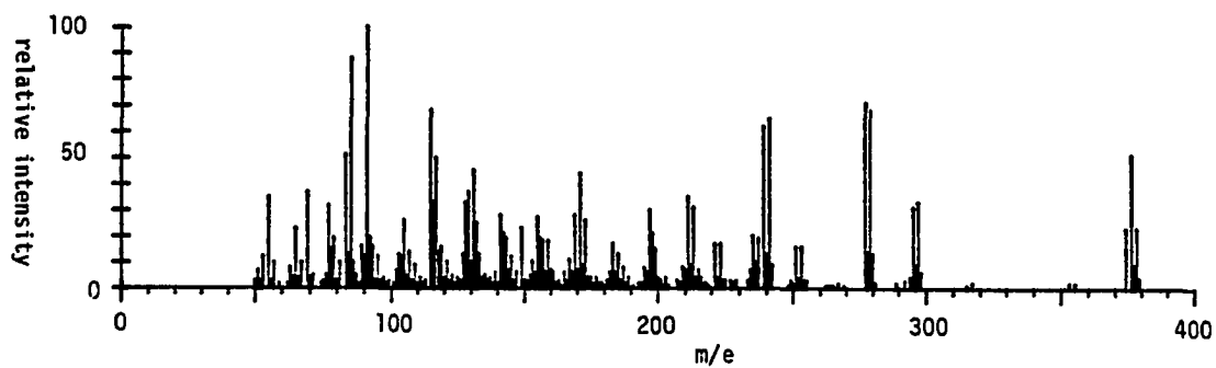
Mass Spectrum of 104a
