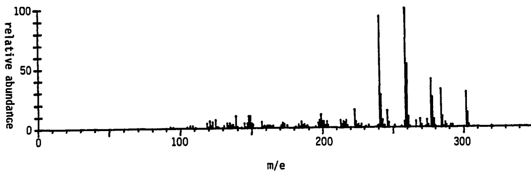
Mass Spectrum of 124
