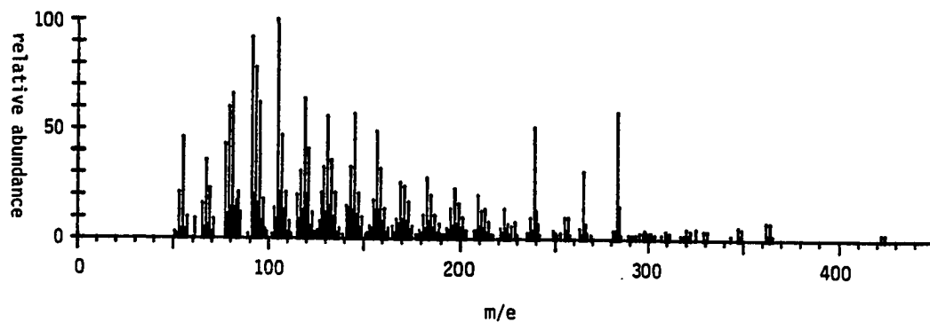
Mass Spectrum of 119
