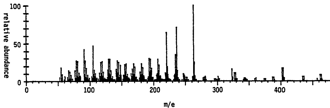
Mass Spectrum of 110a
