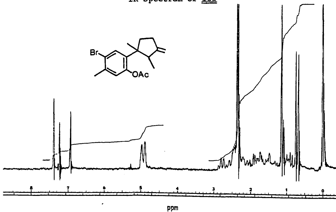
100 MHz PMR Spectrum of 101 in \text{CDCl}_3
