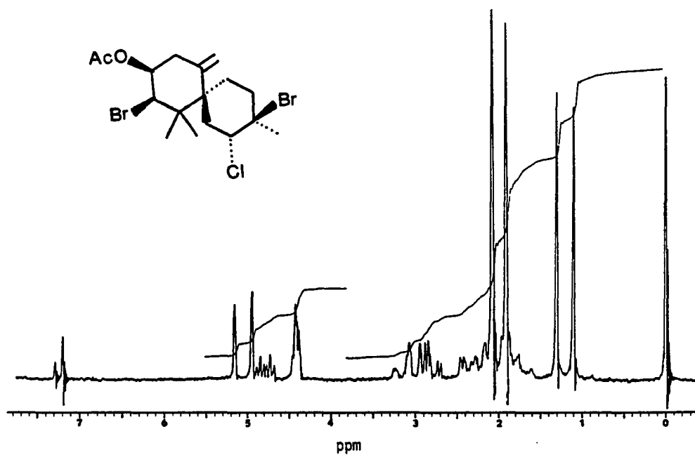
100 MHz PMR Spectrum of 108 in CDCl 3
