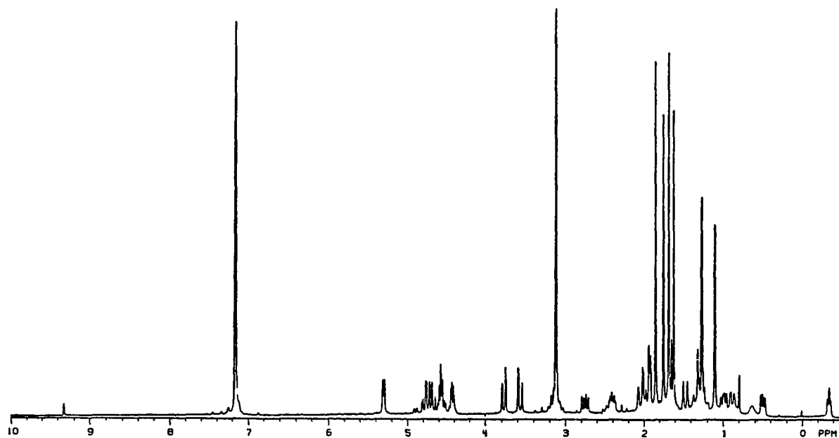
Figure 21. 270 MHz NMR Spectrum of 111 in Benzene-d 6
