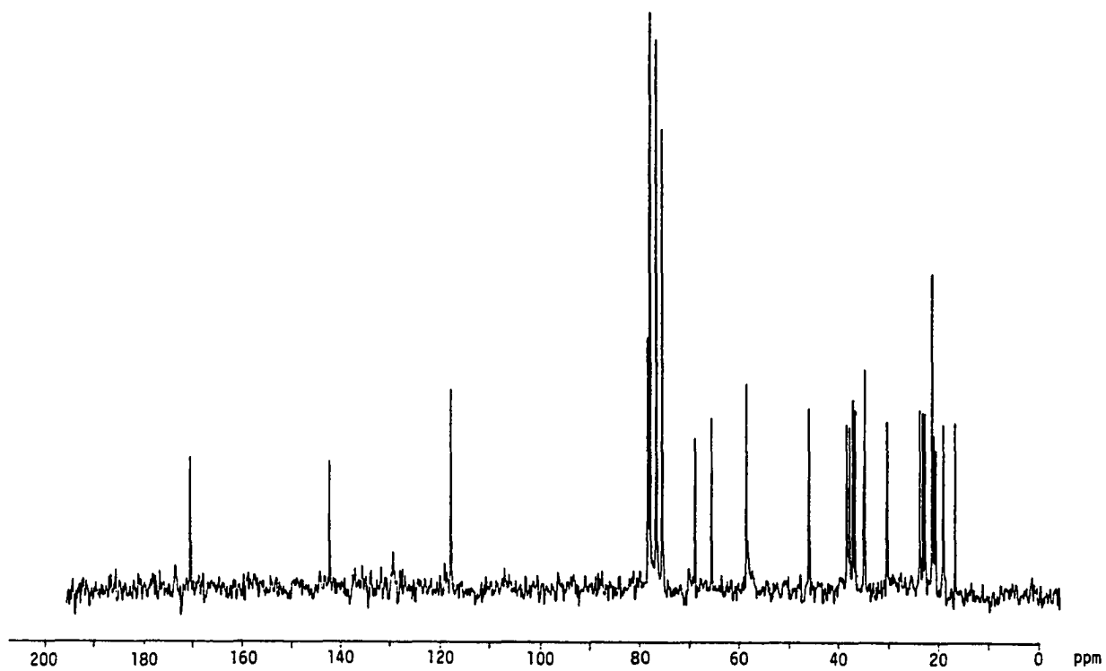
Figure 29. ^{13}\text{C} -NMR ( \text{CDCl}_3 ) Spectrum of Deoxyparguerol Acetate ( 120 ).
