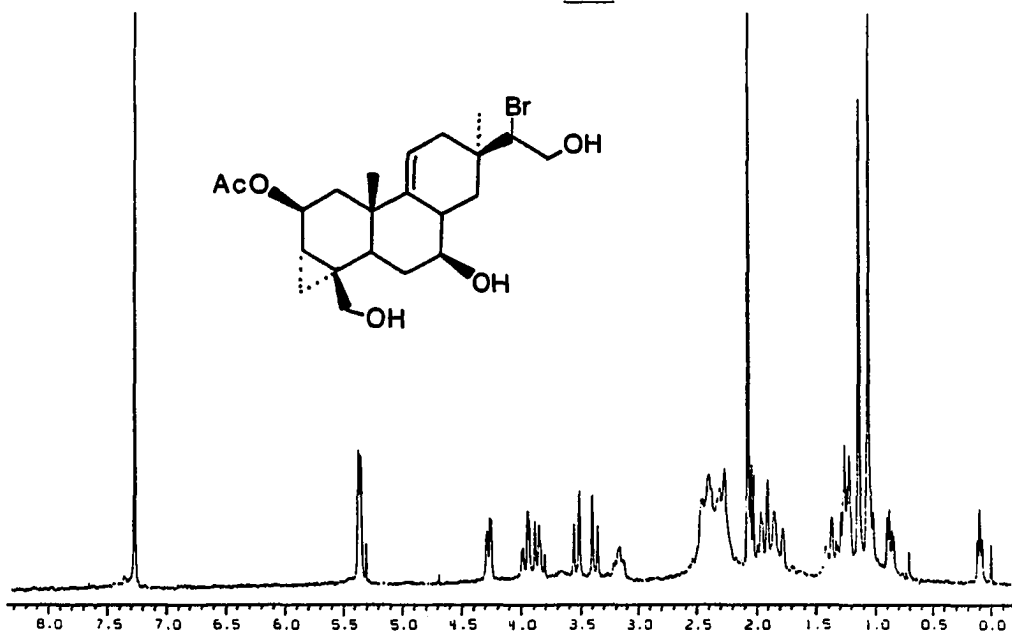
270 MHz PMR Spectrum of 109 in CDCl 3
