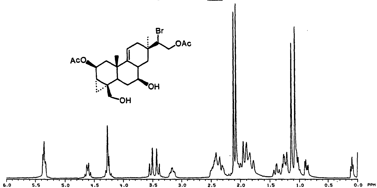
270 MHz PMR Spectrum of 118 in CDCl 3
