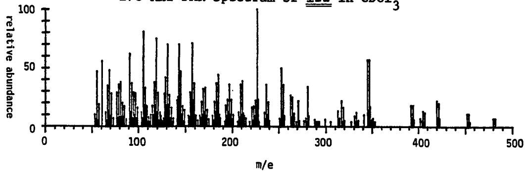
Mass Spectrum of 122
