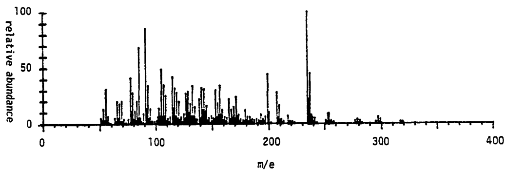
Mass Spectrum of 100
