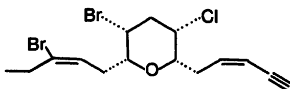
7 dactylyne
