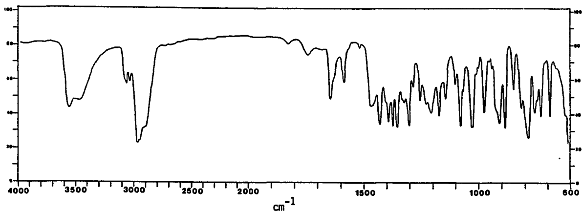
IR Spectrum of 105a
