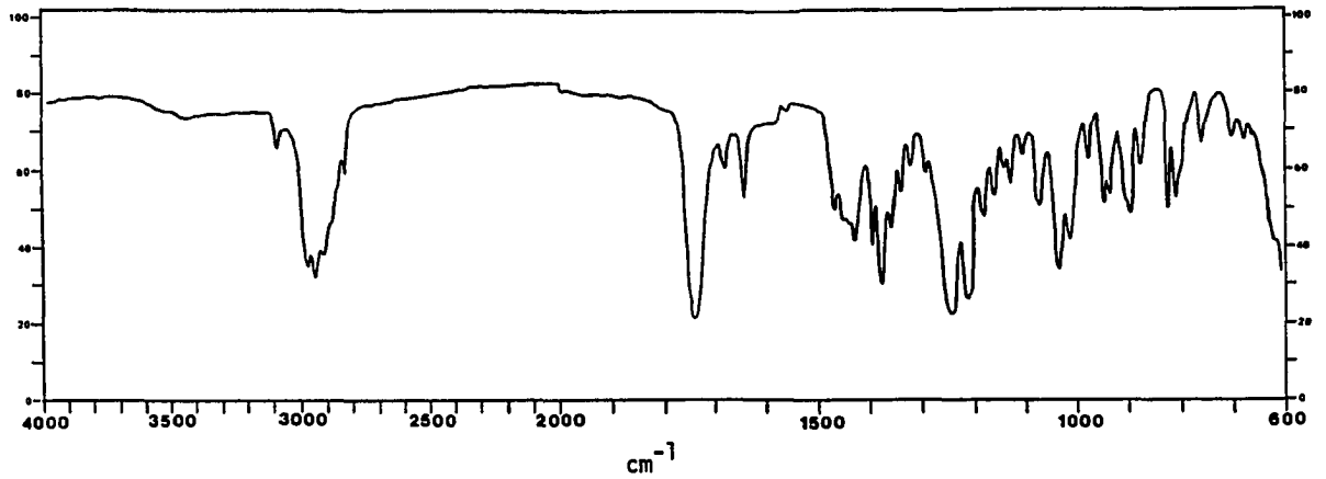
IR Spectrum of Elatol Acetate
