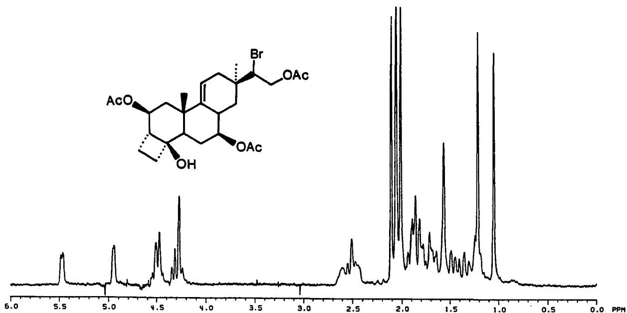
270 MHz PMR Spectrum of 122 in CDCl 3
