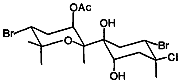
32 dihydroxydeodactol monoacetate
