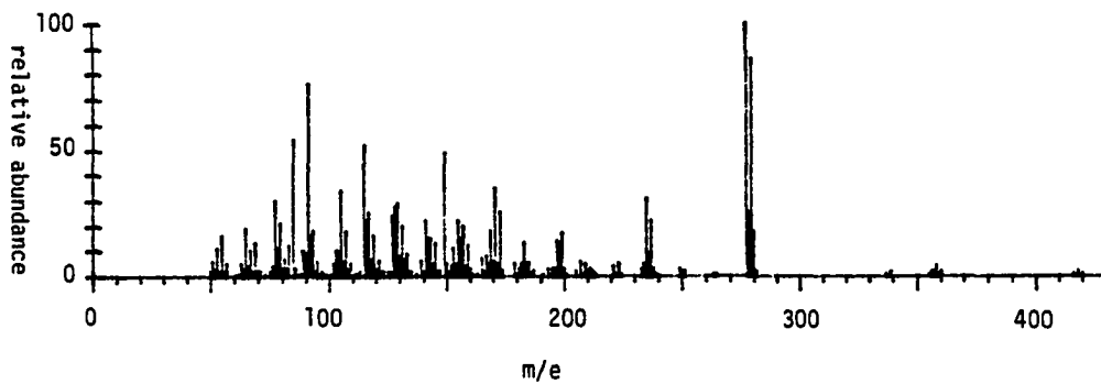
Mass Spectrum of 104b
