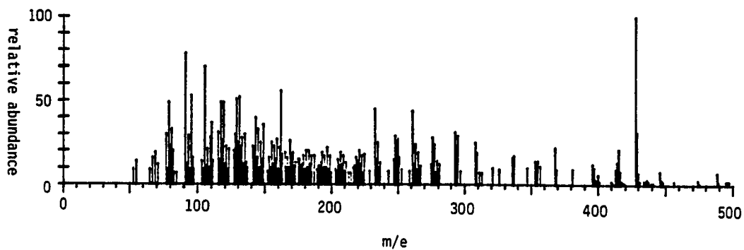
Mass Spectrum of 111
