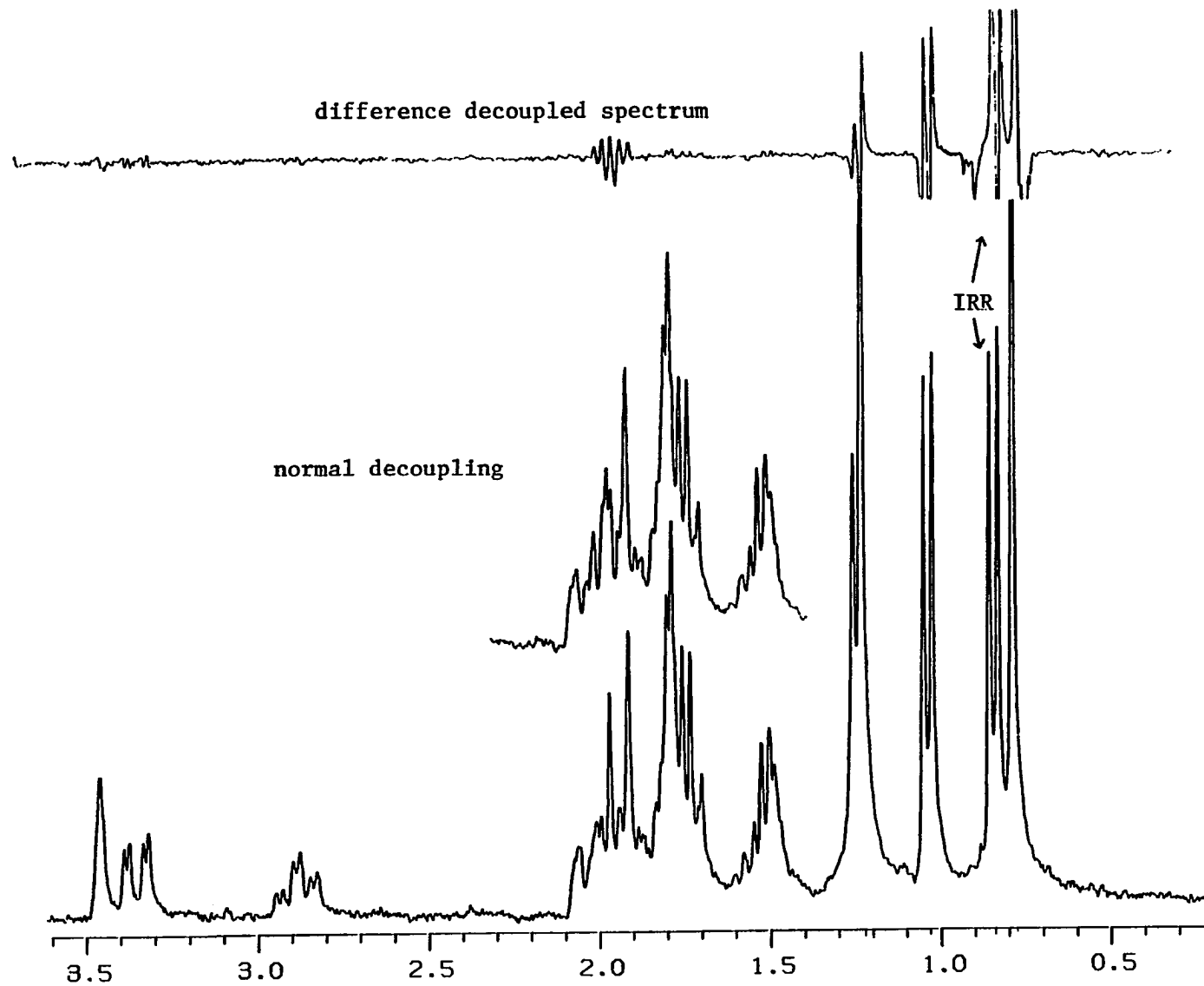
Figure 34. Difference Decoupled Spectrum of 124
