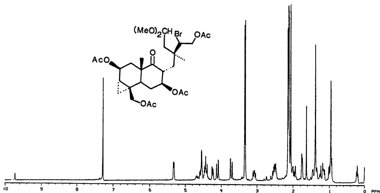
270 MHz PMR Spectrum of 111 in CDCl 3
