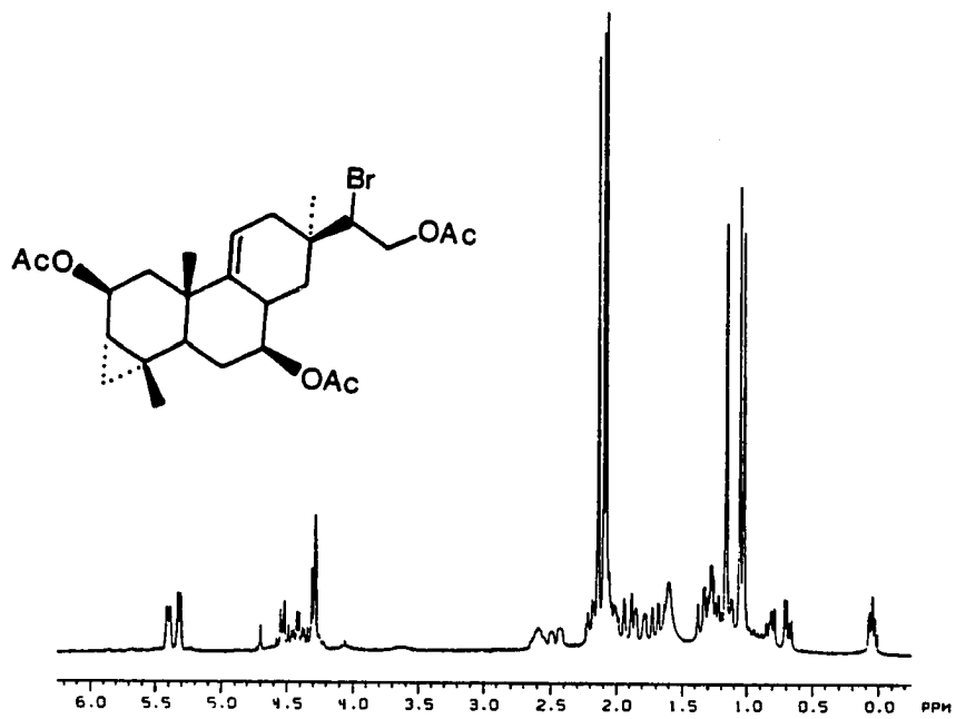
270 MHz PMR Spectrum of 120 in CDCl 3
