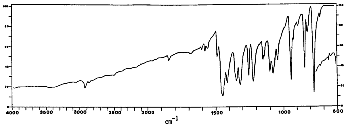
IR Spectrum of 99
