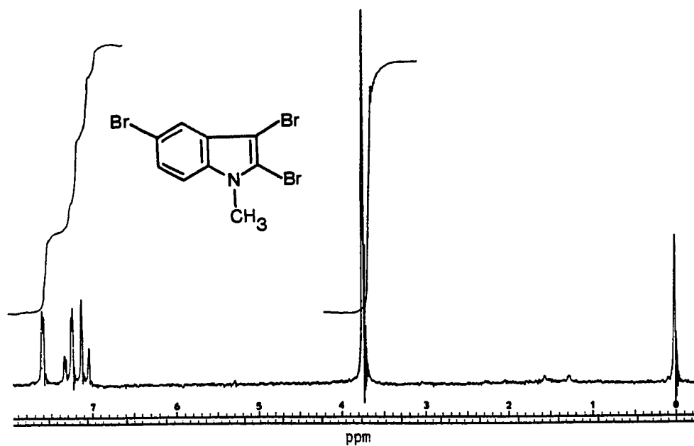
100 MHz PMR Spectrum of 99 in CDCl 3
