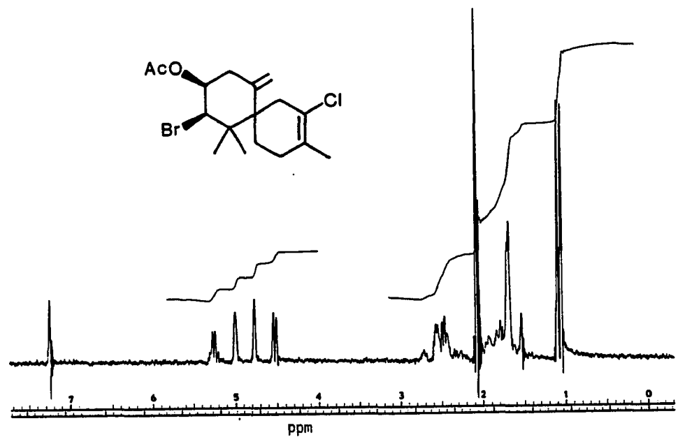
100 MHz PMR Spectrum of Elatol Acetate in \text{CDCl}_3
