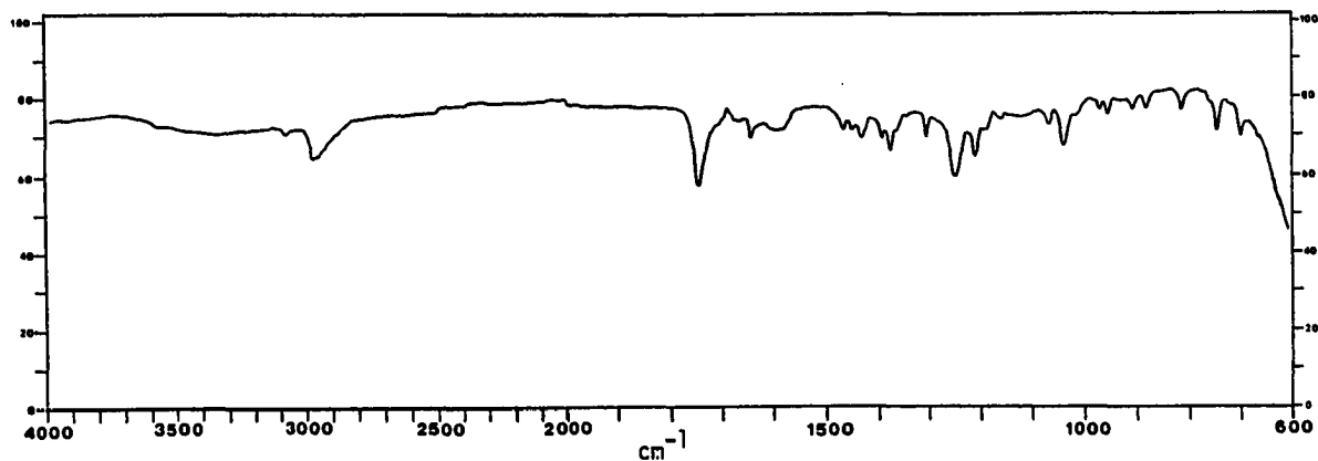
IR Spectrum of 104b
