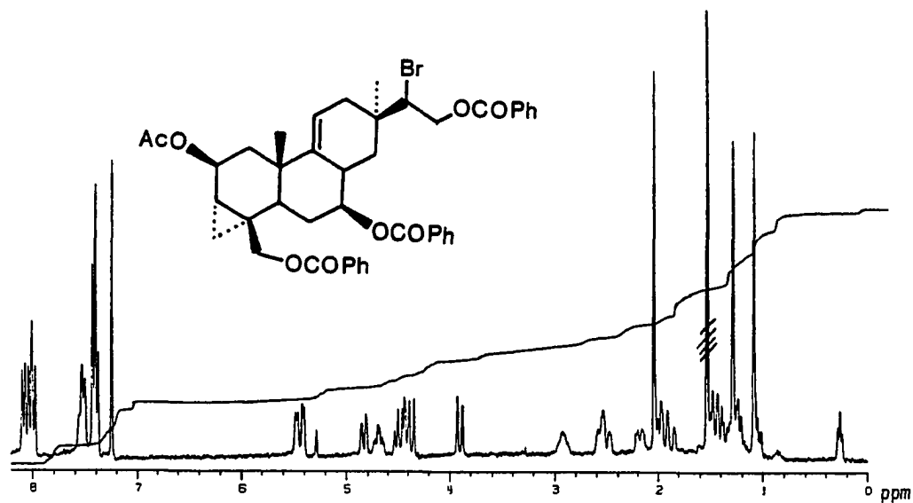
270 MHz PMR Spectrum of 110b in CDCl 3
