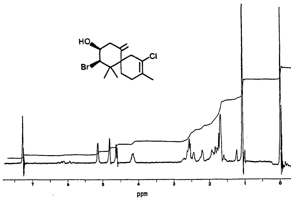
100 MHz PMR Spectrum of 100 in CDCl 3
