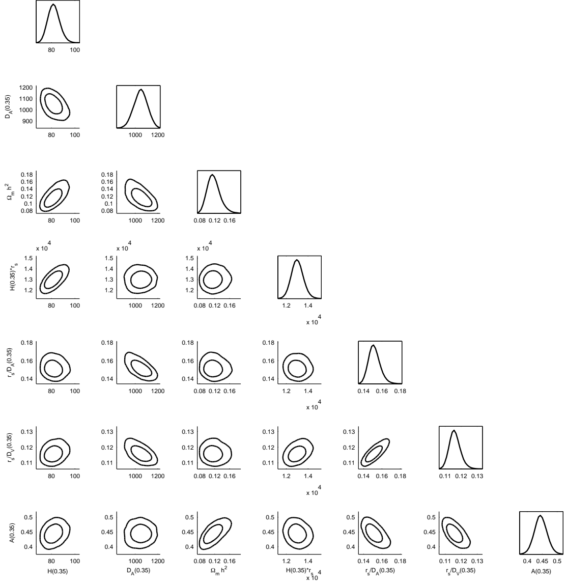
Figure 4.3: 2D marginalized contours (68% and 95% C.L.) for \{H(0.35), D_A(0.35), \Omega_m h^2, H(0.35) r_s(z_d), r_s(z_d)/D_A(0.35), r_s(z_d)/D_V(0.35), A(0.35)\} . The diagonal panels represent the marginalized probabilities. The unit of H is \text{km s}^{-1} \text{Mpc}^{-1} . The unit of D_A , D_V , and r_s(z_d) is Mpc.
