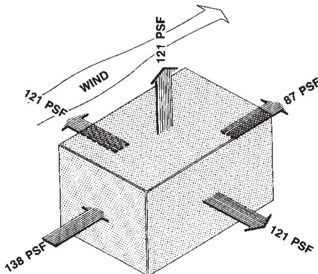
Figure 1. Pressure forces created by 240 mph wind.
