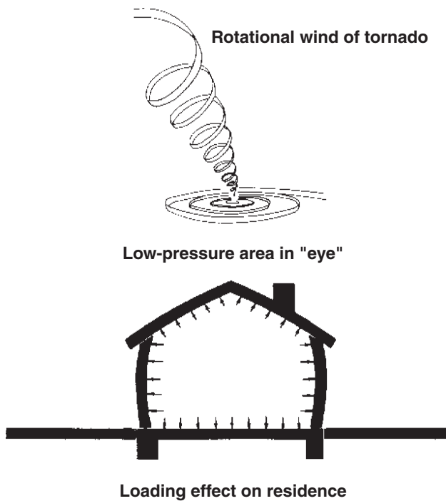
Figure 2. Pressure forces created by sudden pressure drop.
