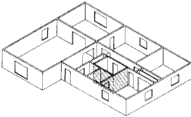
Figure 4. Tornado shelter built within the home.
