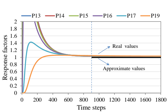
Figure 6 The the real and approximate response factors of P13~P19
