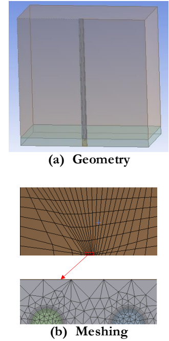
Figure 3 The studied case in ANSYS
