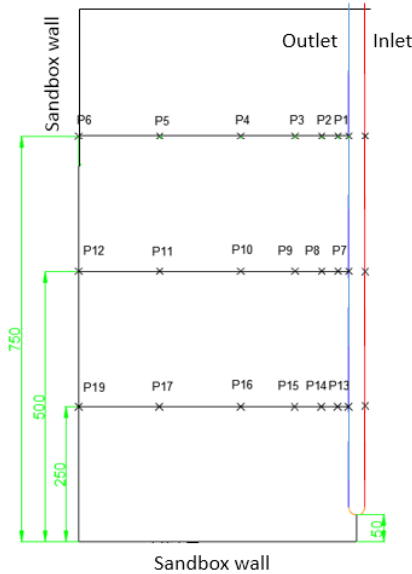
Figure 2 Side view of thermocouples placement within sandbox
