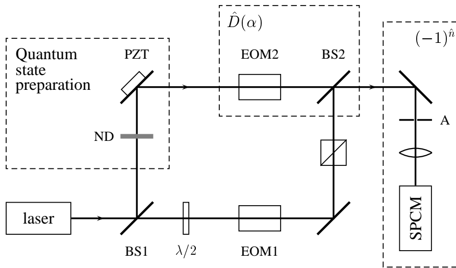
Fig. 1. The experimental setup for measuring the Wigner function of a single light mode. BS1 and BS2 are quartz plates serving as high-transmission beam splitters. The quantum state to be measured is prepared using the neutral density filter ND and the mirror mounted on a piezoelectric translator PZT. The electrooptics modulators EOM1 and EOM2 define the amplitude and the phase of the displacement \hat{D}(\alpha) . The quantum state, after applying the displacement transformation, is detected with the single photon counting module SPCM.
