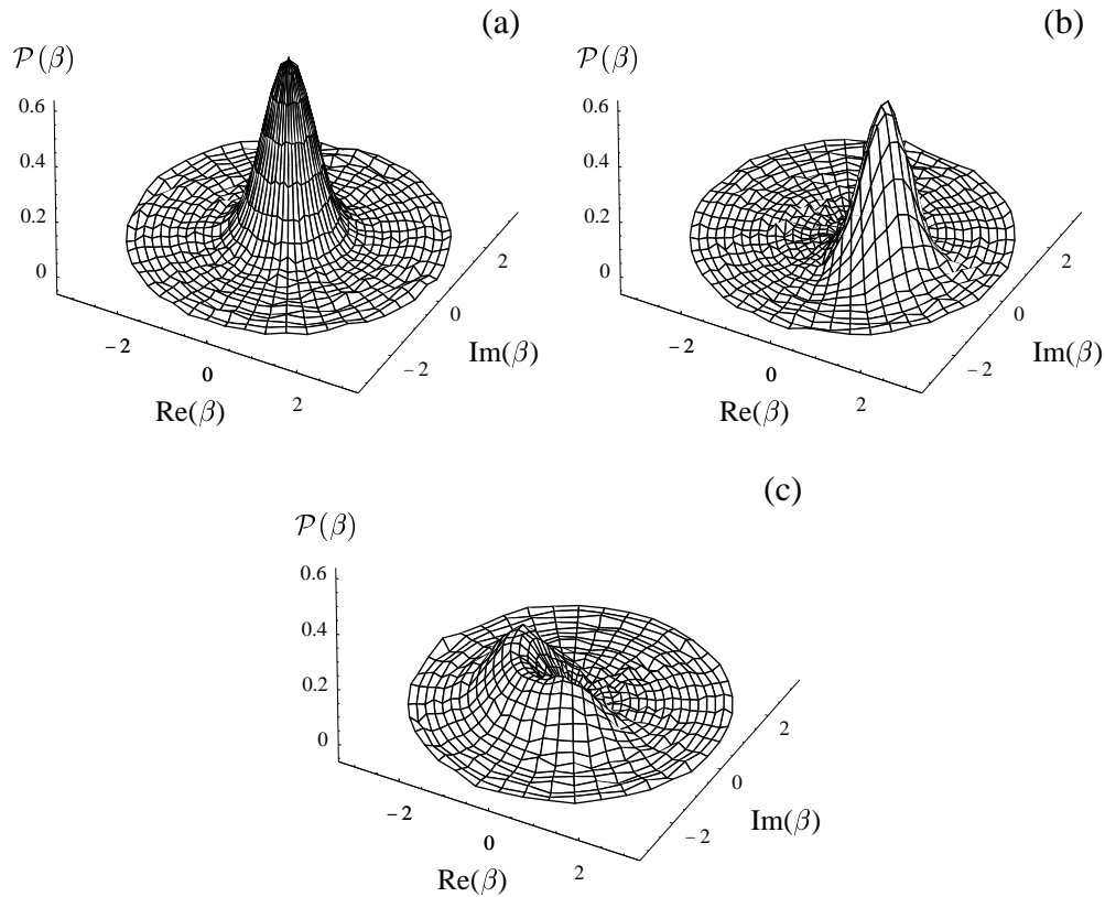
Fig. 2. The measured Wigner functions for (a) the vacuum, (b) a weak coherent state with approximately one photon, and (c) a phase diffused coherent state. The photon statistics was collected on a polar grid spanned by 20 amplitudes, and 50 phases for the plots (a) and (b), or 40 phases for the plot (c). The duration of a single counting interval was 40 \mu\text{s} for (a) and (b) and 30 \mu\text{s} for (c). The measurements were performed for slightly different laser intensity, and the radial coordinate for each of the graphs was scaled separately.
