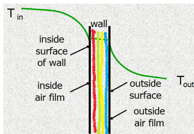
Figure 1. Diagram showing wall insulation sandwich of different materials with temperature inside ( T_{in} ) and temperature outside ( T_{out} ) on a cold day.
