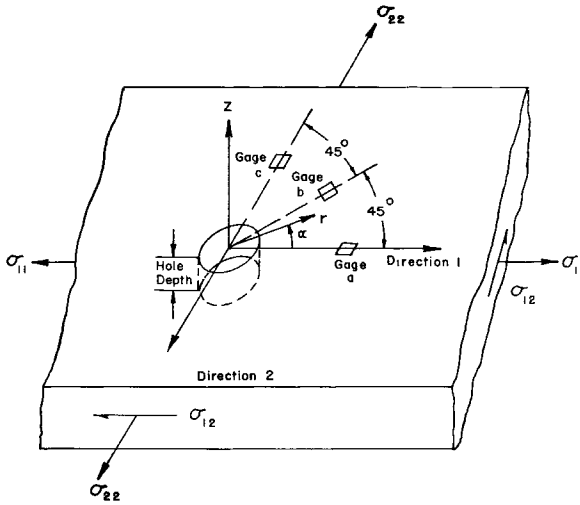
Figure 1. Schematic diagram showing coordinate system, stress components, hole geometry, and strain-gage locations.
