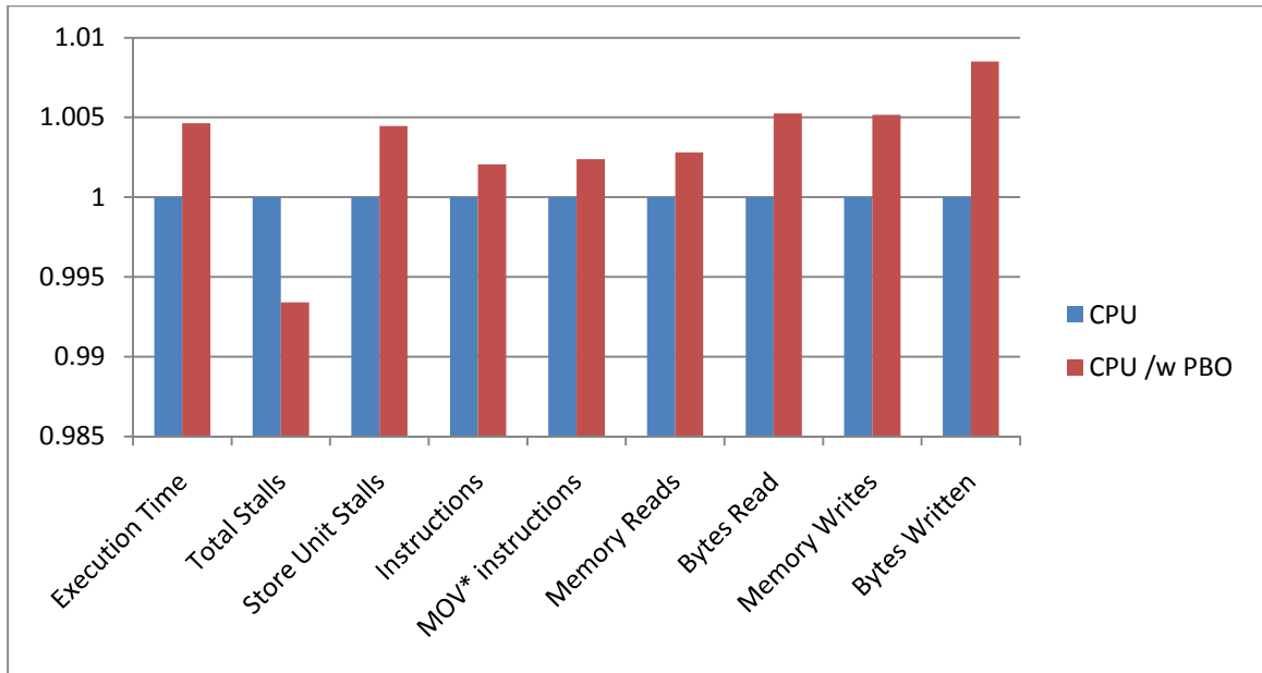
Figure 5.11 – Normalized Comparison of Program Characteristics. There is very little difference between these two programs despite using different means of transferring the pixel data to system memory. Based on this, the program that used a PBO, and subsequently DMA transfers, and the program that did not use a PBO behaved almost identically.
