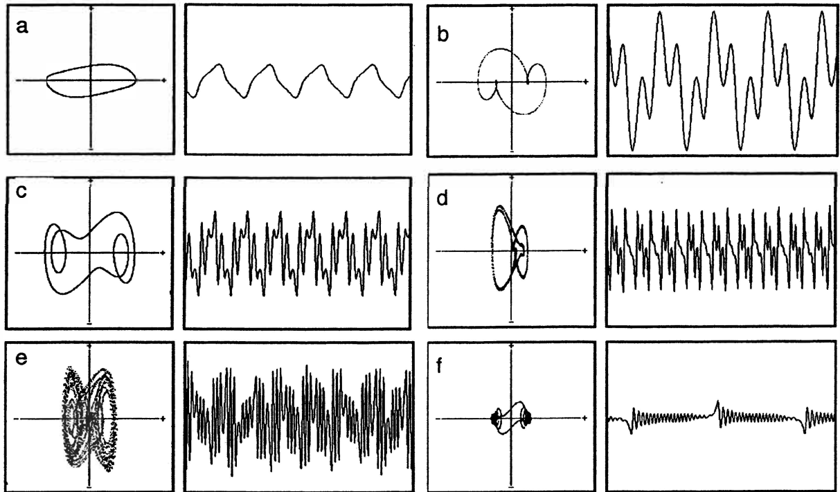
figure 2 - period doubling progression in the cubic oscillator
