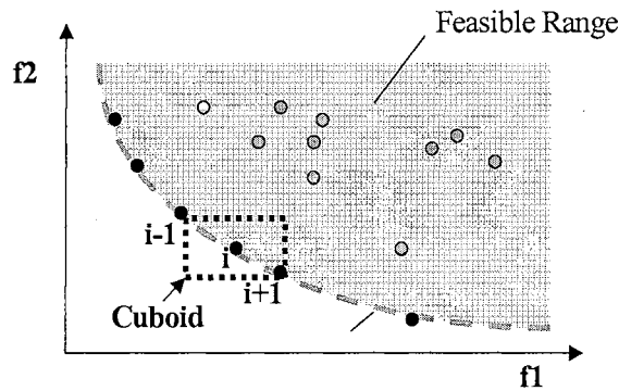
Figure 4.7 Illustration of crowding distance estimation approach
