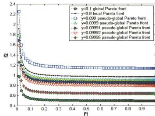
Figure 6.11 Pseudo-global Pareto fronts when x_2 approaches to x_{2\text{ global}} = 0.1 ( q_2 / q_1 = 10,000 ) ratio
