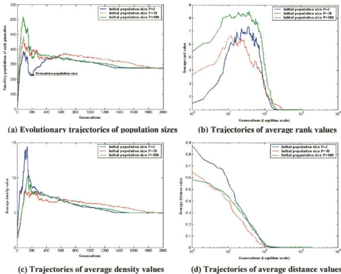
Figure 7.10 Evolutionary trajectories for the population size and the values of three indicators resulting by DMOEA with three different initial population sizes ( A_{th}=10 ) on Function F5
