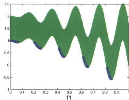
(b) Pareto front of function F5
