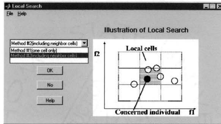
Figure 8.14 GUI of local search setting
