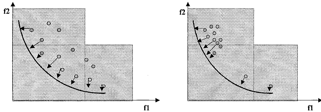
(a) Population diversity is preserved (b) Population diversity is not preserved Figure 4.5 Illustration of the effect of population diversity preservation
