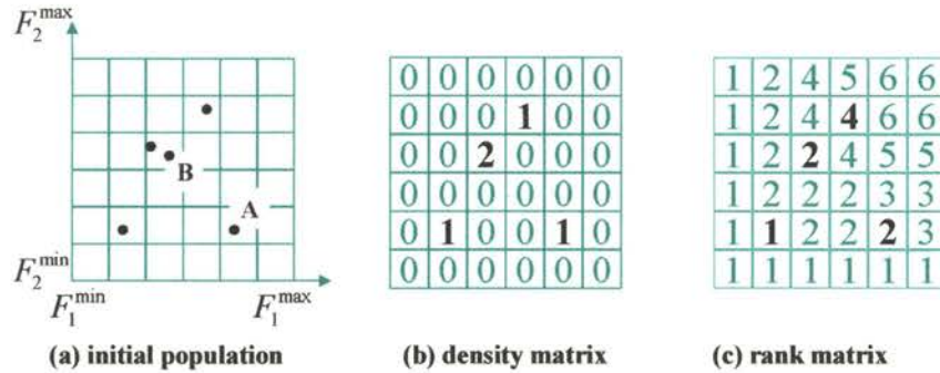
Figure 7.2 Initial population and its corresponding density and rank matrices
