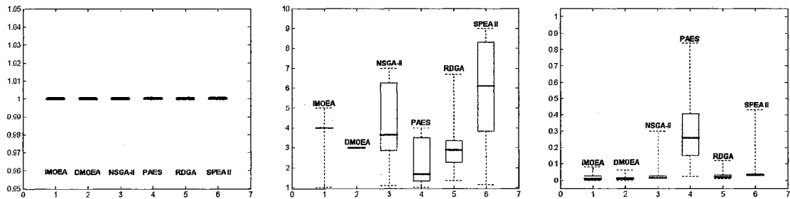
(a) Average individual rank value (b) Average individual density value (c) Average individual distance value Figure 7.17 Box plots of average individual rank, density and distance values on Function F3
