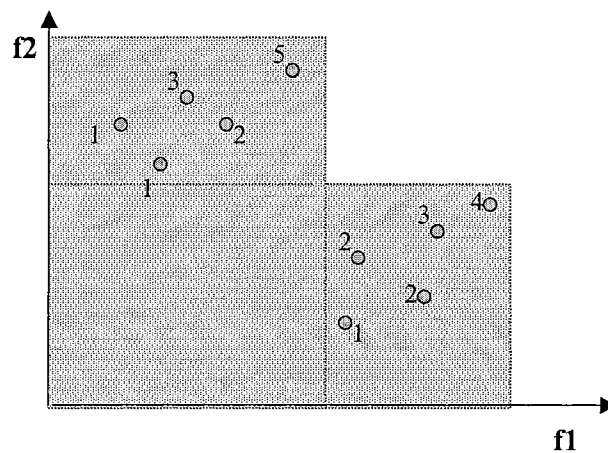
Figure 4.3 Illustration of Fonseca’s Pareto-based ranking scheme
