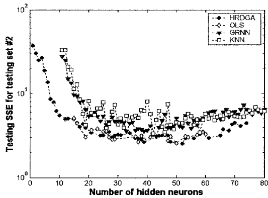
(a) Testing performances
