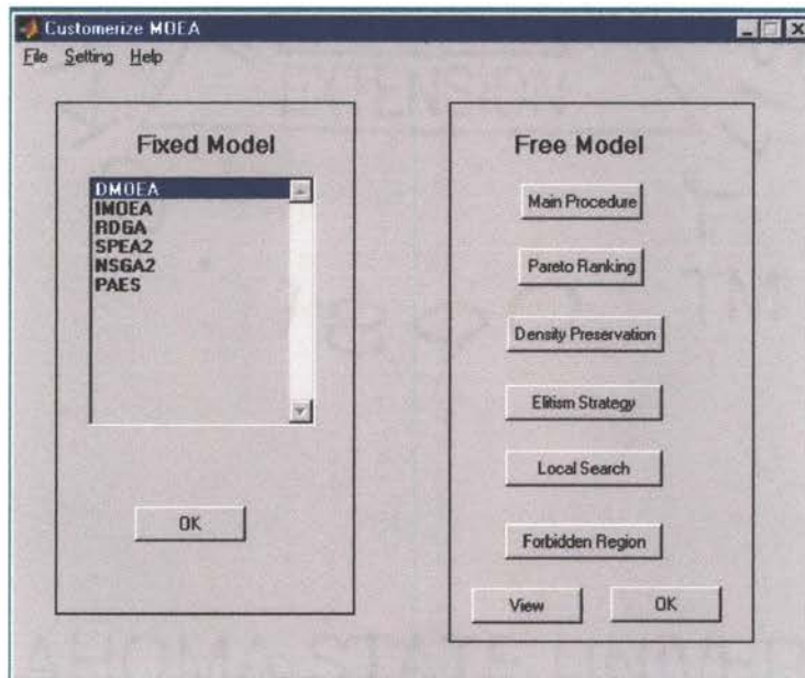
Figure 8.3 GUI of model selection
