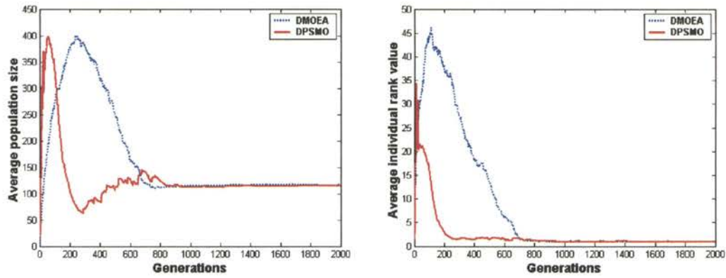
(a) Evolutionary trajectories of population sizes
