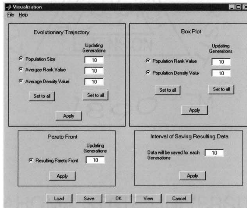
Figure 8.17 GUI of visualization setting
