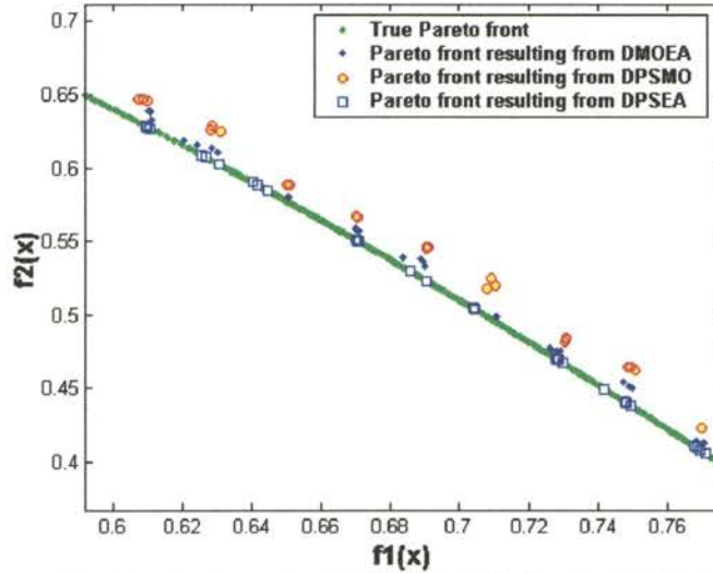
Figure 9.3 Resulting Pareto fronts by DMOEA, DPSMO and DPSEA on Function F3
