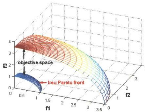
Figure 7.19 Objective space and Pareto front of Function F_6
