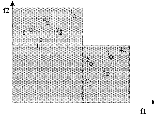
Figure 4.2 Illustration of Goldberg's Pareto-based ranking scheme
