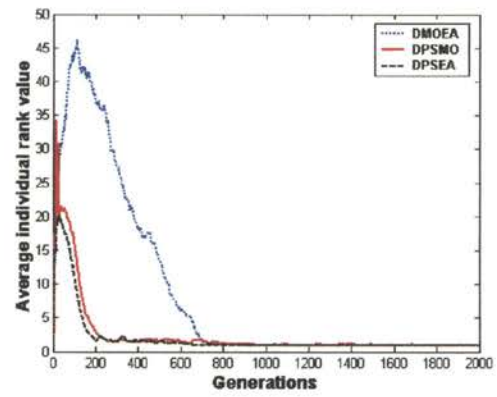
(b) Trajectories of average rank values
