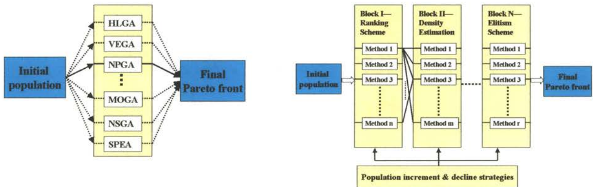
(a) Skeleton of MOEA Toolbox designed by Tan (b) Skeleton of envisioned MOEA Toolbox
