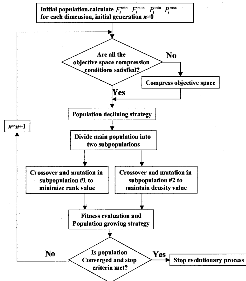
Figure 7.8 Flow chart of DMOEA
