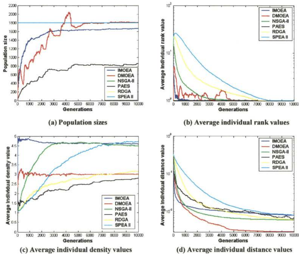
Figure 7.23 Evolutionary trajectories of population sizes and average individual rank, density and distance values from six selected MOEAs over 50 runs on Function F_6
