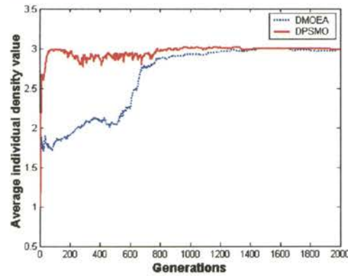
(c) Trajectories of average density value
