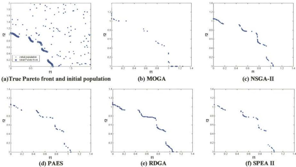
Figure 6.3 True Pareto front and Pareto fronts resulted by MOGA, NSGA-II, PAES, RDGA and SPEA II on Function F1
