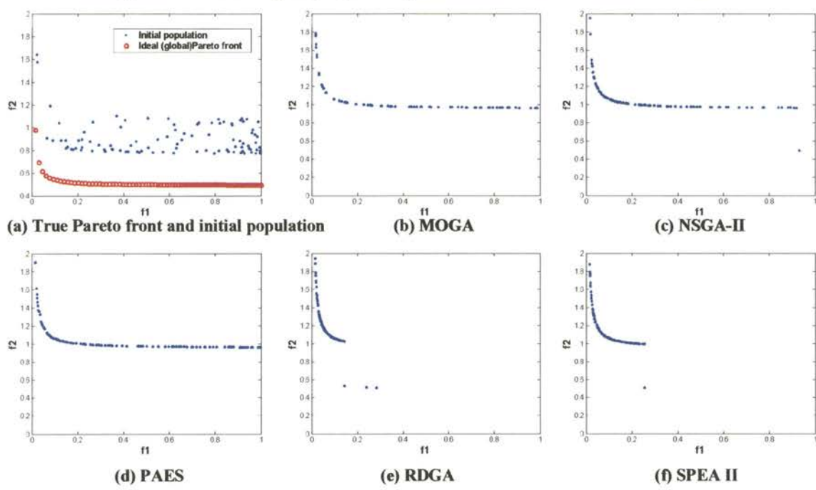
Figure 6.7 True Pareto front Pareto fronts resulted by MOGA, NSGA-II, PAES, RDGA and SPEA II on Function F2-1
