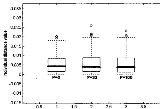
(a) Box plots for population rank values (b) Box plots for population density values (c) Box plots for population distance values Figure 7.11 Box plots of three indicators with three different initial population sizes ( A_{th} = 10 ) on Function F5
