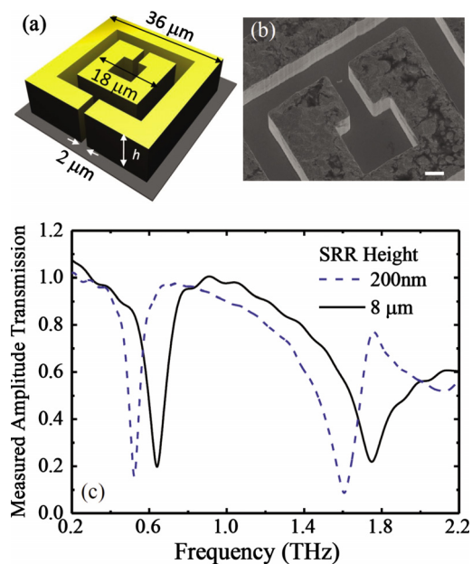
FIG. 1. (Color online) (a) Schematic diagram of a SRR illustrating the dimensions used in this study and the SRR height parameter ( h ), (b) electron micrograph of high aspect ratio SRR with h=8\ \mu\text{m} (scale bar= 2\ \mu\text{m} ), and (c) measured THz spectra for SRRs of different heights.
