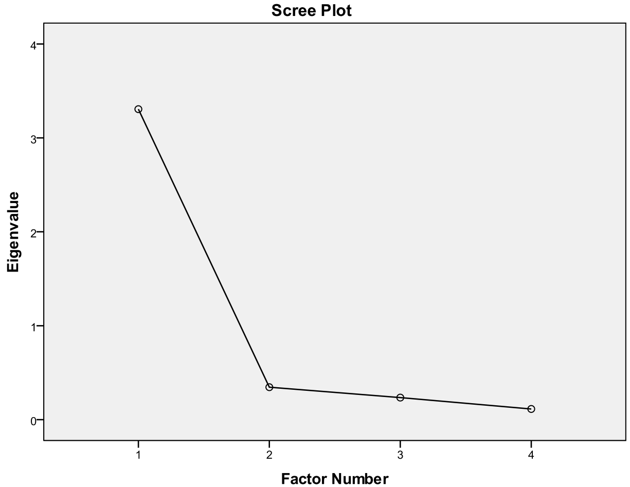
Scree Plot
