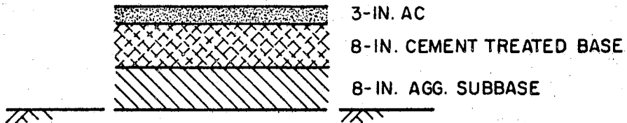
Figure 2.11. A Current Pavement Design in Arizona
