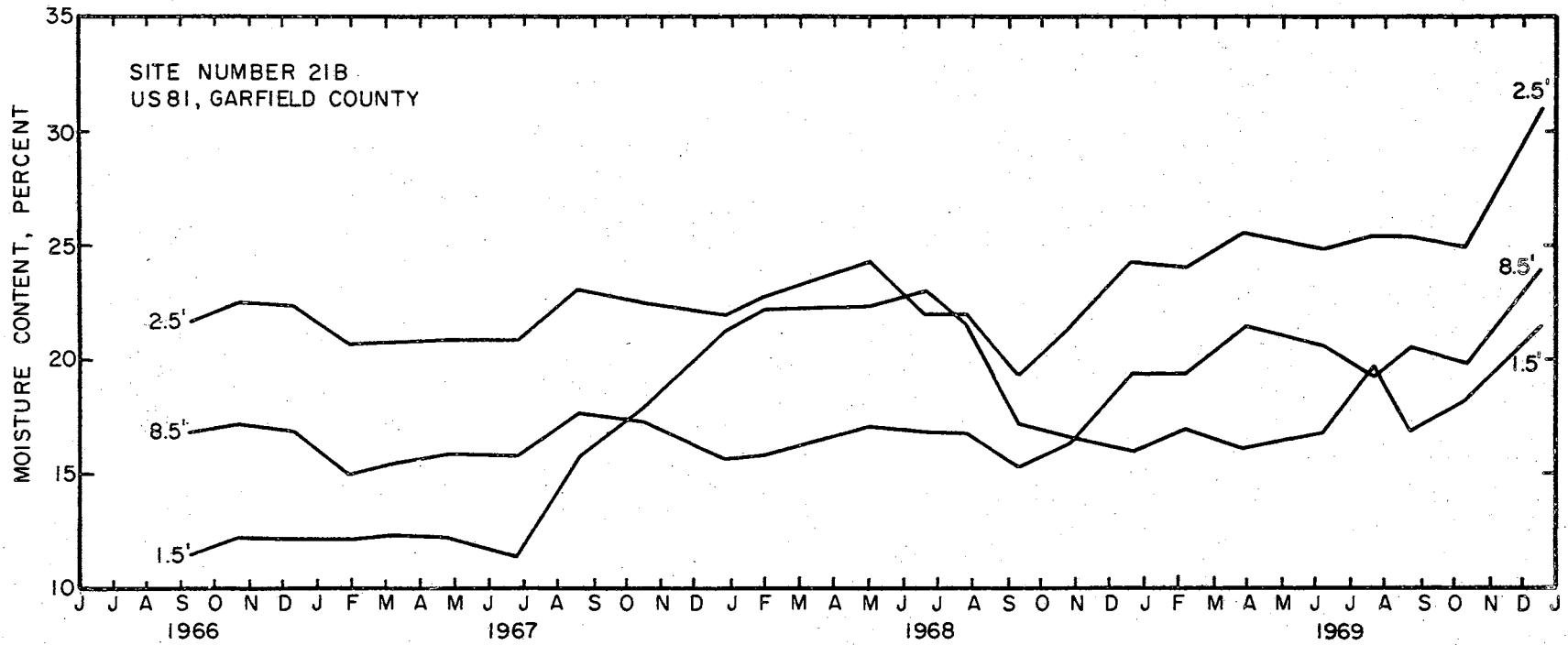
Figure 3.4. Moisture Variations at Selected Levels Beneath Pavement Centerline at Site No. 21
