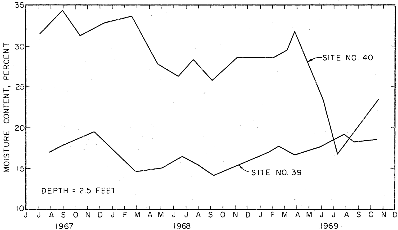
Figure 3.5. Moisture Variations at Depth of 2.5 feet Beneath Pavement Centerline for Sites No. 39 and 40
