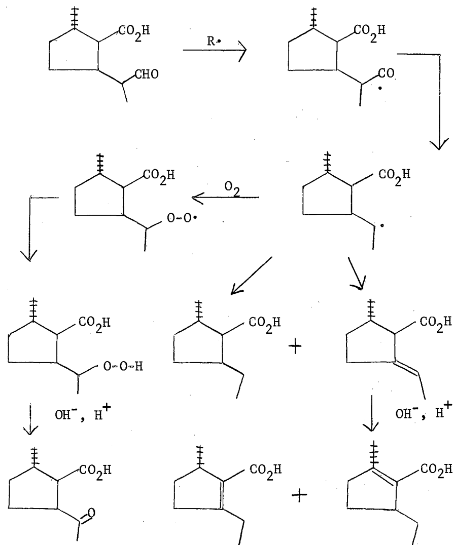
Figure 3. Proposed Radical Mechanism for Formation of Nepetonic Acids
