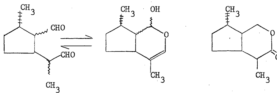
Iridodial
