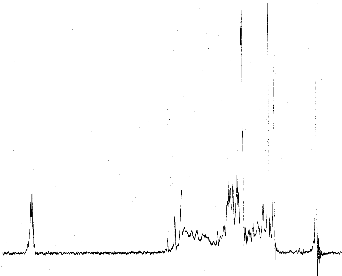
Figure 7. Nmr Spectrum of cis , cis -Nepetalactone, 1d
