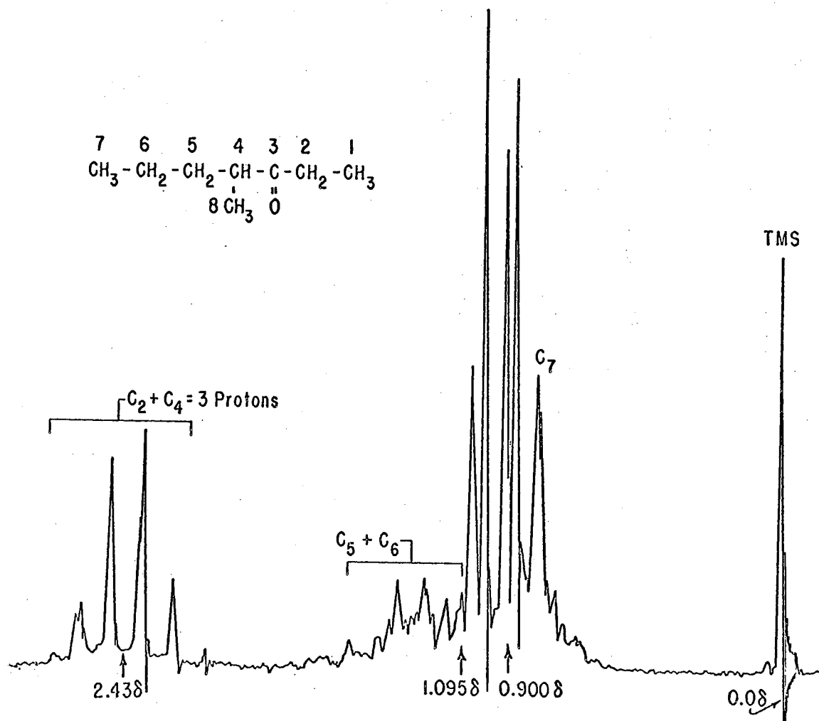
Figure 2. Nmr Spectrum of 4-Methyl-3-heptanone
