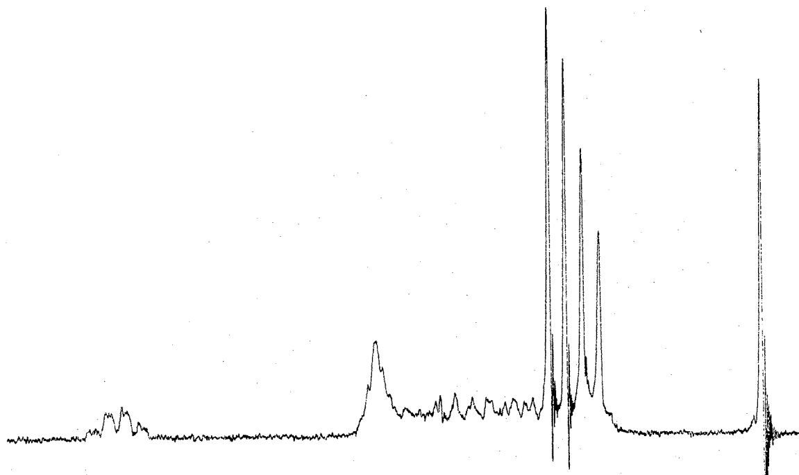
Figure 10. Nmr spectrum of 3R- dis , trans -Nepetolactone, 3a
