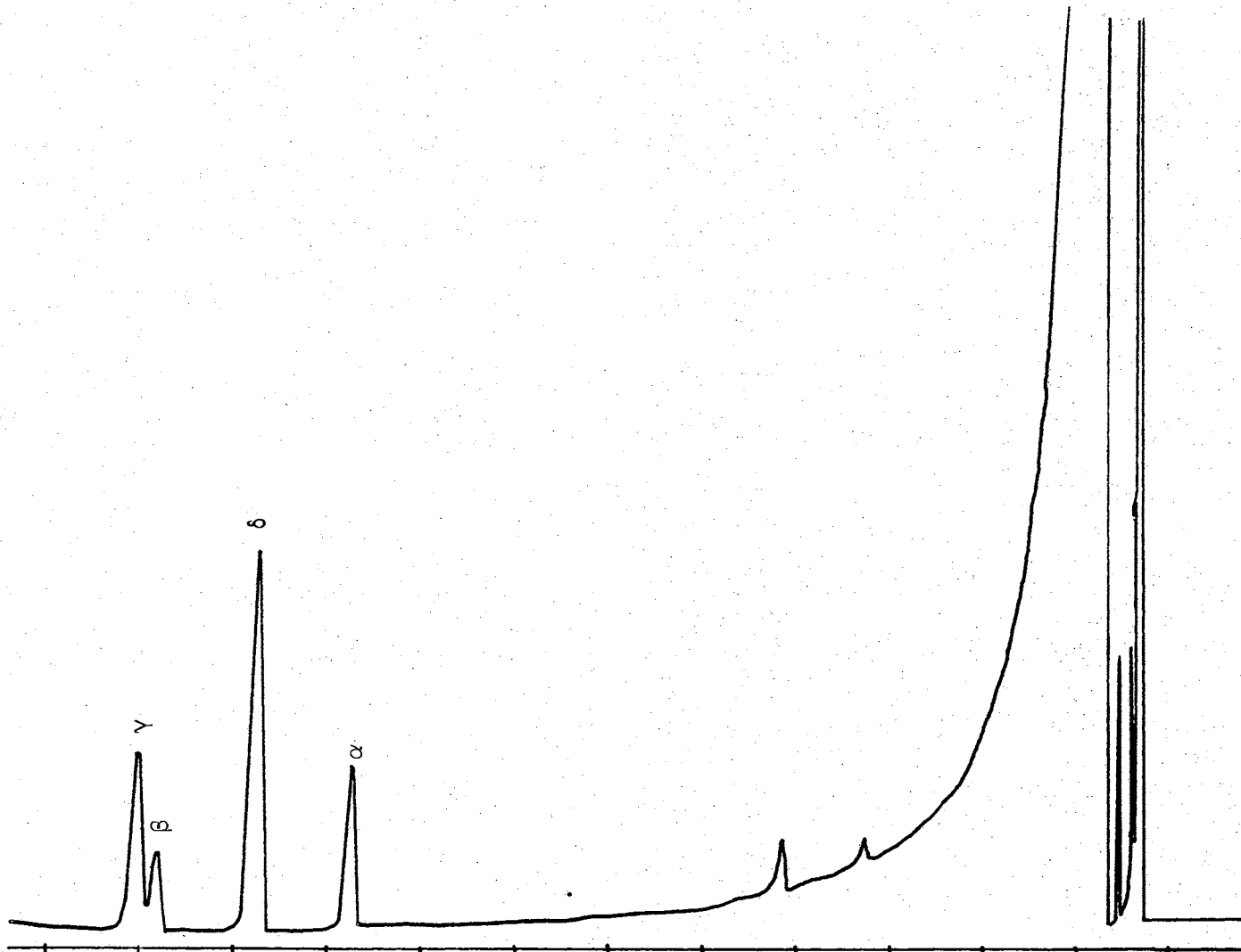
Figure 9. Gas Chromatogram of Standard Iridodiols
