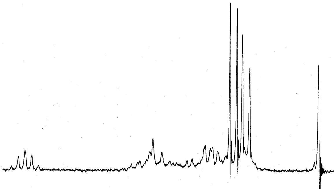
Figure 11. Nmr Spectrum of 3S- cis , trans -Nepetolactone, 3b
