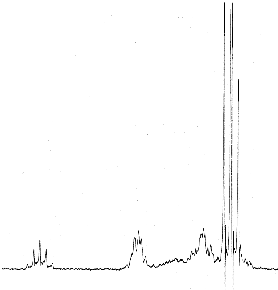
Figure 13. Nmr Spectrum of 3R- cis , cis -Nepetolactone, 3d
