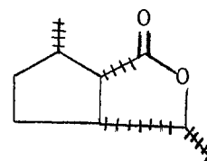
C-4 3d
