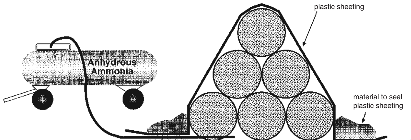
Figure 2. Using anhydrous ammonia with the sheeting covering hay.
