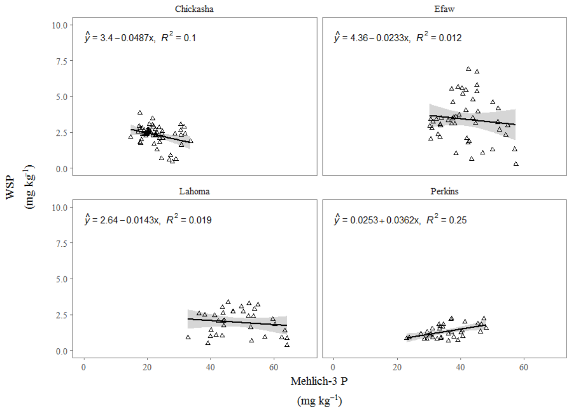
Figure 2.12. Water soluble phosphorus (WSP) as a function of Mehlich-3 phosphorus (M3-P) in soils collected from Chickasha, Efaw, Lahoma, and Perkins. WSP and M3P values are reported in mg kg -1 .
