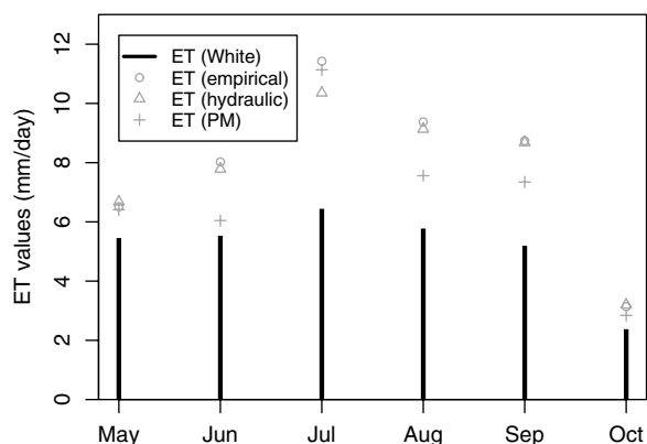
Figure 9 Daily mean ET rates by month of the original White approach and Penman–Monteith (PM) method, as well as of the empirical and hydraulic versions of the present ET estimation method for the 2005 growing season.
