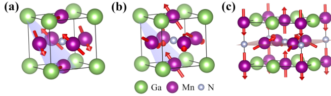
FIG. 1. Different noncollinear magnetic phases in AFM antiperovskite GaNMn 3 : (a) \Gamma_{5g} , (b) \Gamma_{4g} , and (c) M-1. Red arrows denote magnetic moments.
