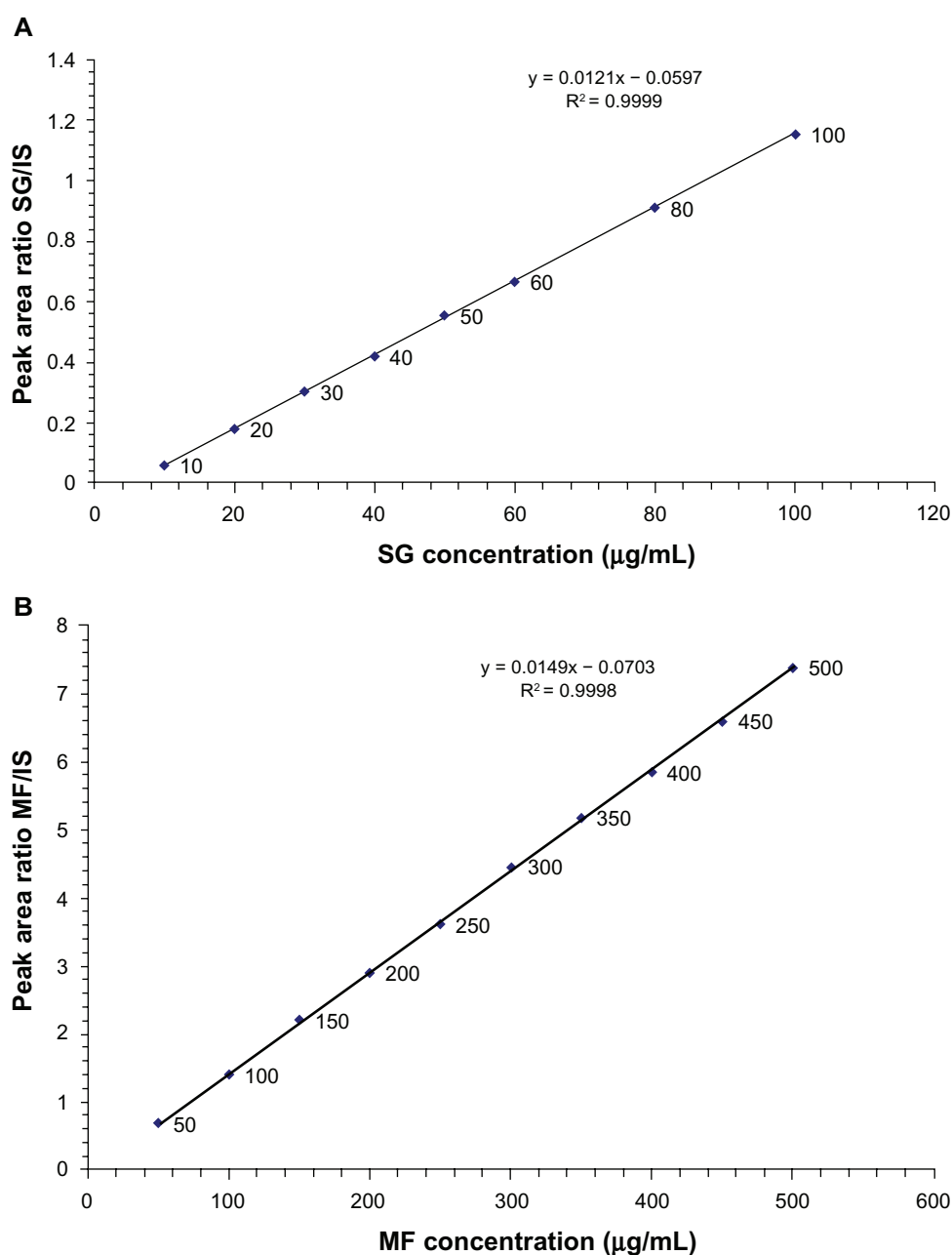
Figure 6. Calibration curve for the determination of (A) SG, (B) MF by the proposed CZE method under the described electrophoretic conditions.
