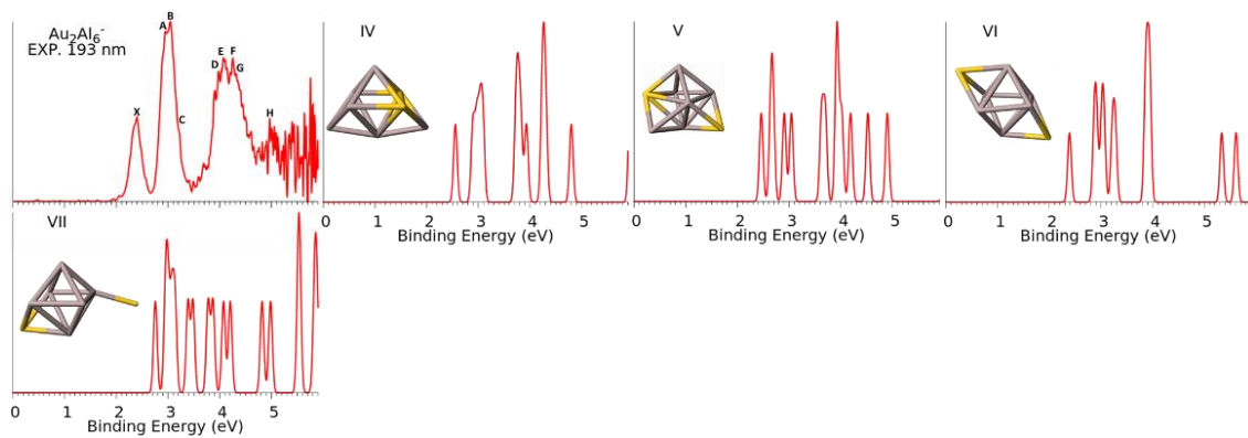
Figure S5. Comparison of the simulated spectra for the isomers IV to VII of \text{Au}_2\text{Al}_6^- with the 193 nm experimental spectra.
