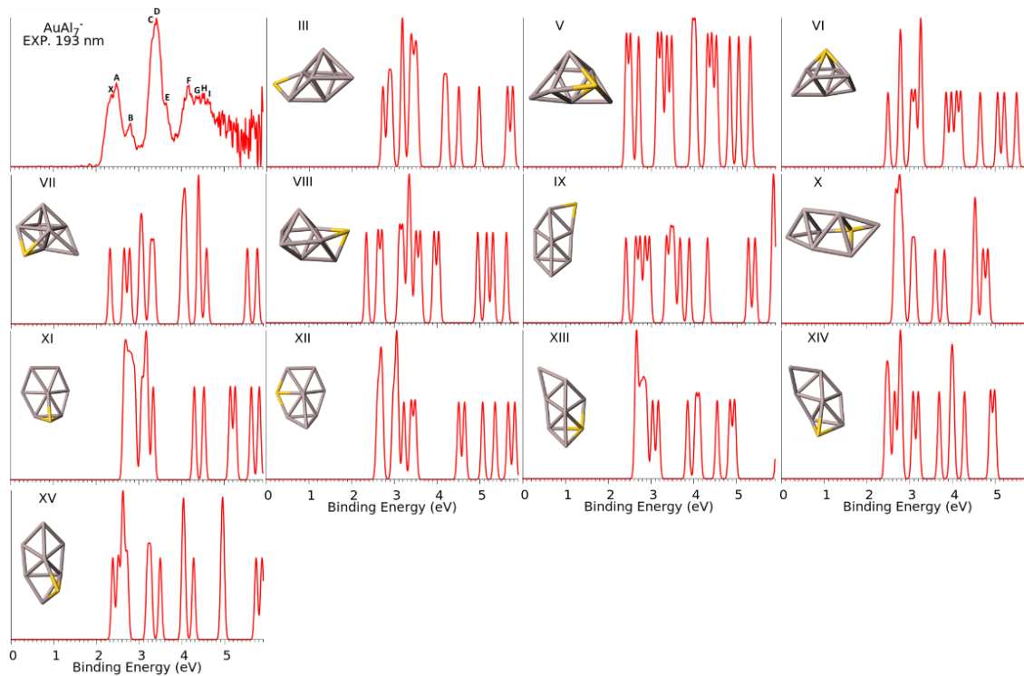
Figure S4. Comparison of the simulated spectra for the isomers III and V to XV of \text{AuAl}_7^- with the 193 nm experimental spectra.
