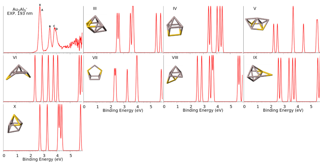
Figure S2. Comparison of the simulated spectra for the isomers III to X of \text{Au}_2\text{Al}_5^- with the 193 nm experimental spectra.
