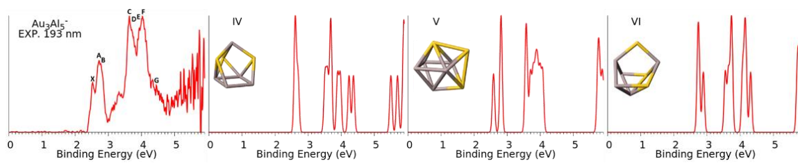
Figure S6. Comparison of the simulated spectra for the isomers IV to VI of \text{Au}_3\text{Al}_5^- with the 193 nm experimental spectra
