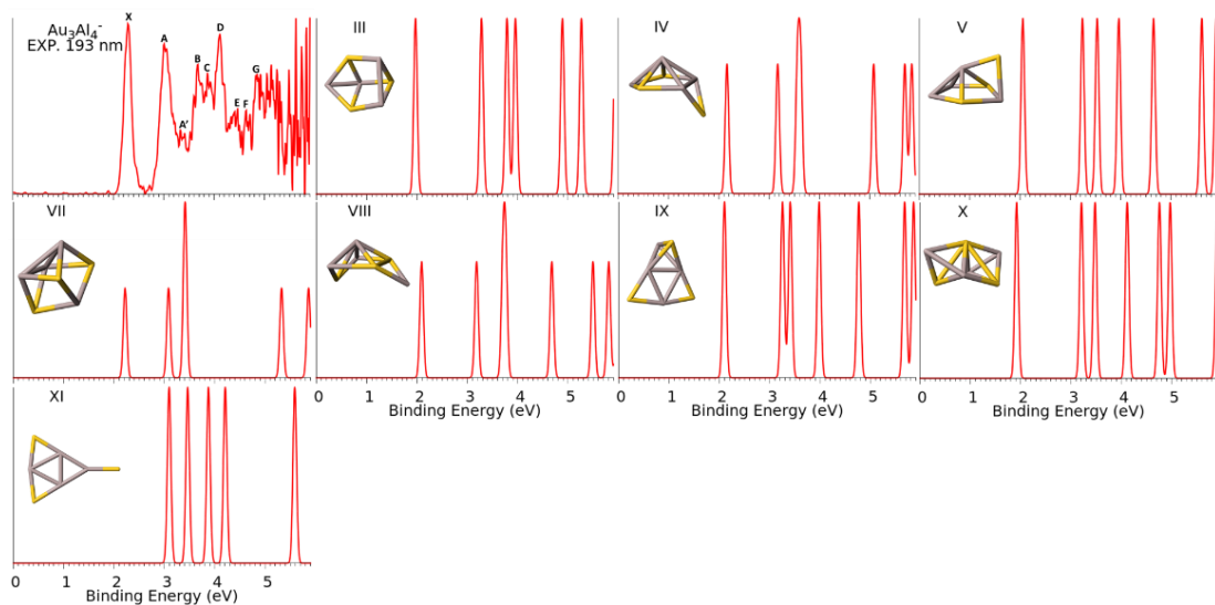
Figure S3. Comparison of the simulated spectra for the isomers III to V and VII to XI of \text{Au}_3\text{Al}_4^- with the 193 nm experimental spectra.
