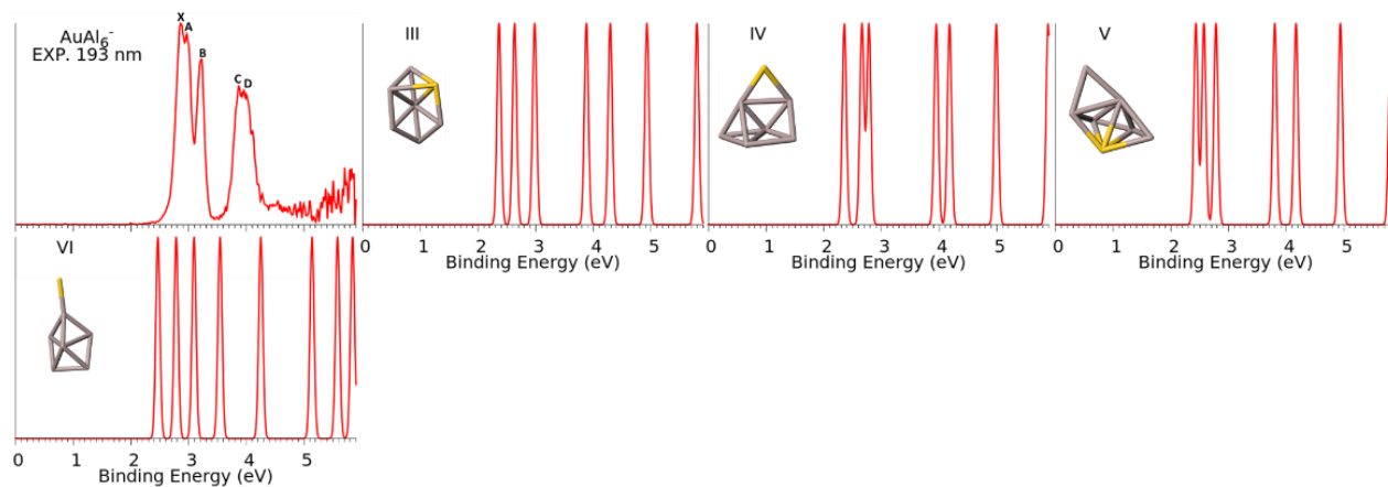
Figure S1. Comparison of the simulated spectra for the isomers III to VI of \text{AuAl}_6^- with the 193 nm experimental spectra.
