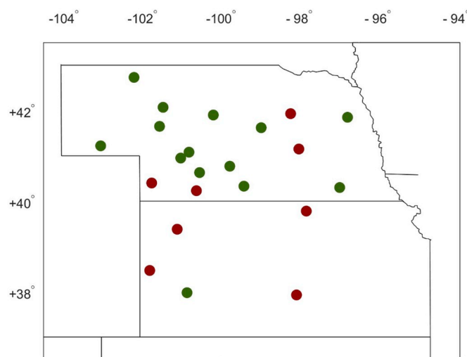
Fig. 1. Location of stations included in the study. Maroon and green colored circles represent irrigated and grassland sites, respectively. (For interpretation of the references to color in this figure legend, the reader is referred to the Web version of this article.)
