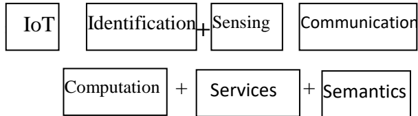
Fig 1: IoT Elements
