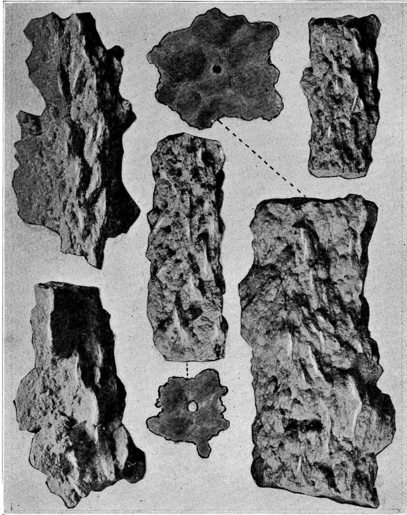
Fig. 21. Sections of manganese fulgurites, side and end views. The smaller end view has a filling of calcite. The larger is hollow. Four-fifths natural size.
