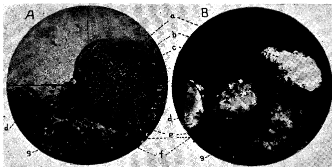
FIG. 43. A. Plane polarized. B. Crossed nicols. A Biaxial mineral on exterior surface of the crest of a ridge. a, Exterior crystalline portion still giving good optical reactions. b, Zone of semi-fused crystal with fringing structure very much resembling the character of albite when heated to 1125° Cent. See Iddings, Carnegie Institute of Washington, No. 31, Pl. XIX. c, Zone of vitrified crystal; grain apparently squeezed outward by f and e during folding of crest. d, Feldspar, very slightly granulated on interior margin. e, Quartz grain. f, Feldspar, granulated. g, Feldspar fragment. X 110.
