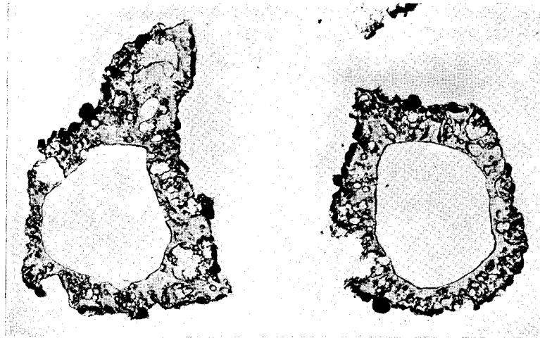
FIG. 29. Sections of the Poland specimen made by Julian figured in his "A Study of the Streamers in Fulgurites," Journal of Geology , Vol. IX, No. 8, 1901.
