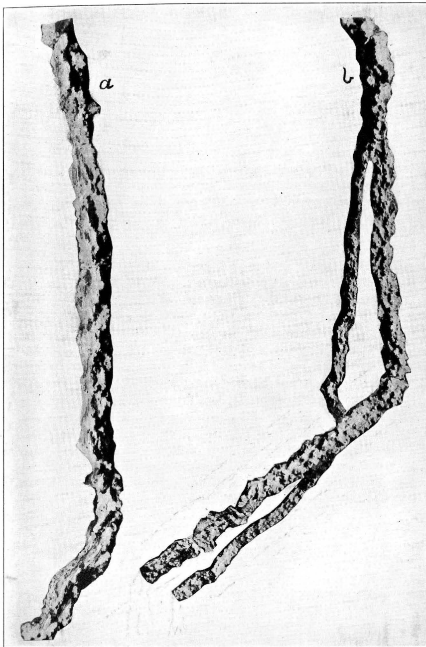
Plate 1 The Stanton County Fulgurite. Lower nine feet. The part a belongs on the part b.
