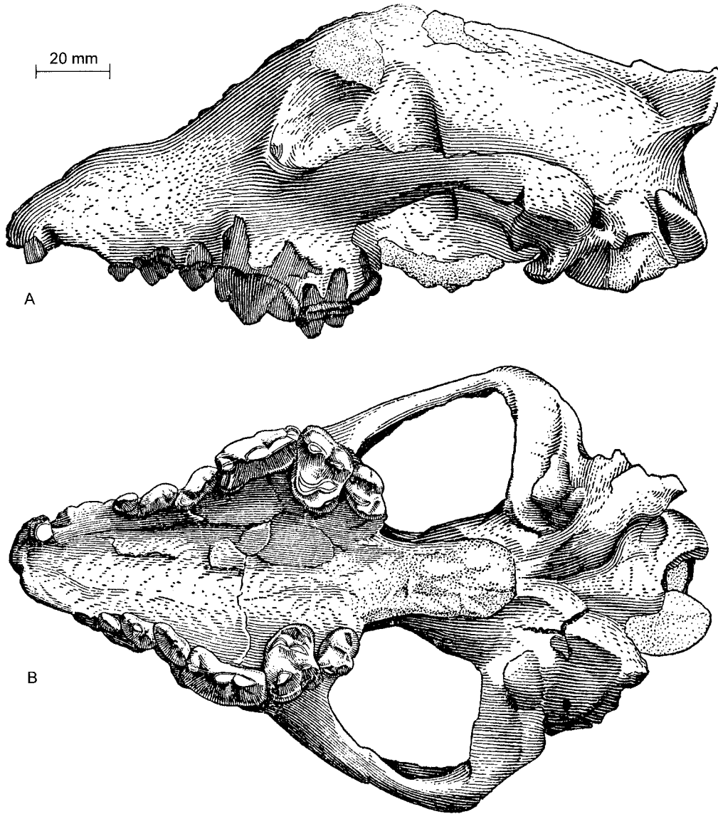
Fig. 116. Borophagus littoralis . A , Lateral and B , ventral views of skull, UCMP 34515, Black Hawk Ranch Quarry, Green Valley Formation (late Clarendonian), Contra Costa County, California. Modified from Macdonald (1948: fig. 5), both reversed from the original figures.
