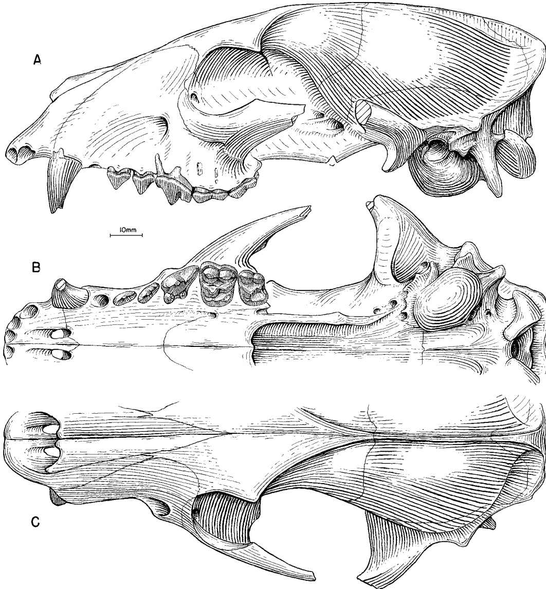
Fig. 54. Paracynarctus sinclairi . A, Lateral, B, ventral, and C, dorsal views of skull, F:AM 61009, holotype, Quarry 2, Olcott Formation (early Barstovian), Sioux County, Nebraska.
