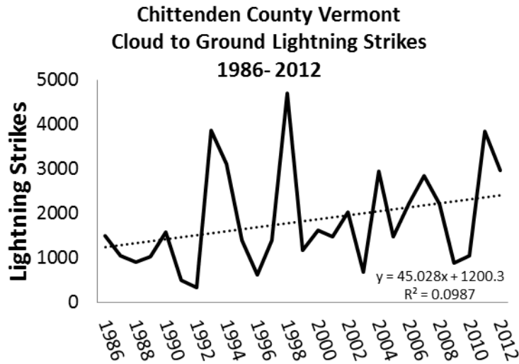
Figure 3.14. Increasing lightning strikes indicate increasing intensity of electrical storms (NWS 2014).
