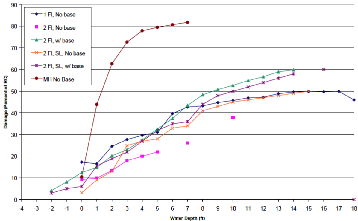
Figure 3.16 Imbalanced damages to mobile homes, FIA Credibility-Weighted Building Depth-Damage Curves as of 12/31/1998.
