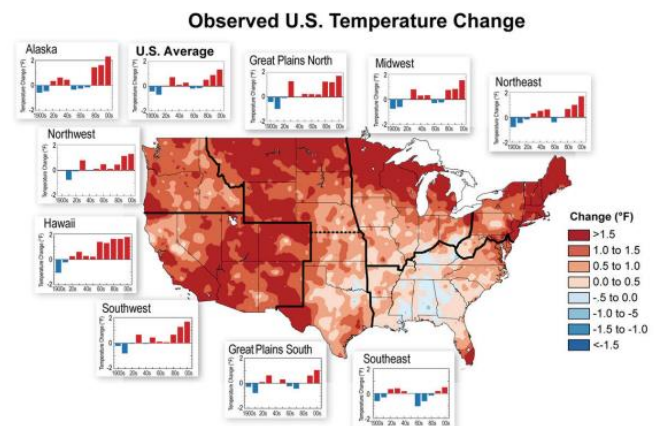
Figure 1.2. Temperatures changes over the past 20 years (1991-2011) compared to the 1901-1960 average. Bar plots show average temperature changes by decade for 1901-2011 relative to the 1901-1960 average by region (Melillo et al. 2014).
