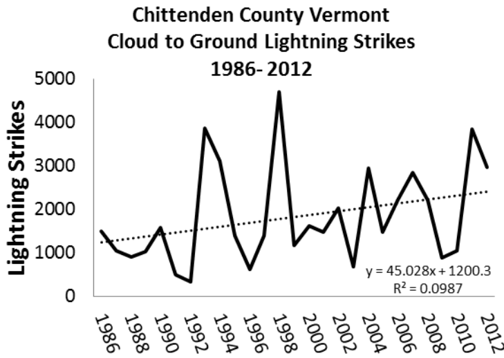
Figure 17. Chittenden County, Vermont: Cloud to ground lightning strikes.
