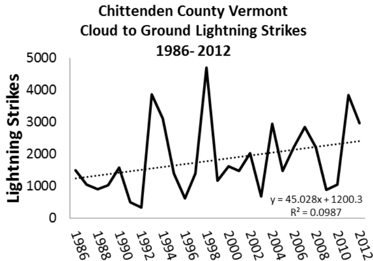
Figure 4.5. Chittenden County, Vermont: Cloud to ground lightning strikes (Chapter 1, this report).
