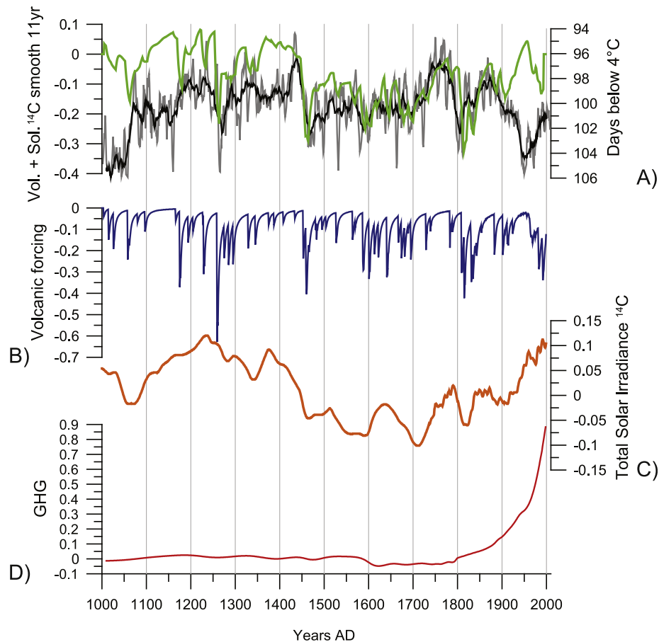
Fig. 7. DB4 °C variations (this study) in response to forcings. A) combined solar and volcanic forcing (green, 11 years smoothed) (Crowley, 2000), compared to the chrysophyte based-DB4 °C reconstruction (grey line, 5-yr filter; black line 21-yr. filter), B) volcanic forcing (blue), C) Total Solar Irradiance (orange), and D) GHG (red). (For interpretation of the references to colour in this figure legend, the reader is referred to the web version of this article.)
