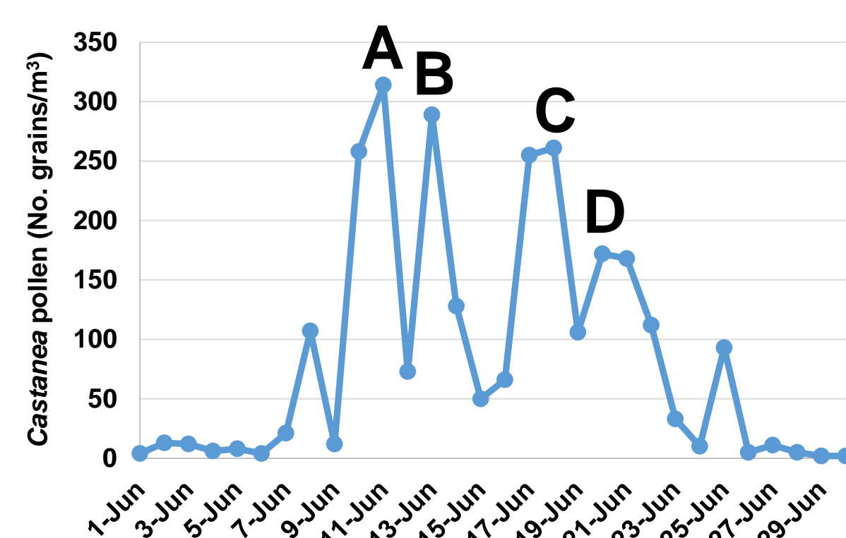
Daily concentration of Castanea pollen during June 2017. Capital letters correspond to the peak days.
