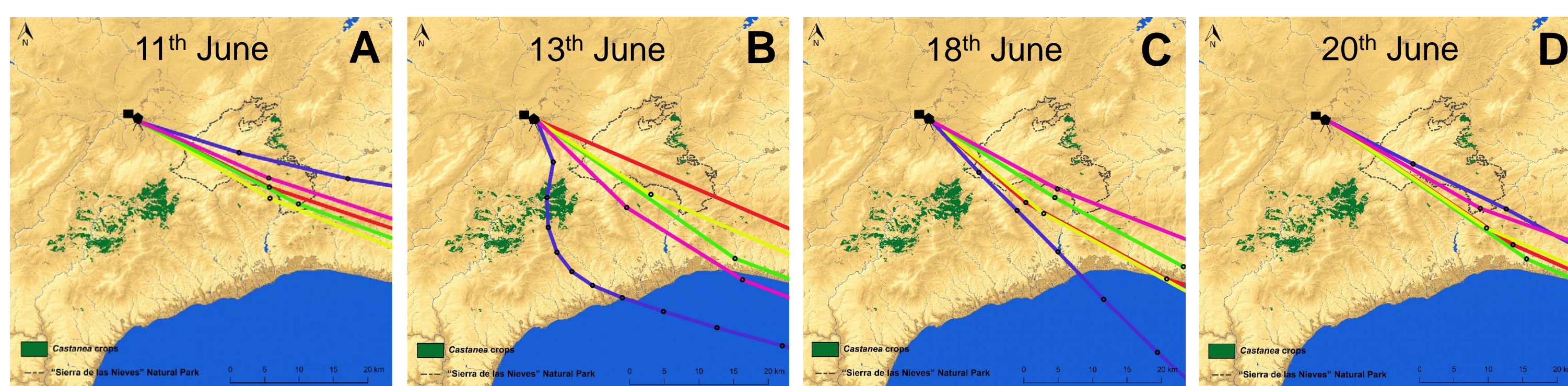
Backward air trajectories of backward air trajectories for each peak day of Castanea pollen. Red at 06h; blue at 18h and pink at 23h. The distance between two points in each trajectory shows the movement of the air mass in one hour. Capital letters correspond to each peak day of Castanea pollen (graph below).
