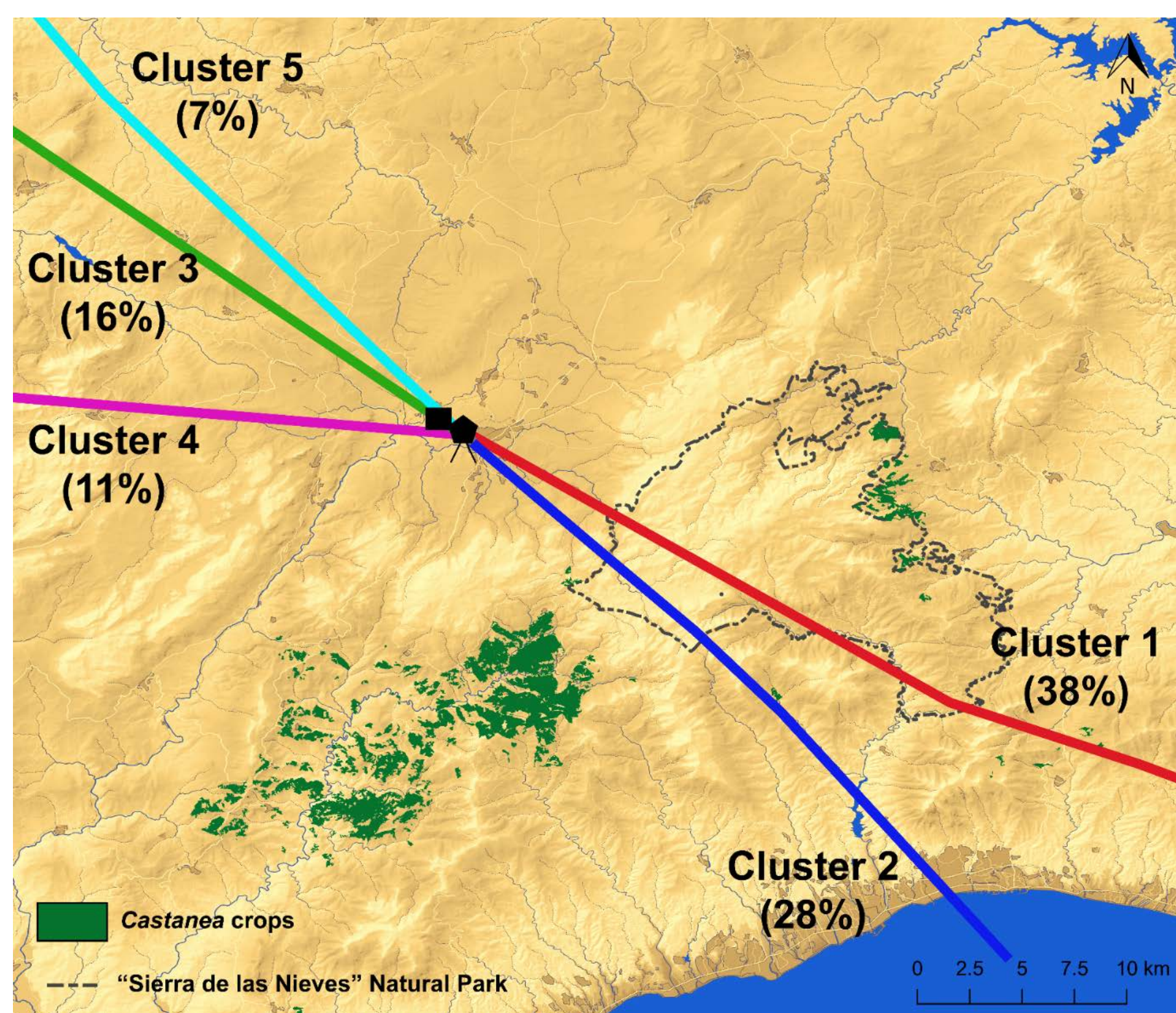
Spatial representation of mean air trajectories during June 2017 in the study area. The number in parenthesis is the percentage of trajectories in each cluster. Castanea crops are represented in green and the limits of "Sierra de las Nieves" Natural Park are delimited with a dashed line.
