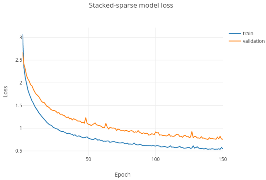
Figure 7: Training and validation loss curves of the stacked-sparse architecture.
