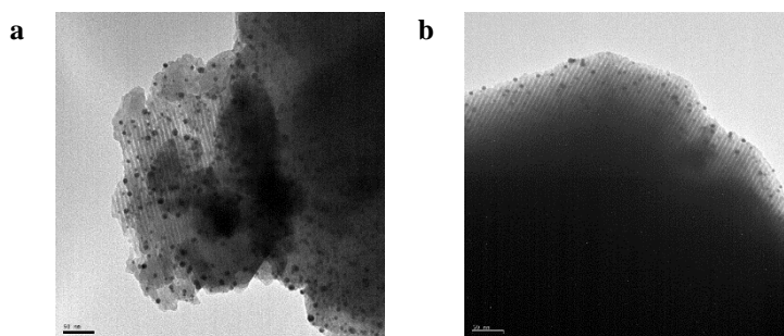
Figure 1: TEM images of (a) Au/SBA-15 and (b) Au/TiSBA-15
