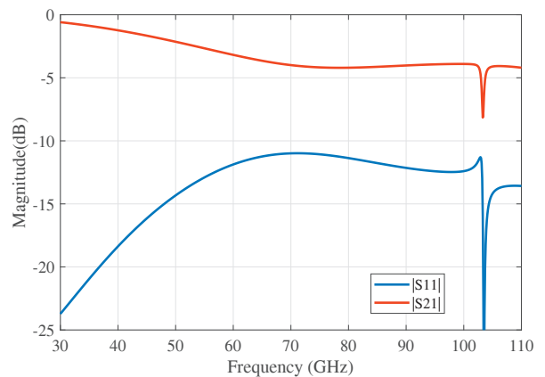
Fig. 3. Magnitude of the S-parameters of the simulated structure.
