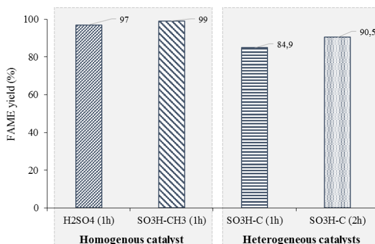
Figure 2. Catalytic activity of sulfonated carbon: 12:1=MeOH:Oil; 120^\circ\text{C} ; 10.34 bar; 3 wt% catalysts.
