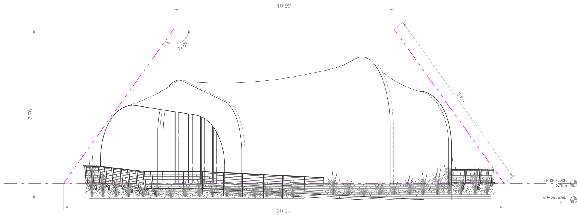
1 SOLAR ENVELOPE DIAGRAM-SOUTH EAST
