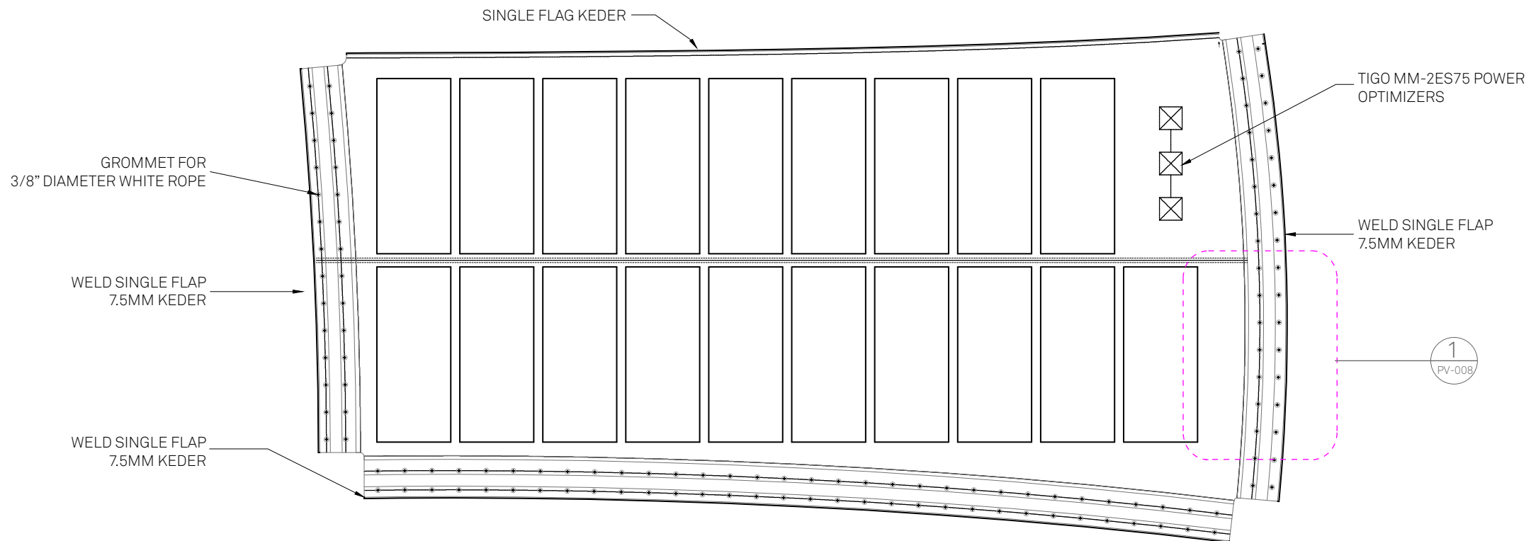
1 PVILION PHOTOVOLTAIC SYSTEM - ASSEMBLY C PROPRIETARY PVILION TECHNOLOGY, PATENTS PENDING
