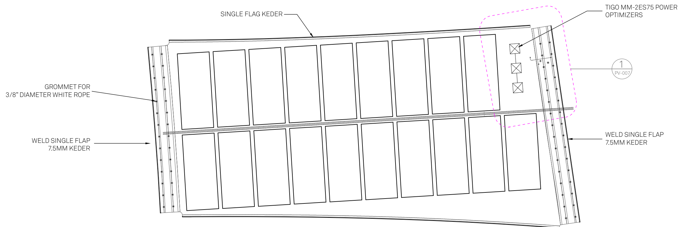
2 PVILION PHOTOVOLTAIC SYSTEM - ASSEMBLY B PROPRIETARY PVILION TECHNOLOGY, PATENTS PENDING
