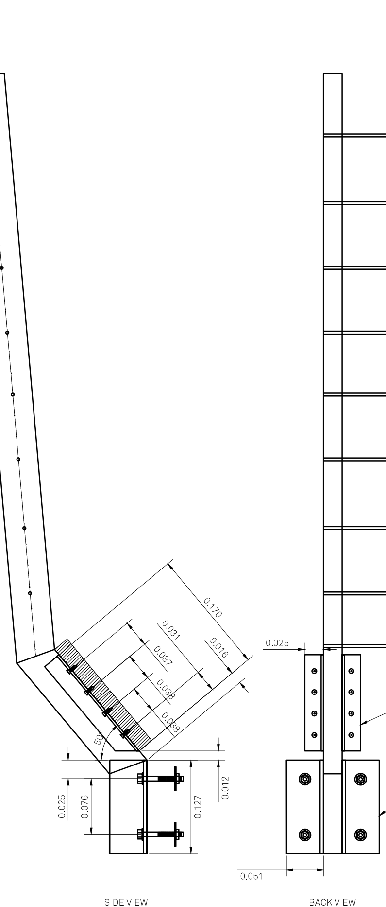
SIDE VIEW
