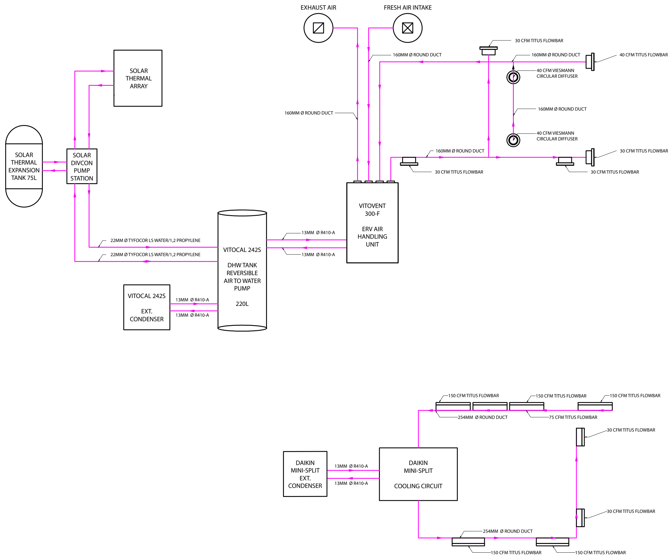
1 SYSTEM SCHEMATIC
