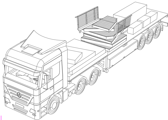
TRUCK N O. 3 FLOOR PALLETS SOUTH DECK MISCELLANEOUS Load: 1,810 kg
