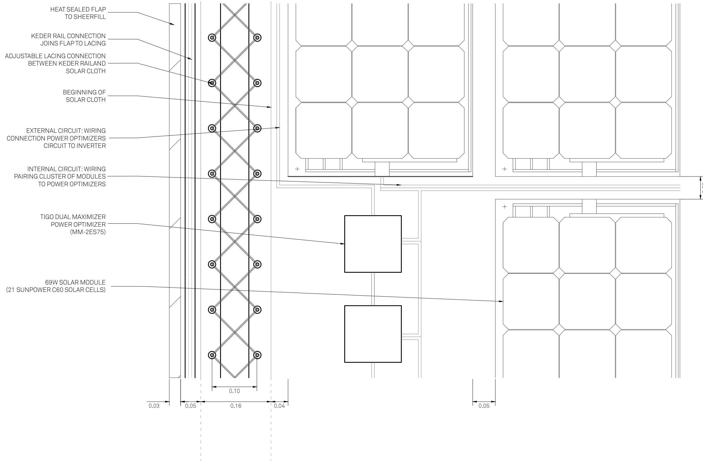
1 PHOTOVOLTAIC SYSTEM ATTACHMENT - PLAN DETAIL
