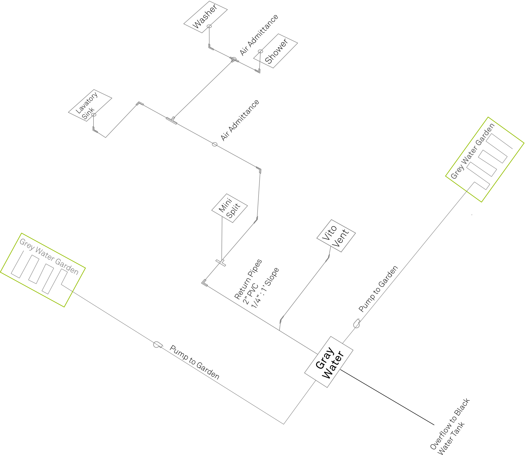
1 GRAY WATER ISOMETRIC
