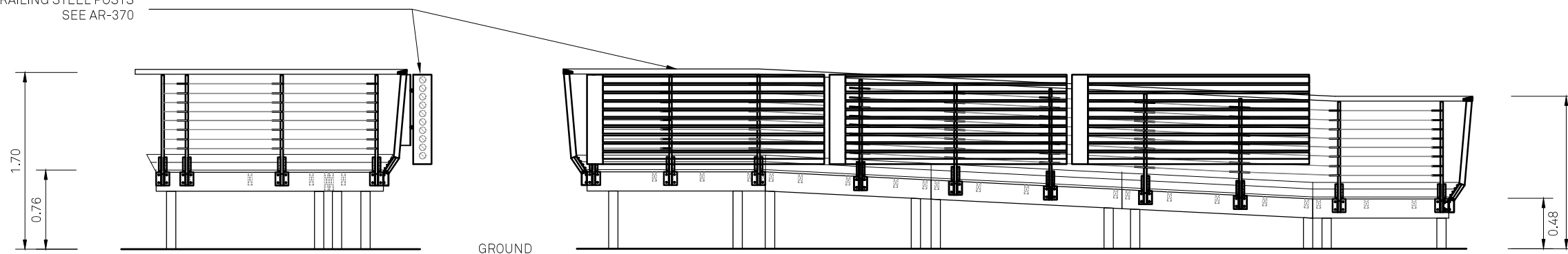
2 DECK ELEVATION - SOUTH WEST
