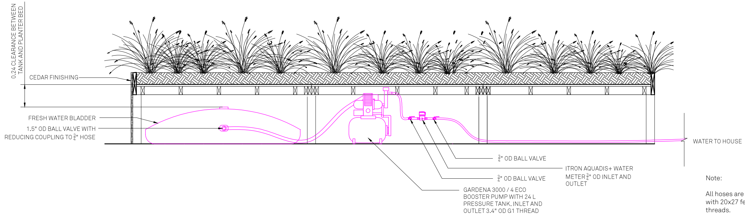
2 FRESH WATER PUMP SECTION
