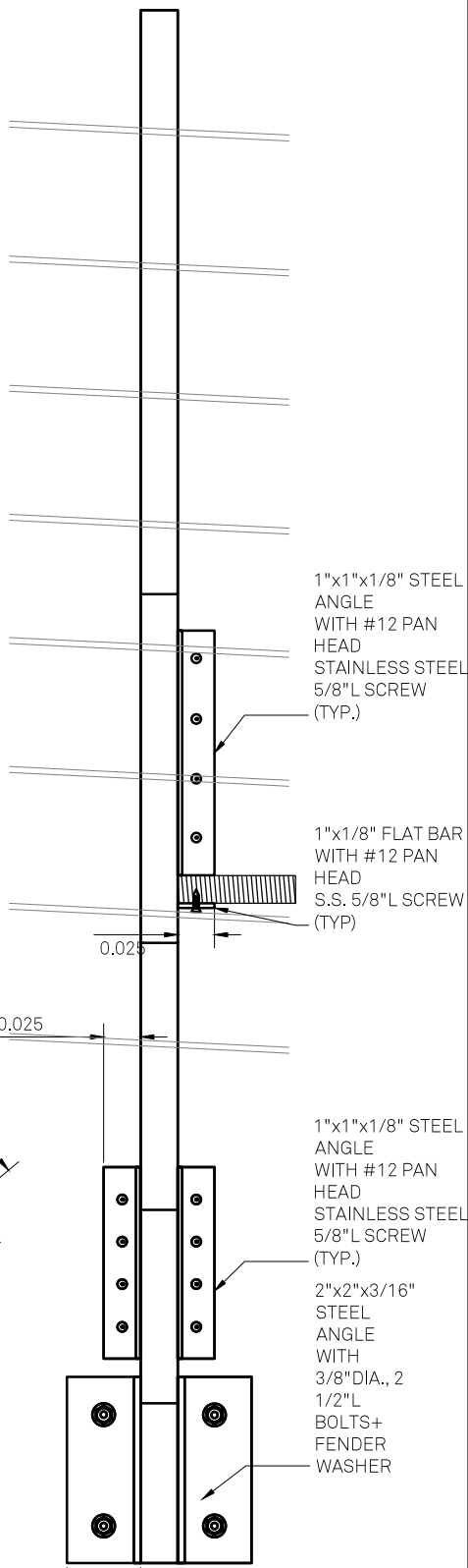
BACK VIEW
