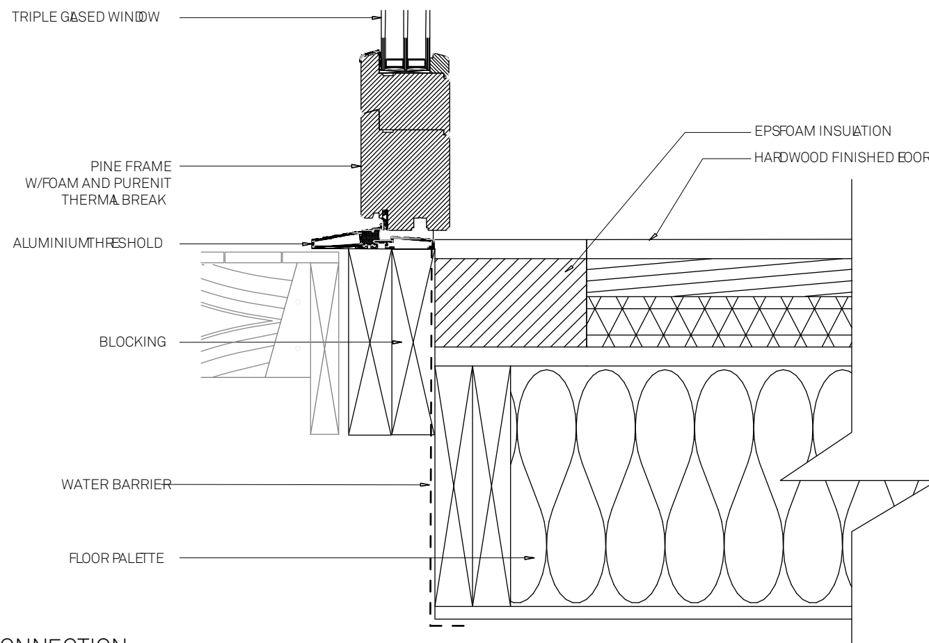
1 DOOR TO FLOOR CONNECTION
