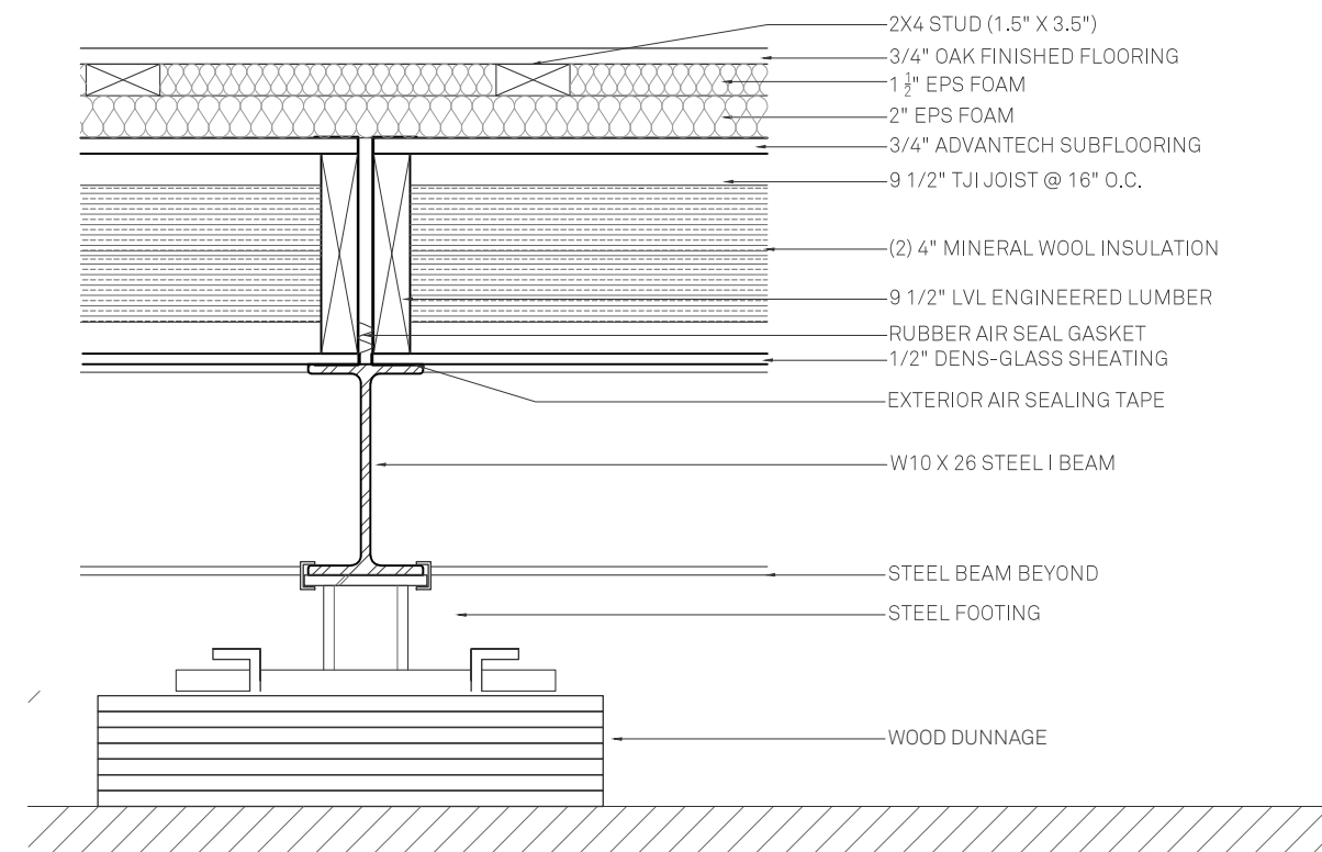
2 FLOOR PALETTE LONGITUDINAL SECTION DETAIL
