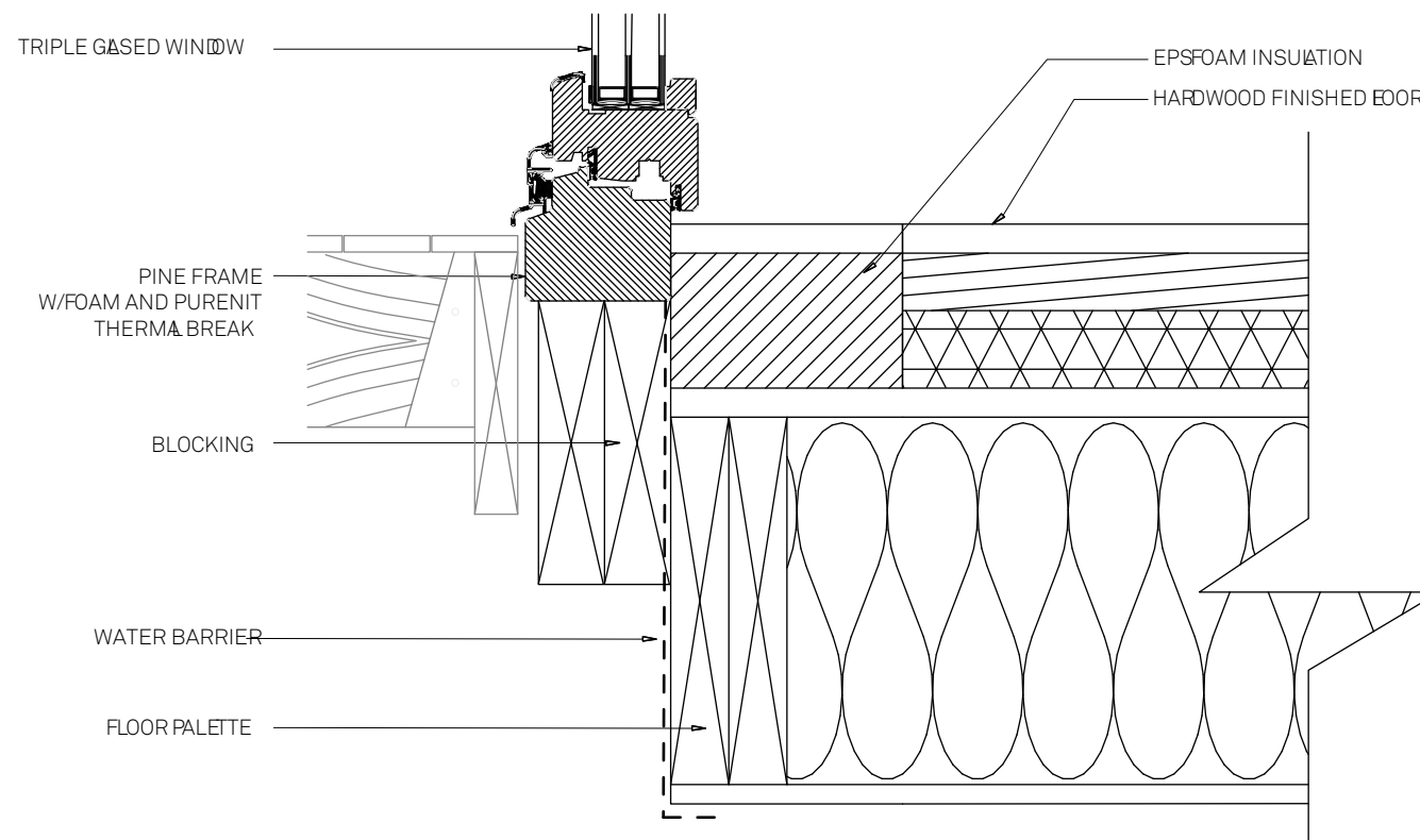
2 WINDOW TO FLOOR CONNECTION
