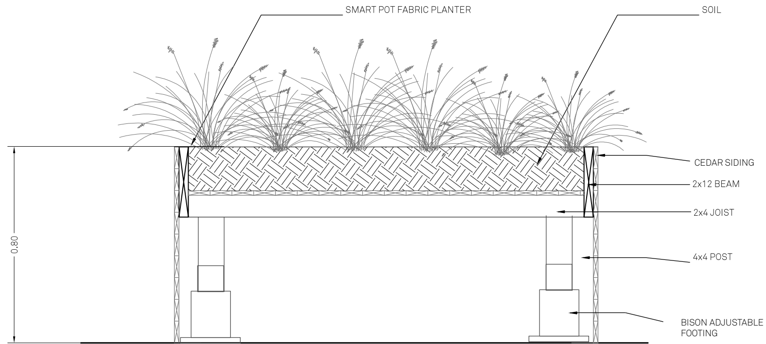
2 SOUTHERN EDIBLE GARDEN SECTION
