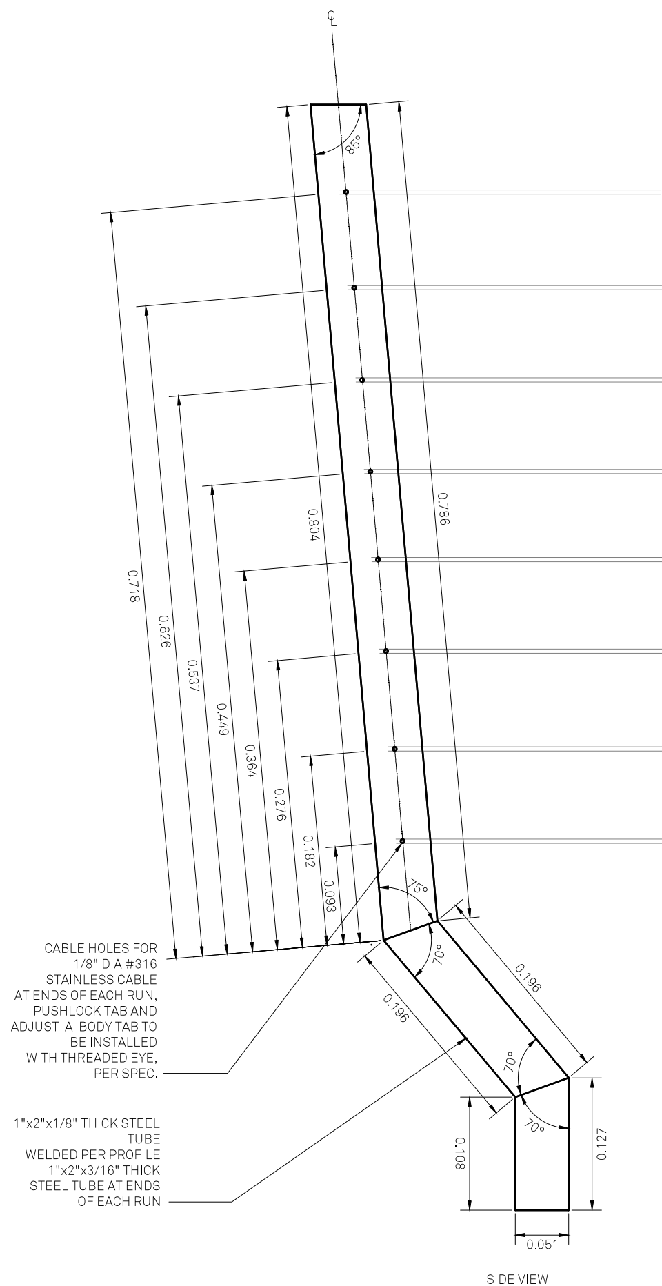
SIDE VIEW
