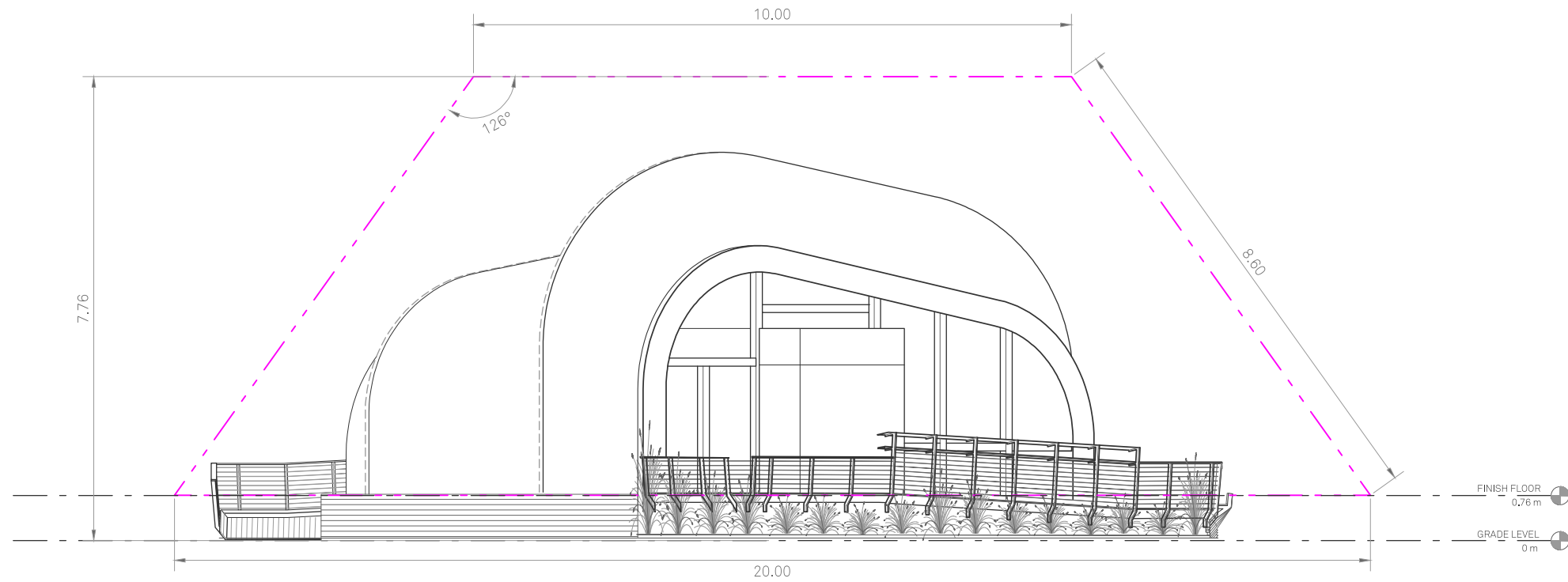
1 SOLAR ENVELOPE DIAGRAM-NORTH EAST
