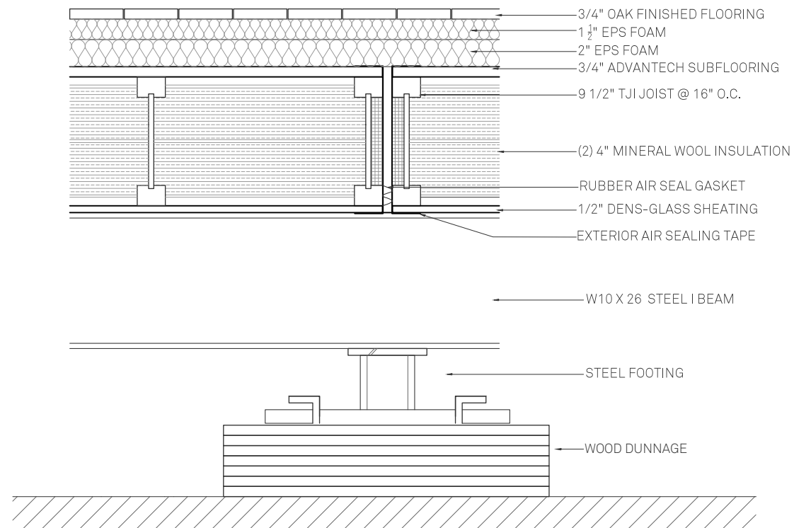
1 FLOOR PALETTE CROSS SECTION DETAIL
