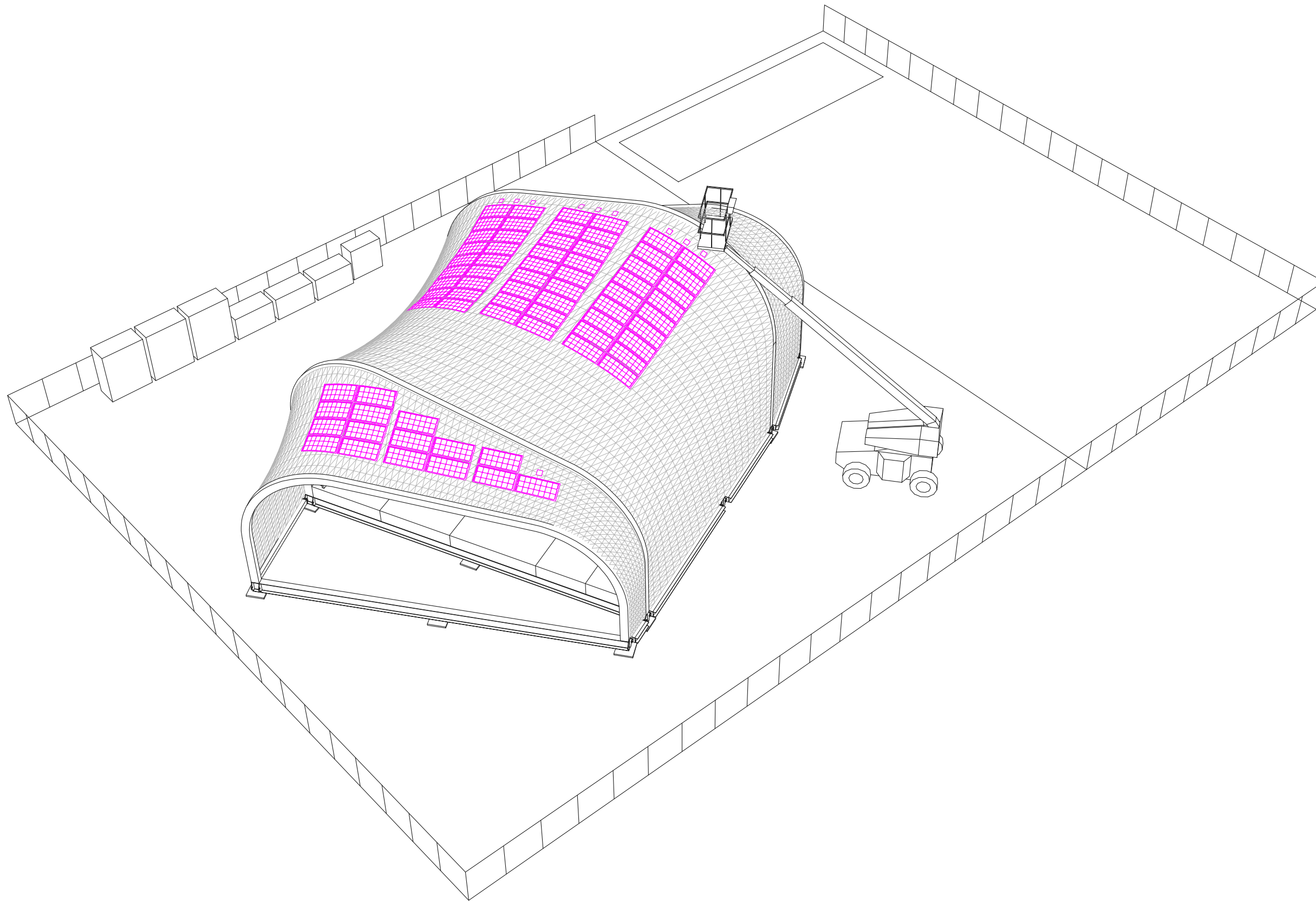
1 INSTALLATION OF SOLAR ARRAY
