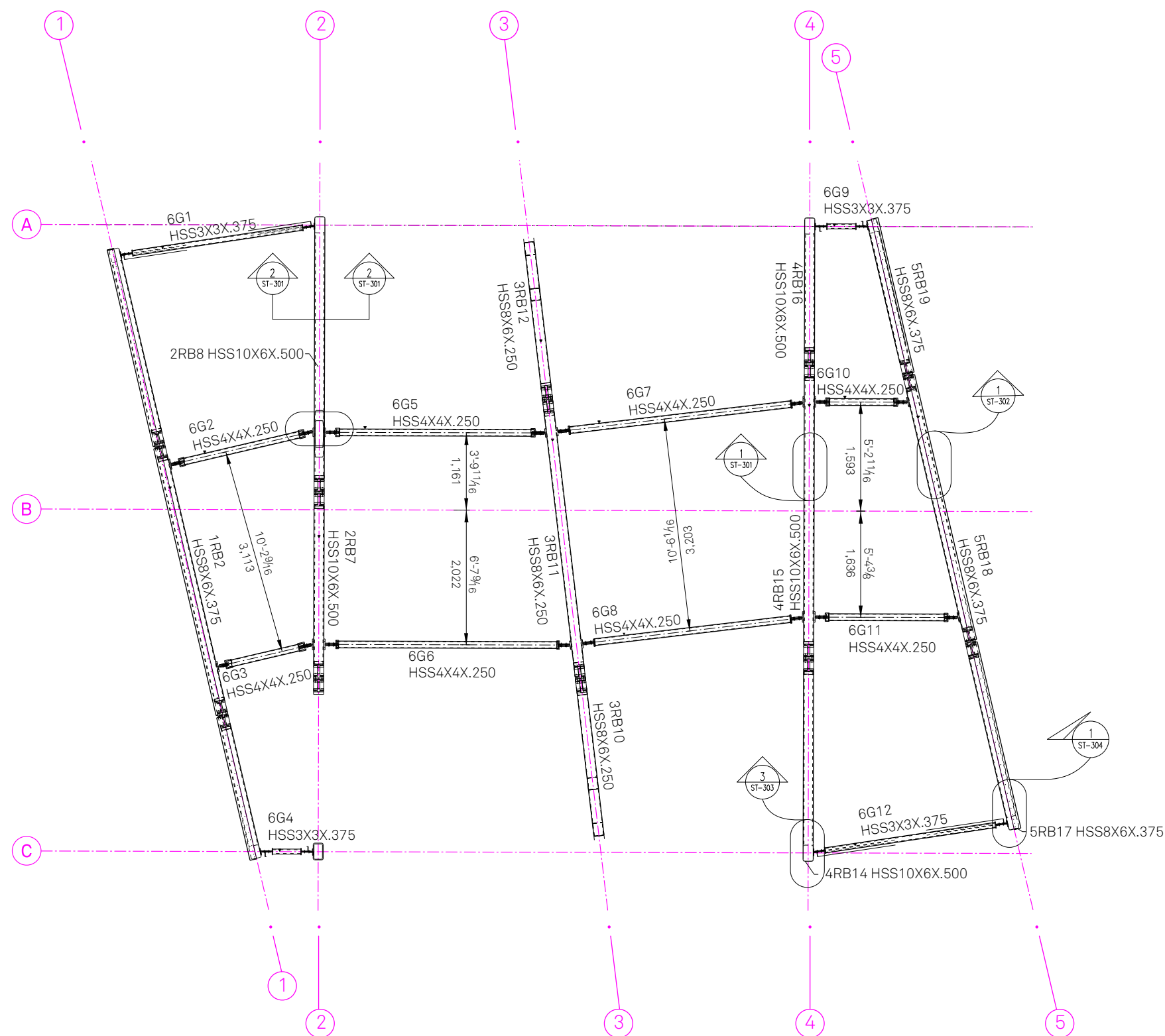
① STRUCTURAL RIB PLAN
