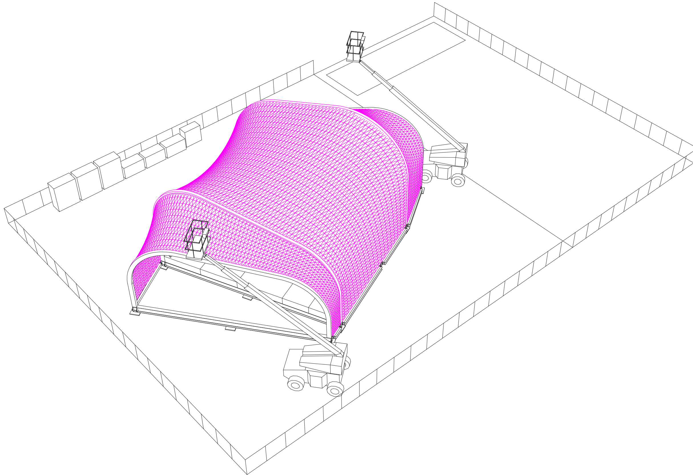
1 SHEERFILL MEMBRANE INSTALLATION
