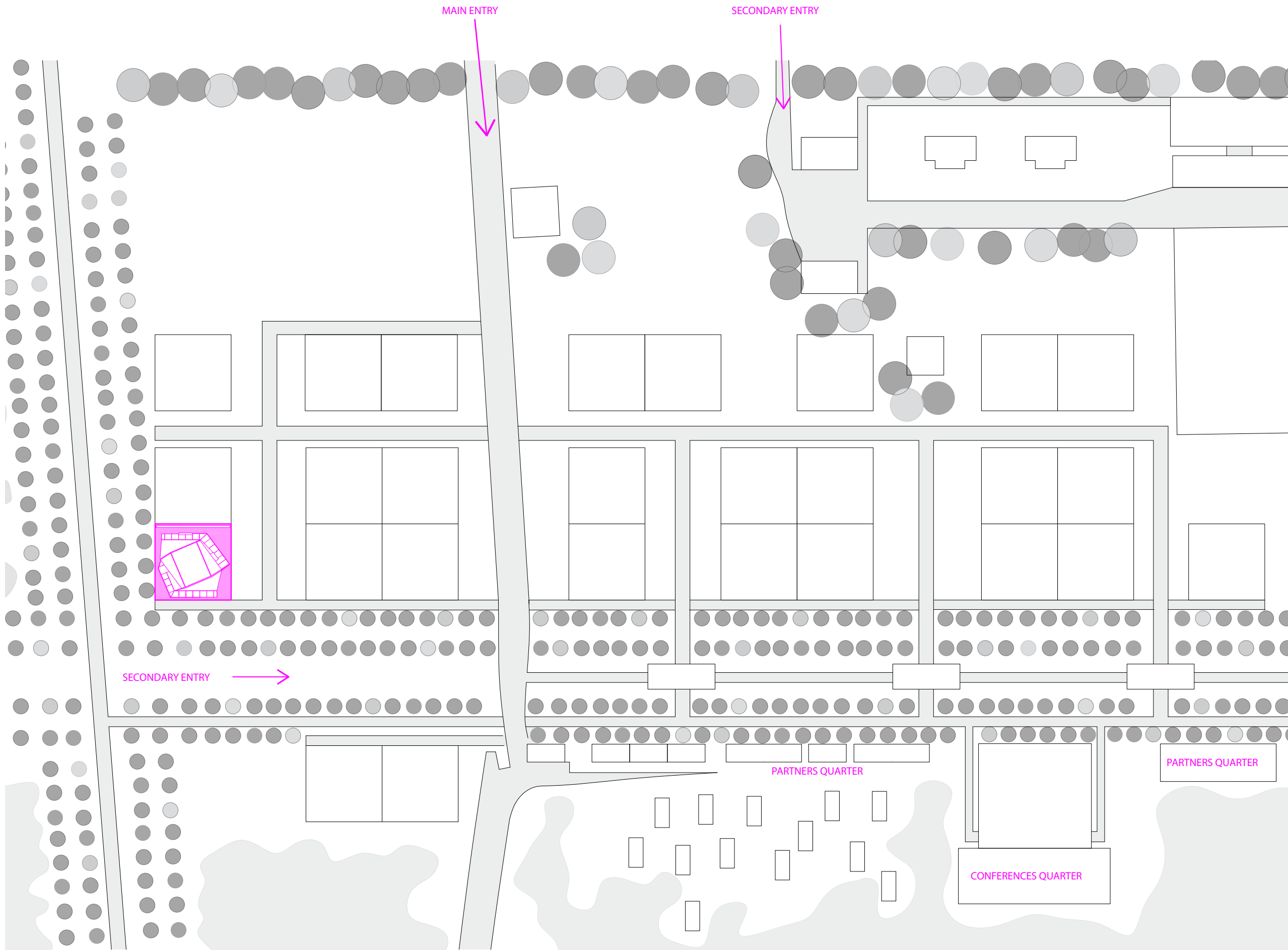
1 SOLAR VILLAGE PLAN | TECHSTYLE HAUS - SITE C
