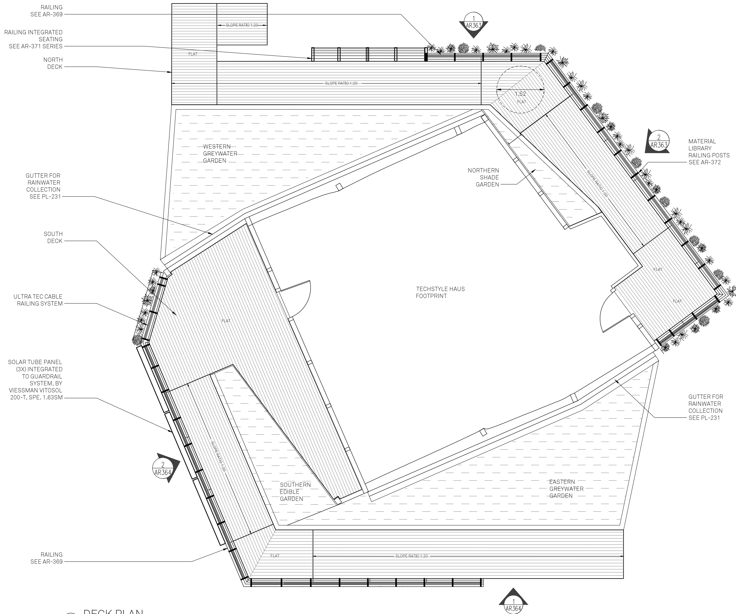
1 DECK PLAN
