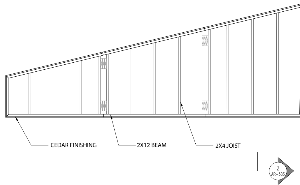
1 SOUTHERN EDIBLE GARDEN FRAMING
