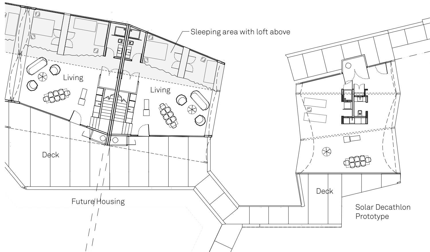
1 FIRST FLOOR PLAN
