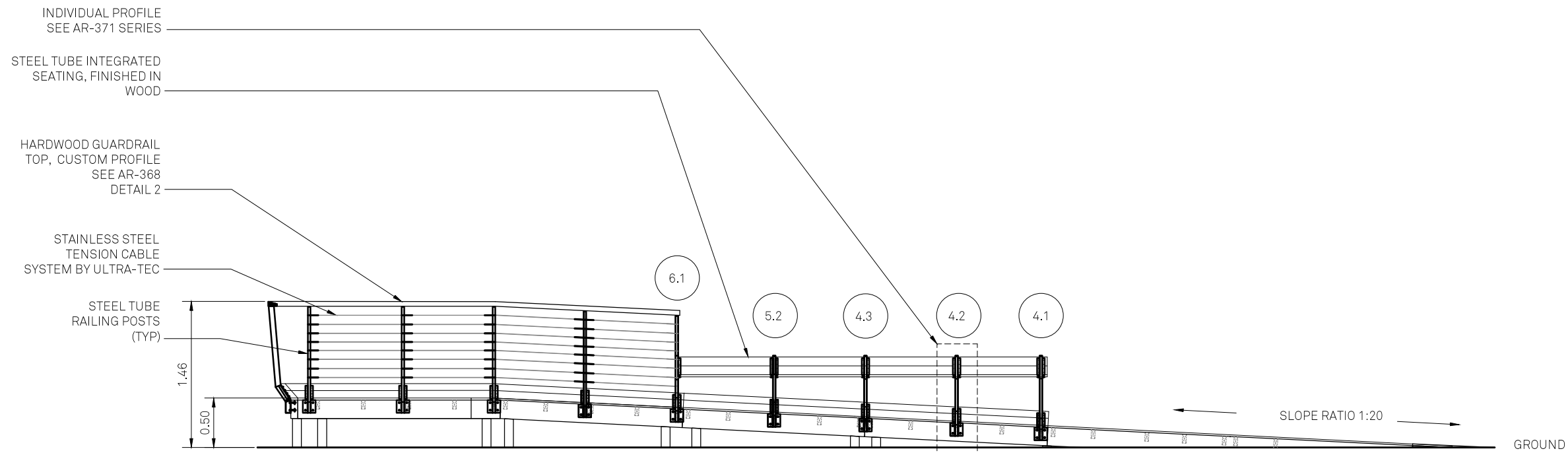
1 DECK ELEVATION - NORTH WEST
