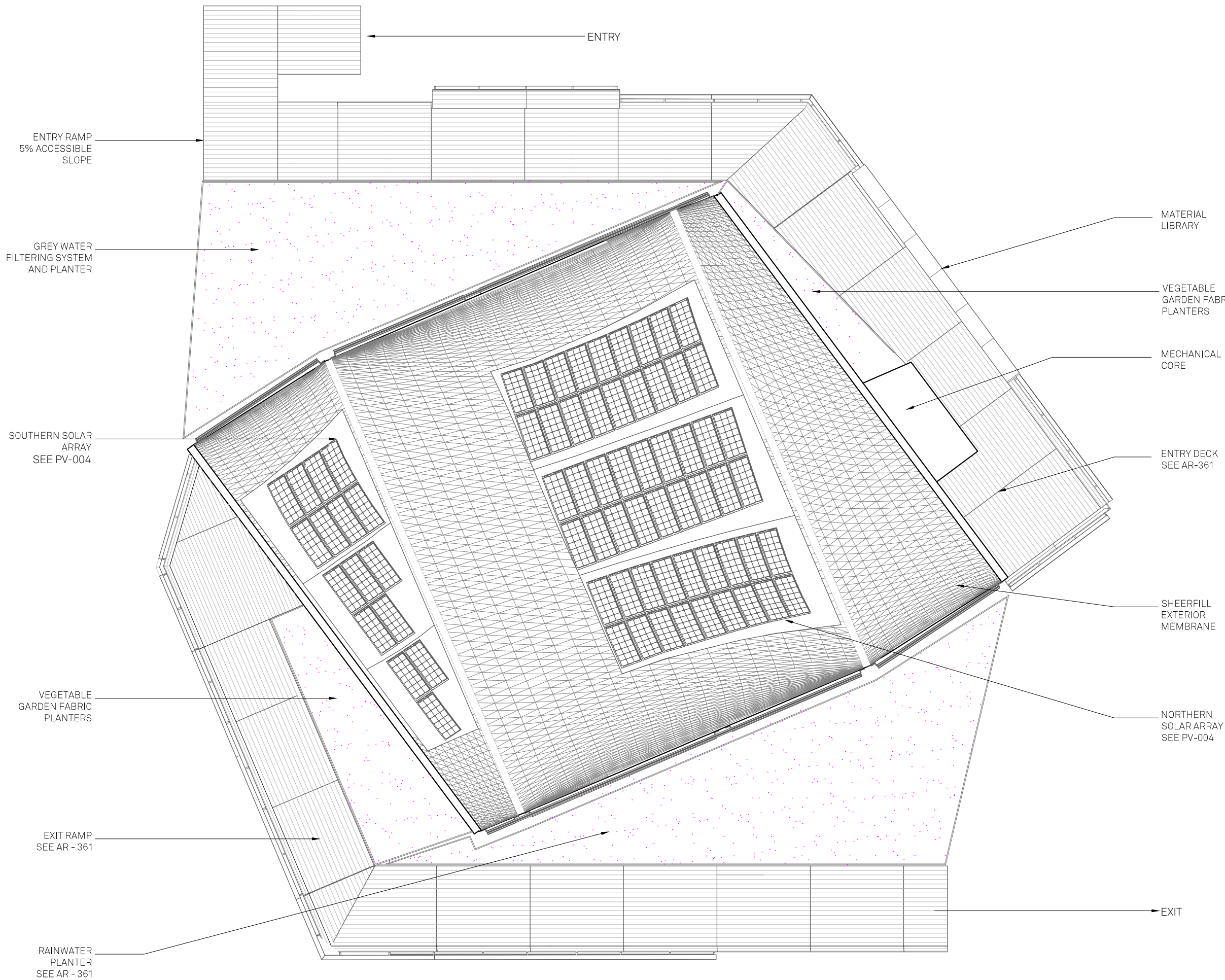
1 SITE PLAN
