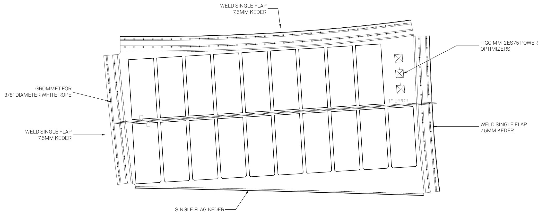
1 PVILION PHOTOVOLTAIC SYSTEM - ASSEMBLY A PROPRIETARY PVILION TECHNOLOGY, PATENTS PENDING
