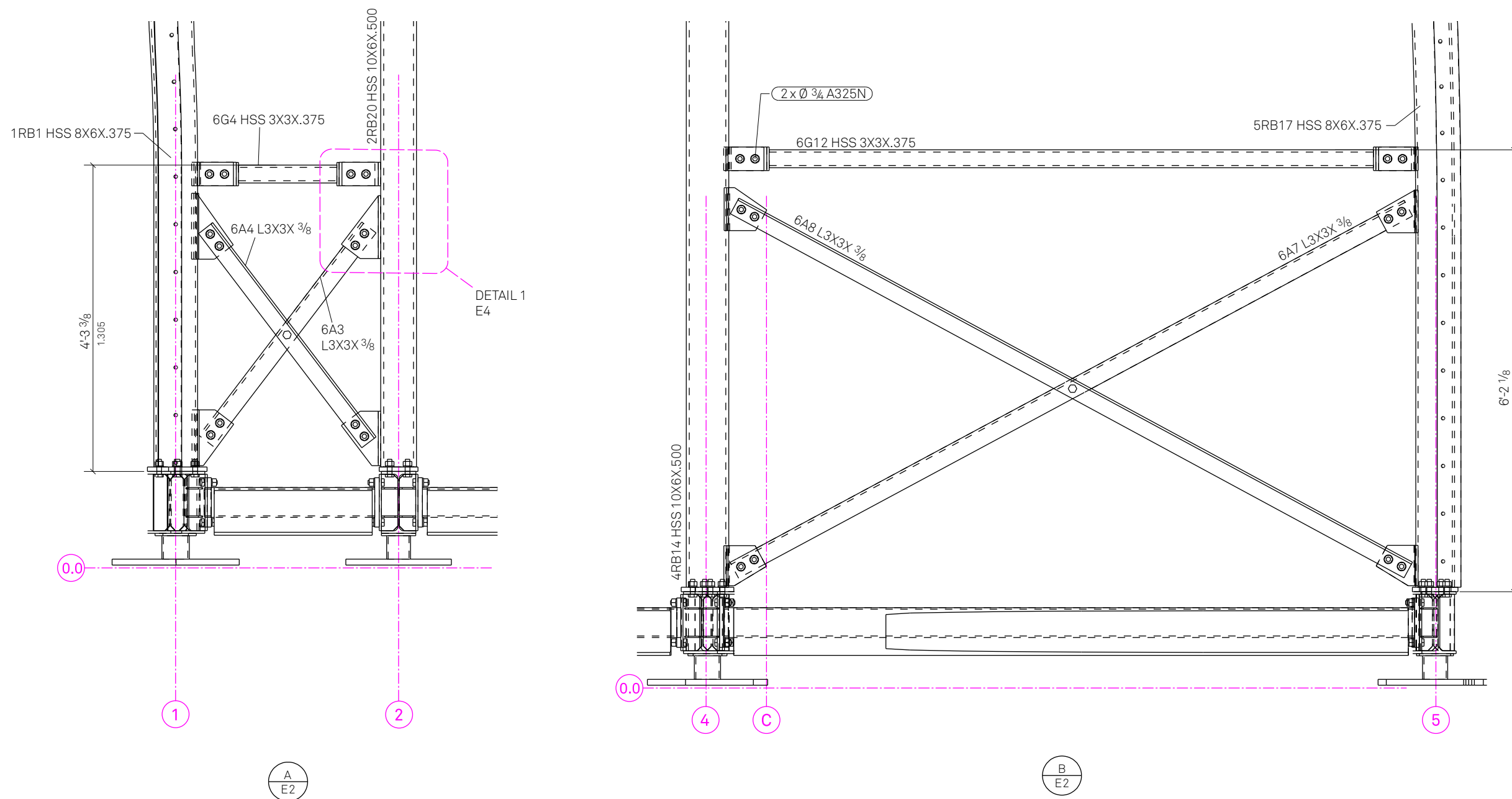
1 STEEL BRACING CONNECTION DETAILS
