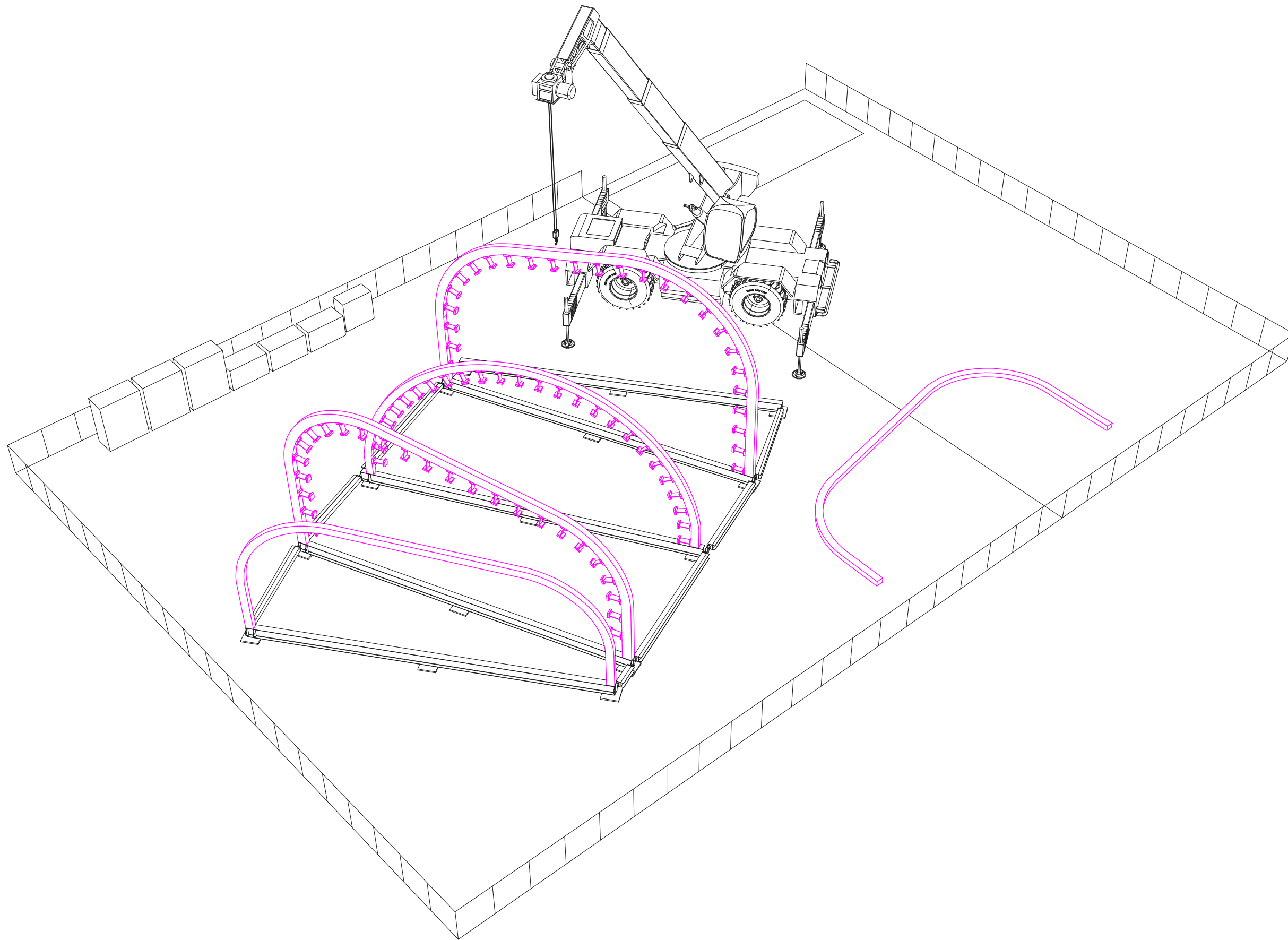
1 STEEL RIB ERECTION
