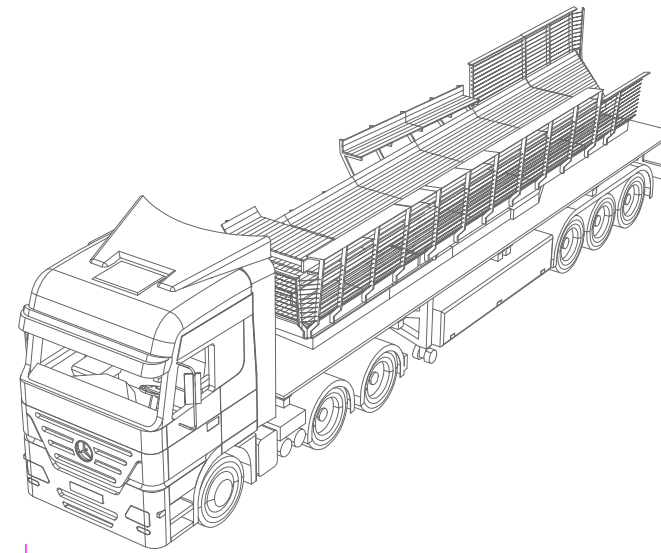
TRUCK N O. 10 DECK S PLANTER S SOLAR THERMAL ARRAY Load: 1,000 kg
