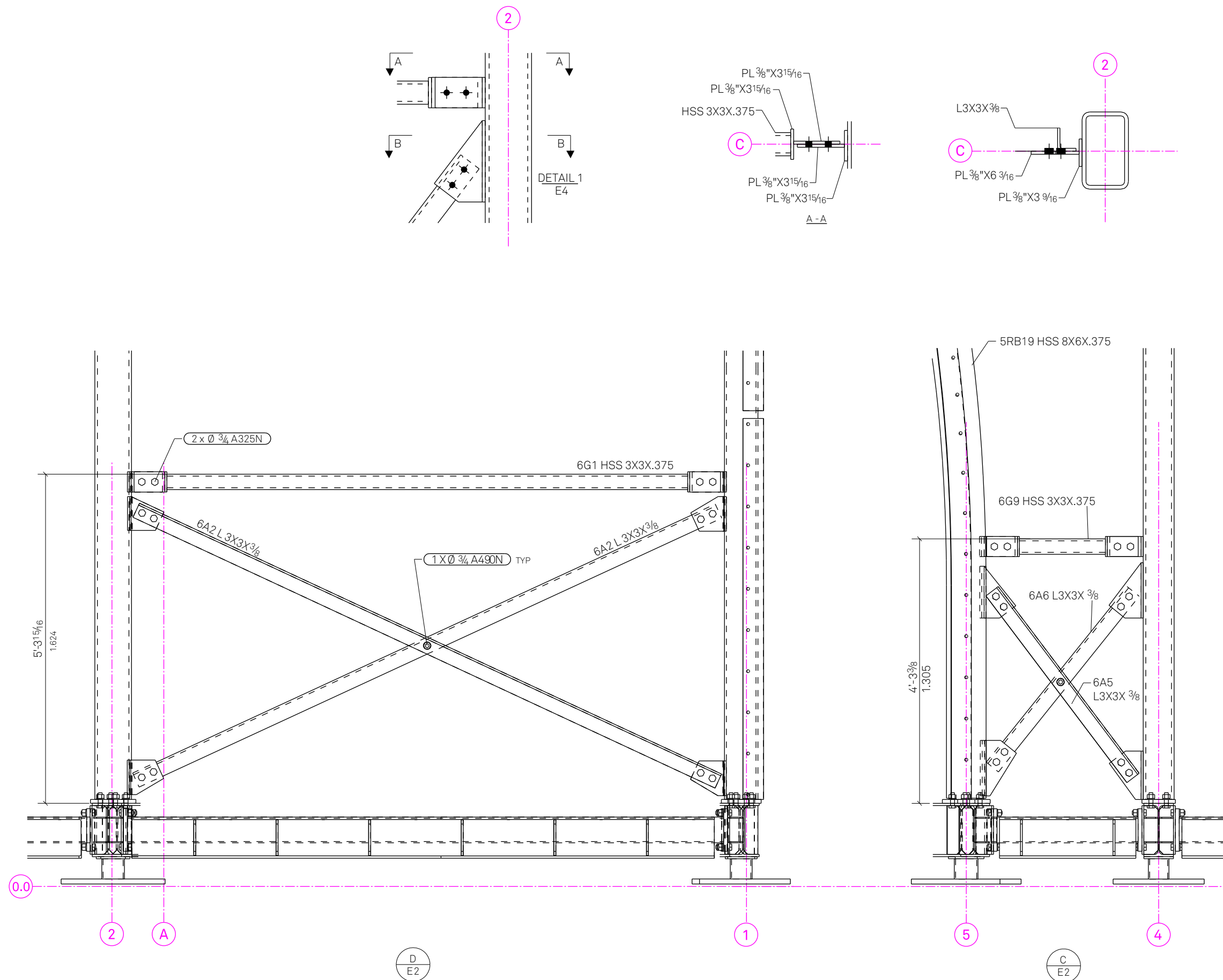
1 STEEL BRACING CONNECTION DETAILS
