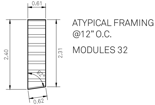
CORE FRAMING @12" O.C. EXTRA SUPPORT ON ENDS AND CENTER MODULES 20-24
