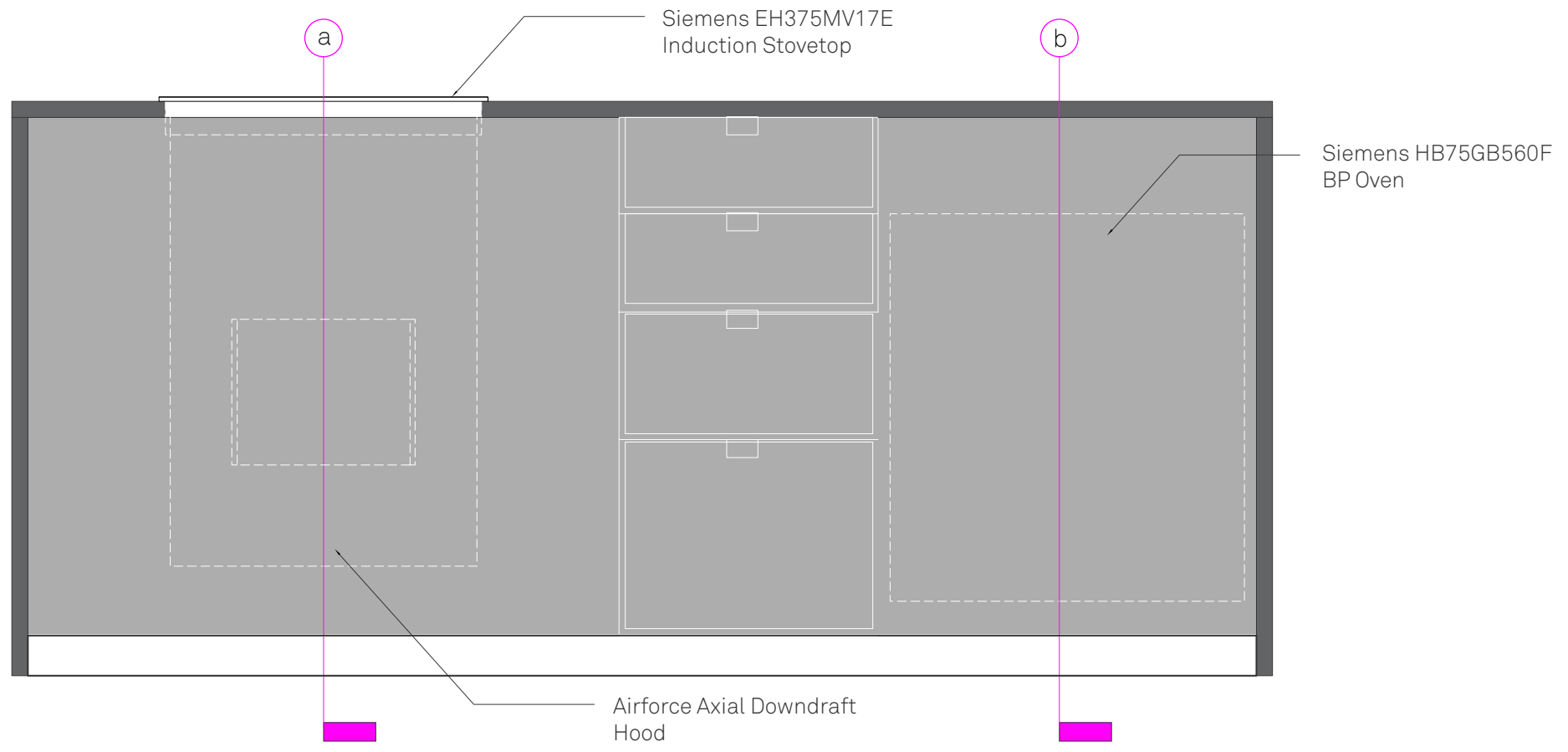
1 KITCHEN ISLAND SECTIONS AND ELEVATION
