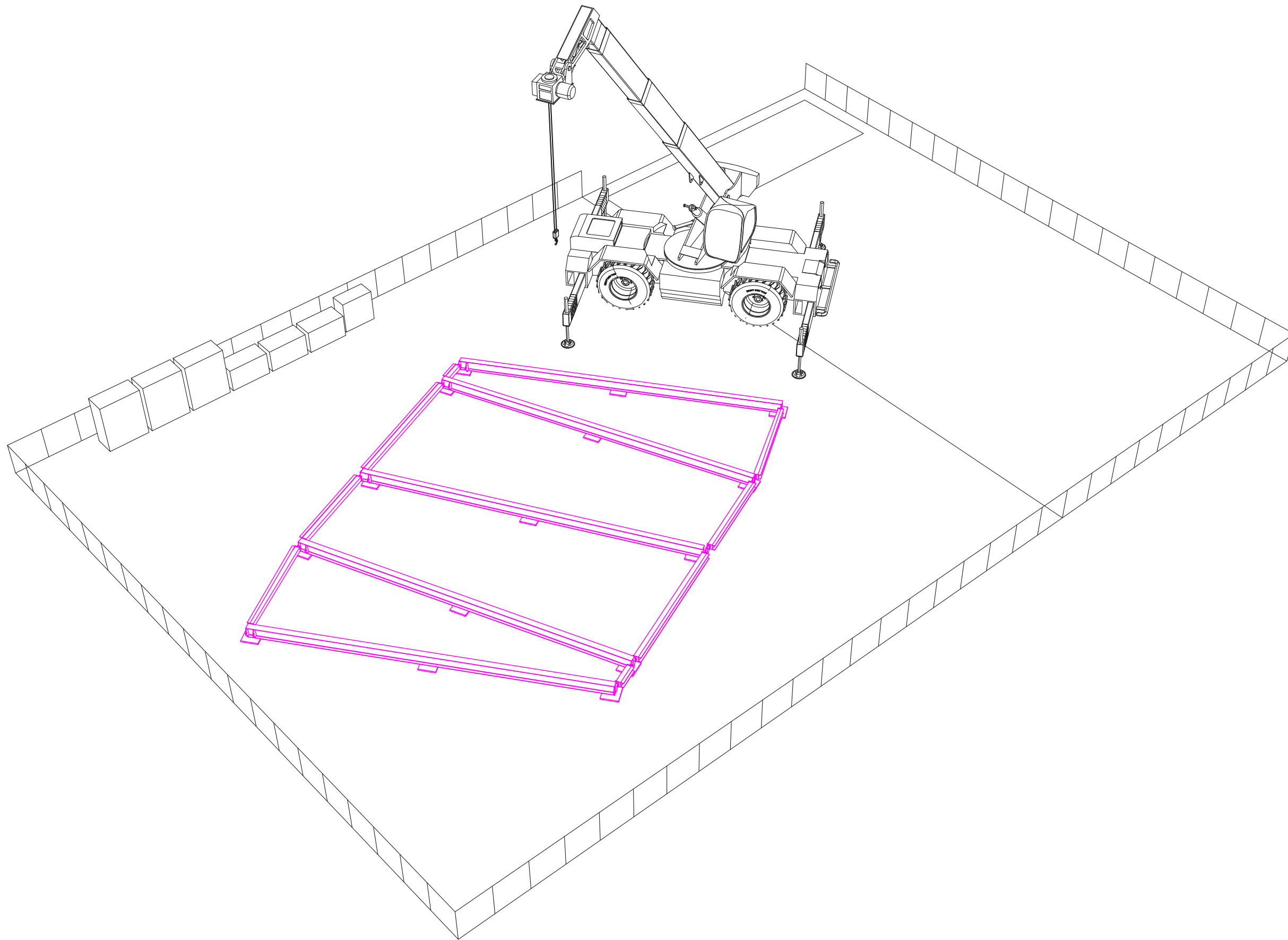
1 STEEL BASE FRAME ERECTION
