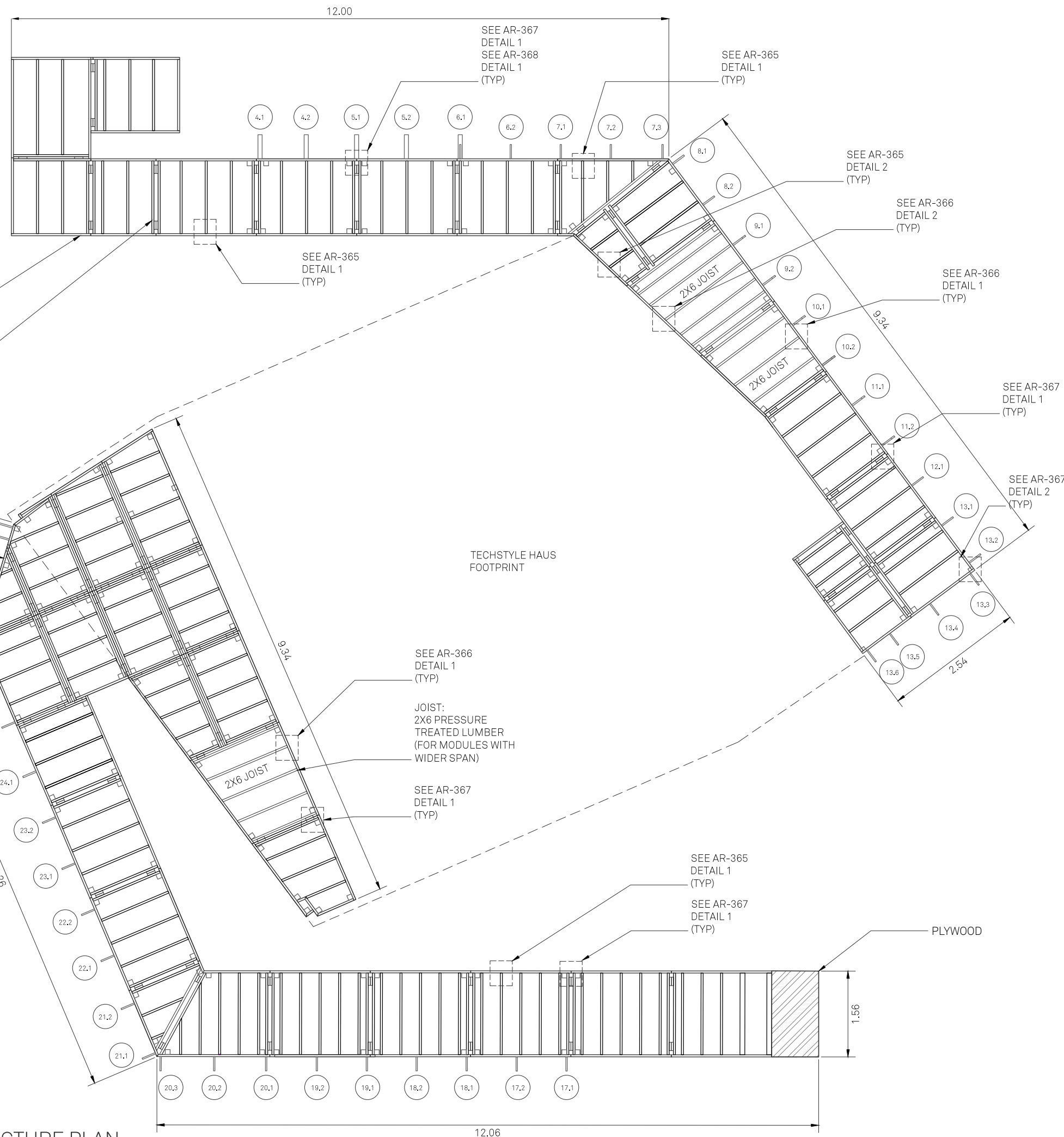
2 DECK STRUCTURE PLAN
