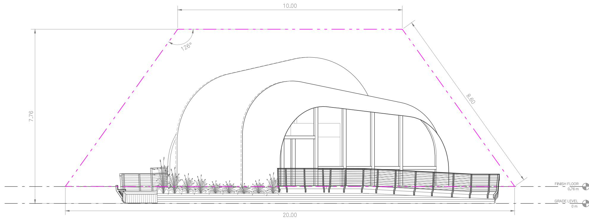
2 SOLAR ENVELOPE DIAGRAM-SOUTH WEST
