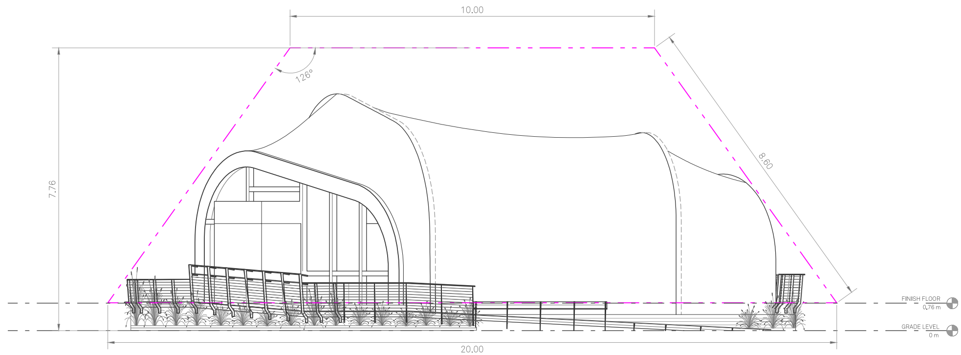
2 SOLAR ENVELOPE DIAGRAM-NORTH WEST
