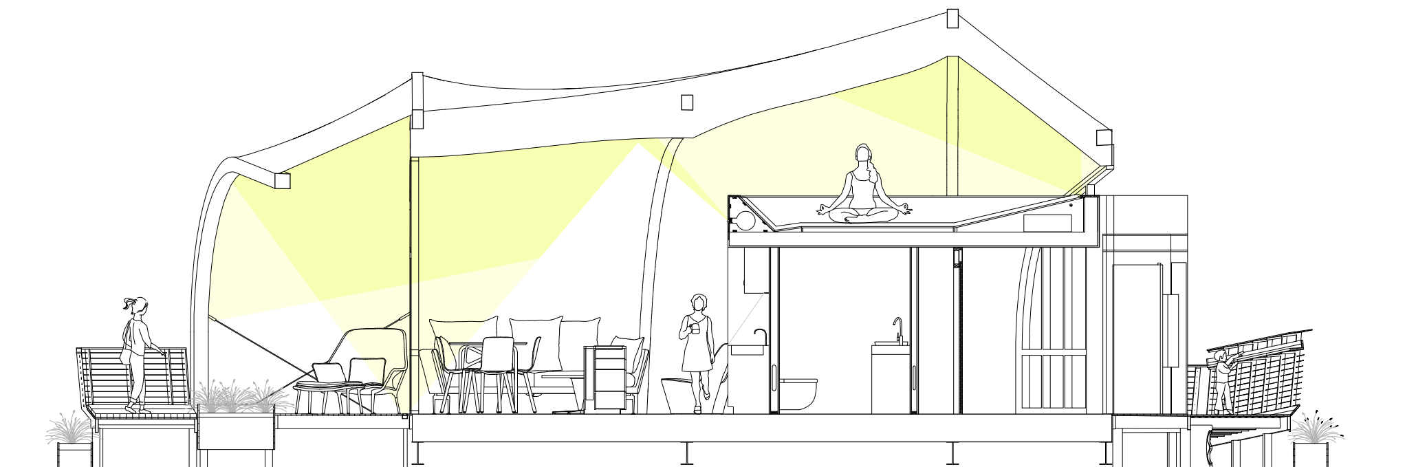
1 LIGHTING DIAGRAM LONGITUDINAL SECTION
