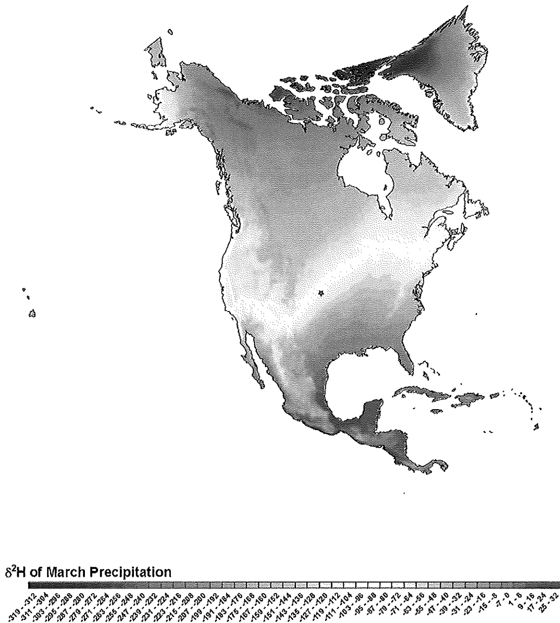
Figure 6. Spatial distribution of deuterium in precipitation for the month of March according to Bowen (2009). Deuterium isotopes fall in a known precipitation gradients across the United States. Regions that fall into the light orange/yellow (-80 to -87 gradient) are approximate to the values reflected in the Black Rail body covers. The star denotes the approximate location of the study site.
