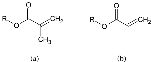
Figure 1. Structure of (a) methacrylate and (b) acrylate vinyl ester functional groups.
