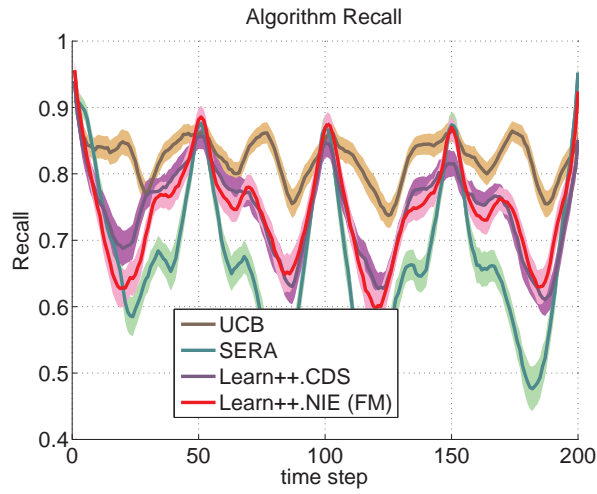
(e) Recall
