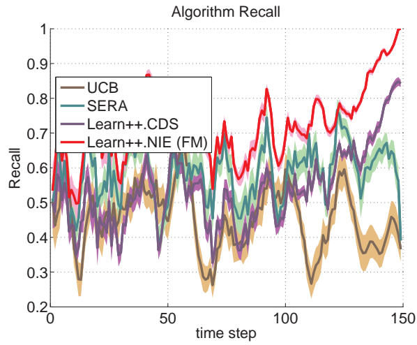
(e) Recall
