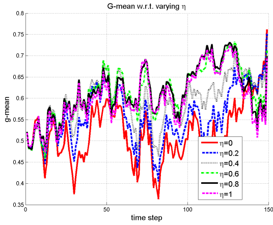
(c) G-mean
