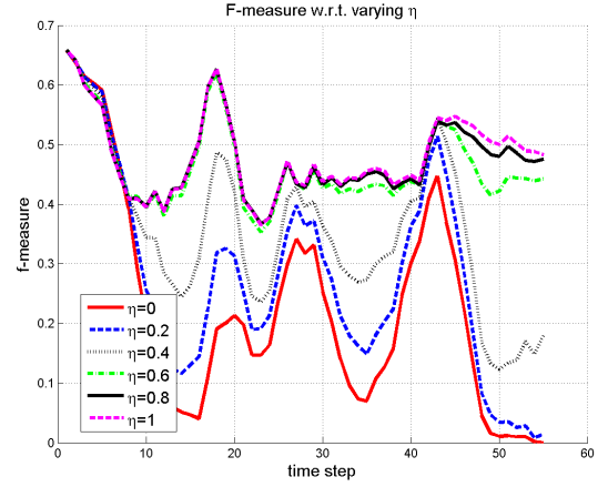
(b) F-measure
