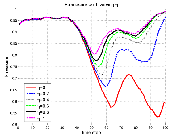
(b) F-measure
