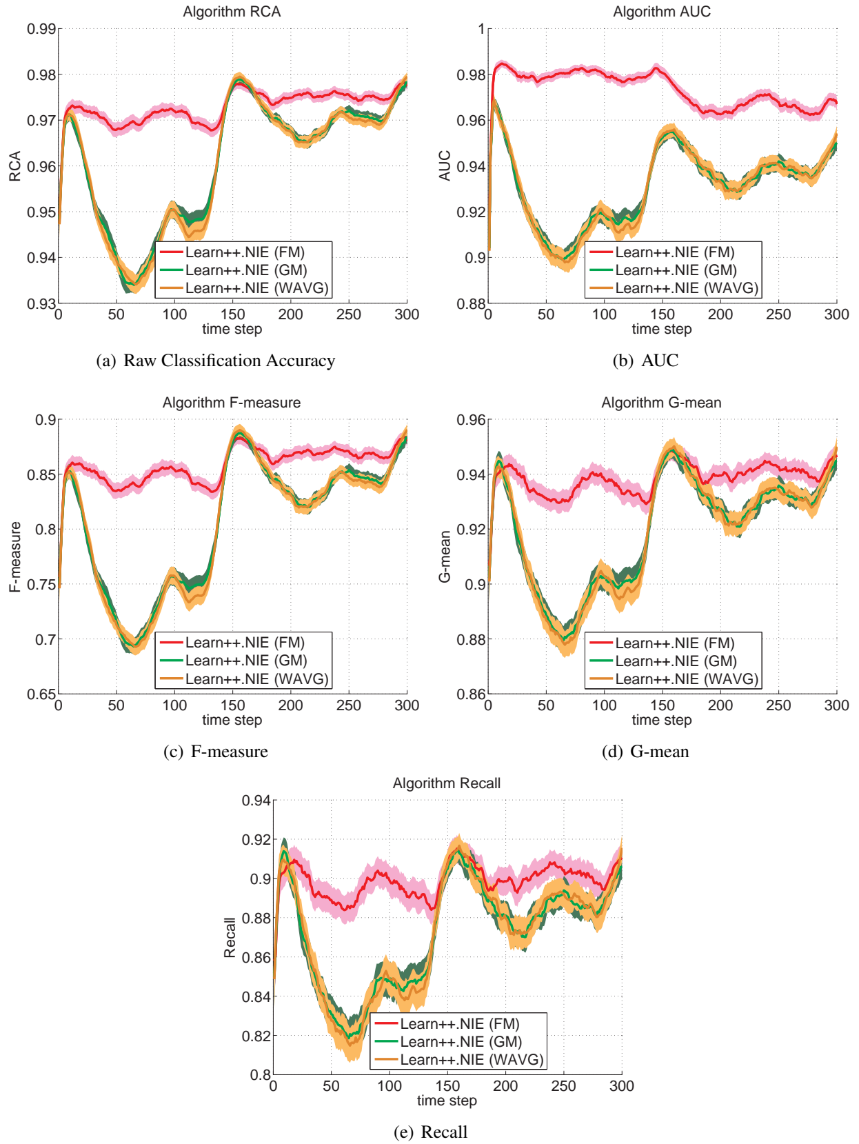
Fig. 5.15 : Learn++.NIE family of algorithms evaluated on Spiral Data
