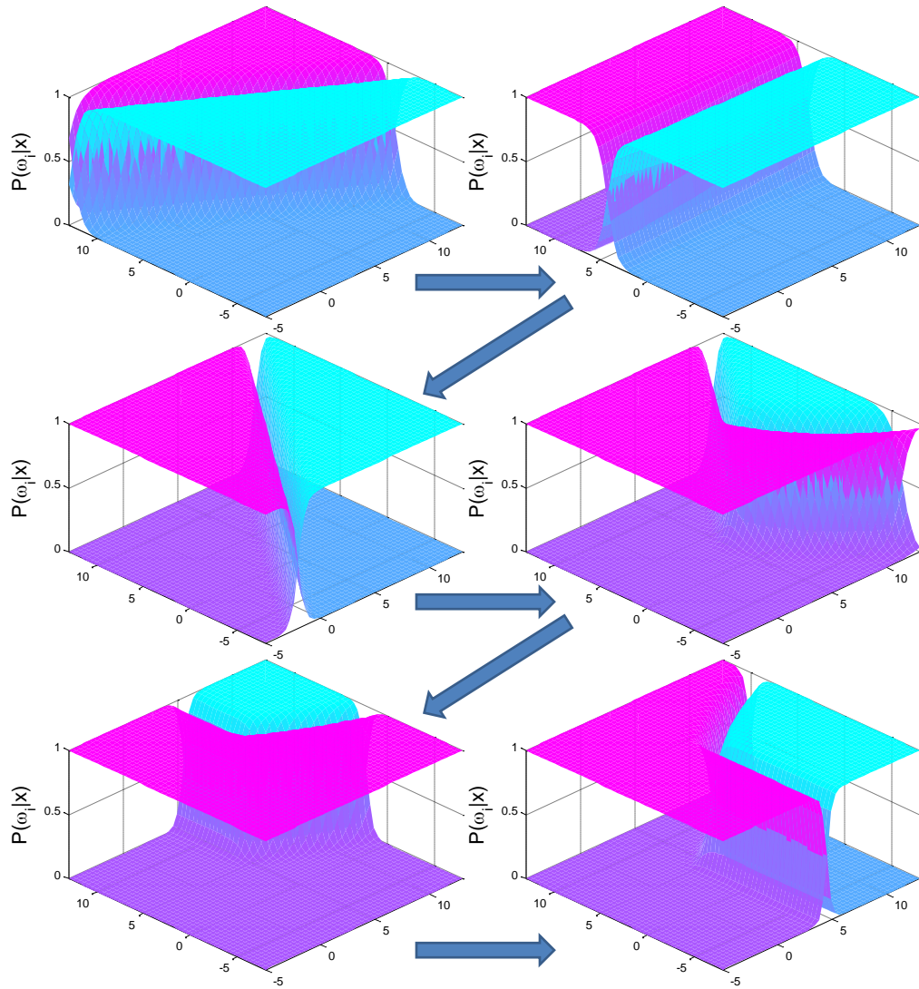
Fig. 5.45 : Evolution of the RandGauss dataset by observing the posterior probability. The dataset begins with 2-modes (one for each class) and begin slowly drifting. The drift stops at the third evolution point and remains static for 25 time stamps followed by the introduction of a new mode for the magenta class. The dataset continues to evolve with slow change followed by abrupt changes.
