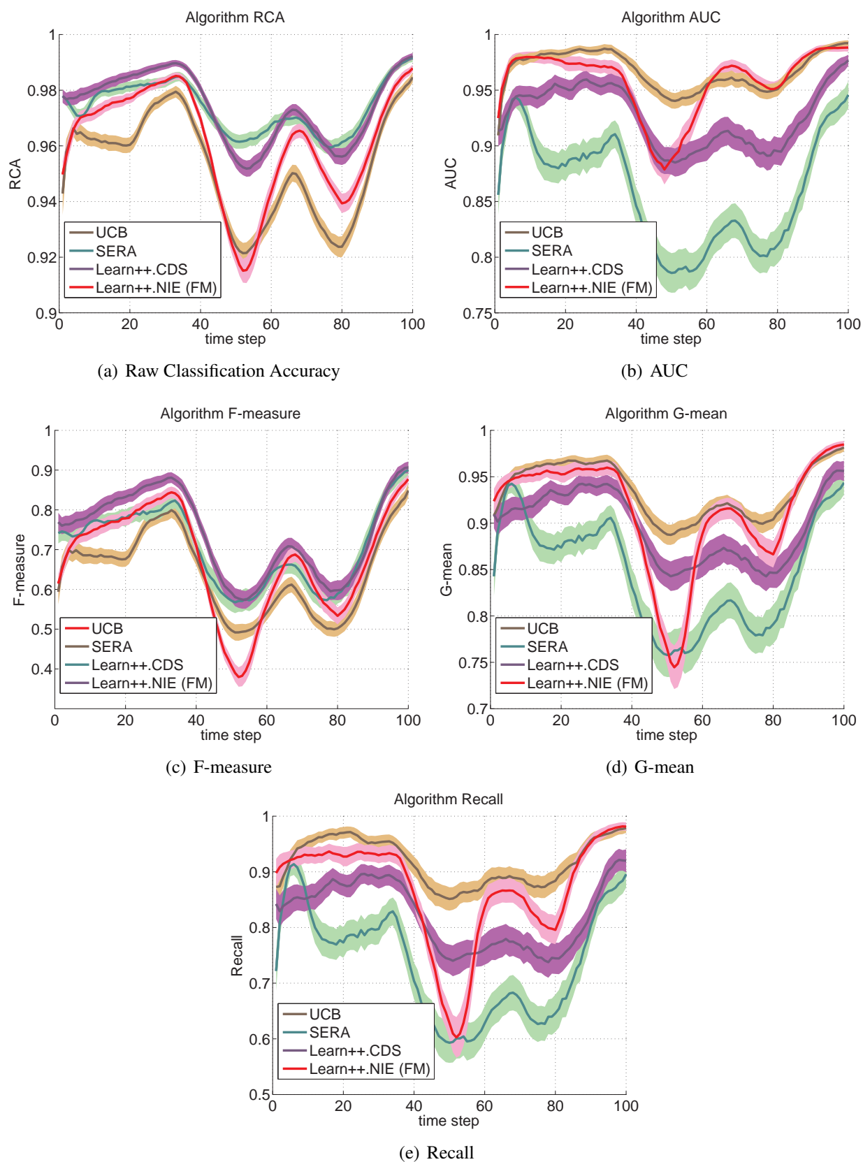
Fig. 5.21 : Baseline algorithms evaluated on Gaussian data
