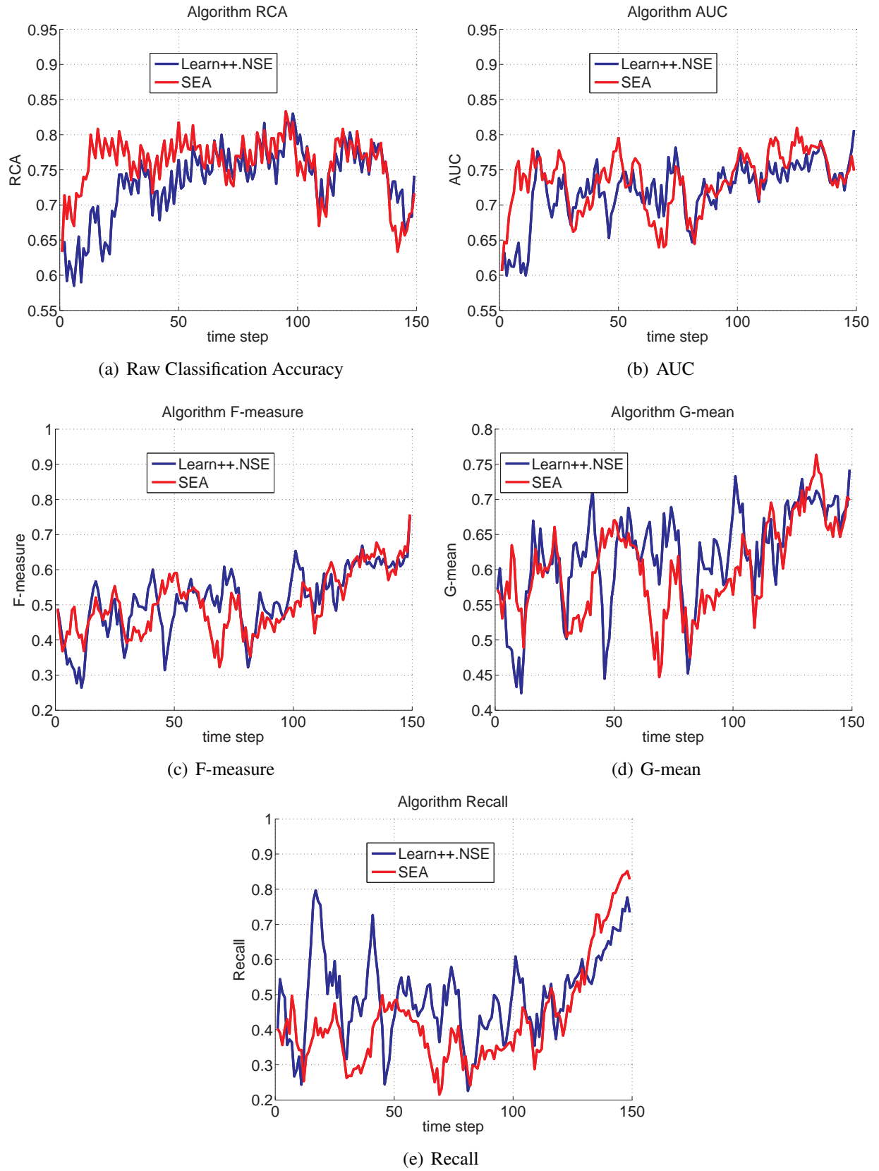
Fig. 5.34 : Learn ++ .NSE and SEA evaluated on the NOAA Dataset
