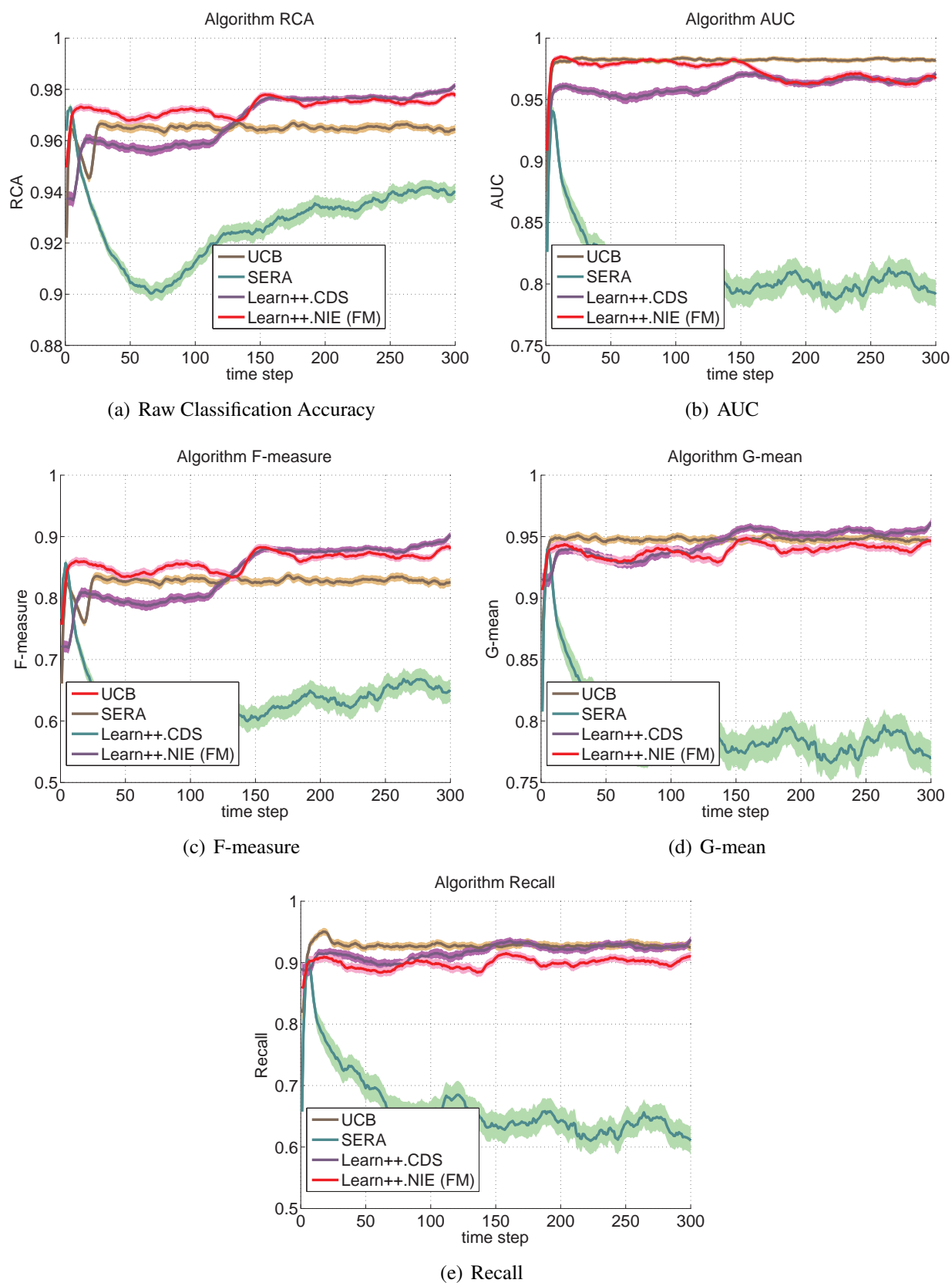
Fig. 5.16 : Baseline algorithms evaluated on Spiral Data
