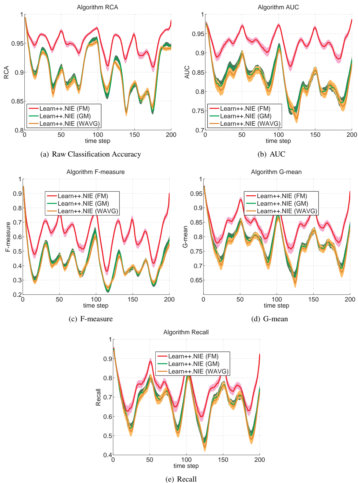
Fig. 5.9 : Learn ++ .NIE family of algorithms evaluated on Checkerboard data
