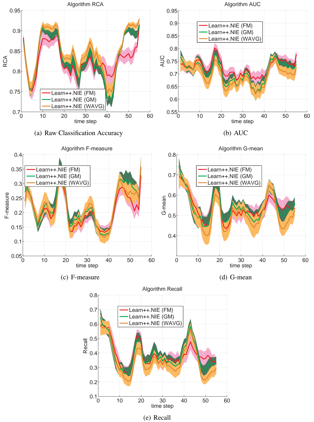
Fig. 5.30 : Learn ++ .NIE family of algorithms evaluated on the Elec2 Dataset
