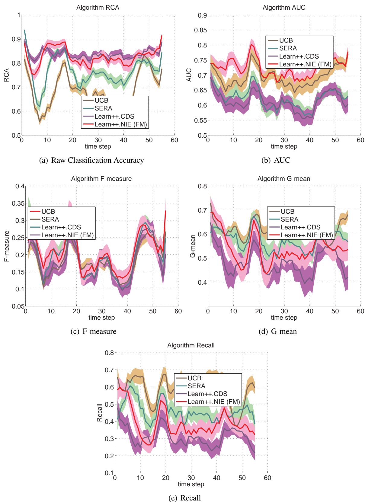
Fig. 5.31 : Baseline algorithms evaluated on the Elec2 Dataset
