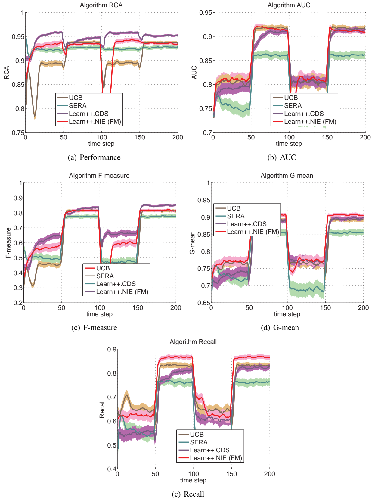
Fig. 5.26 : Baseline algorithms evaluated on a Shifting Hyperplane Dataset
