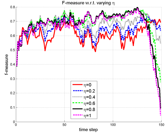
(b) F-measure
