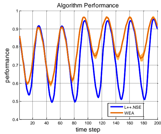
(e) Bias=7
