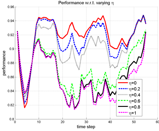
(a) Performance
