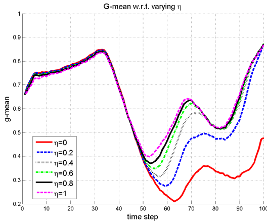
(c) G-mean
