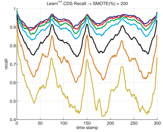
(b) SMOTE(%)=200
