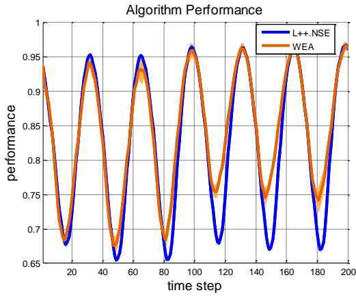
(c) Bias=3
