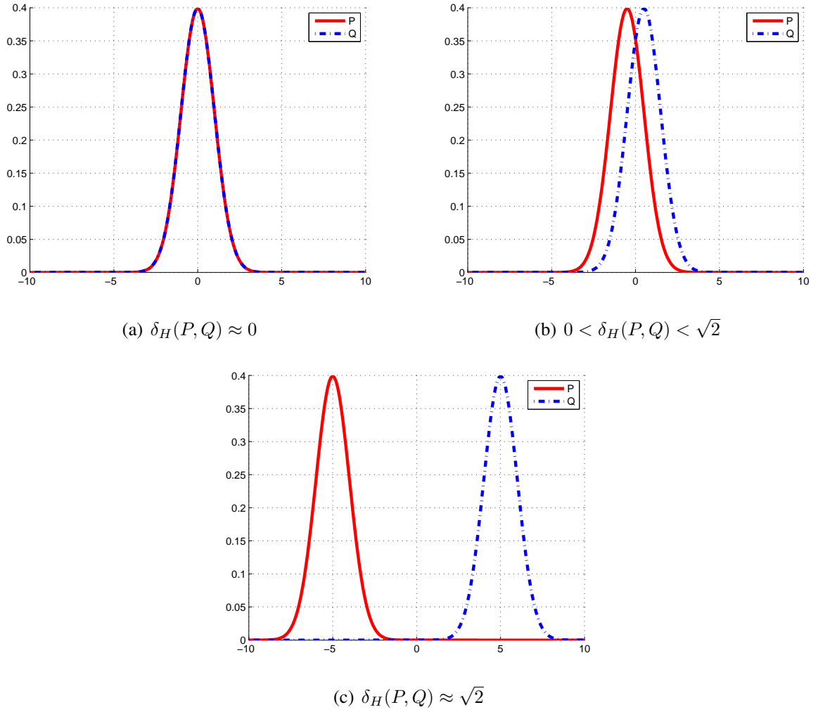
Fig. 4.5 : Hellinger distance computed between two probability distributions P and Q .
