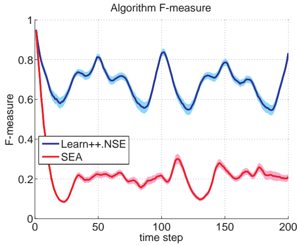
(i) F-measure
