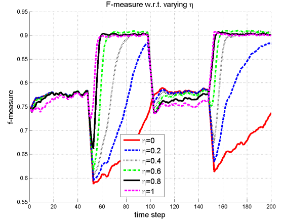
(b) F-measure
