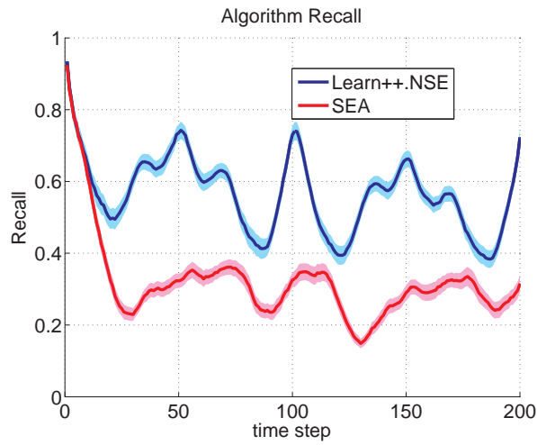
(k) Recall
