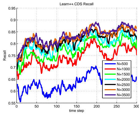
(e) Recall
