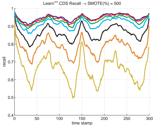
(c) SMOTE(%)=500
