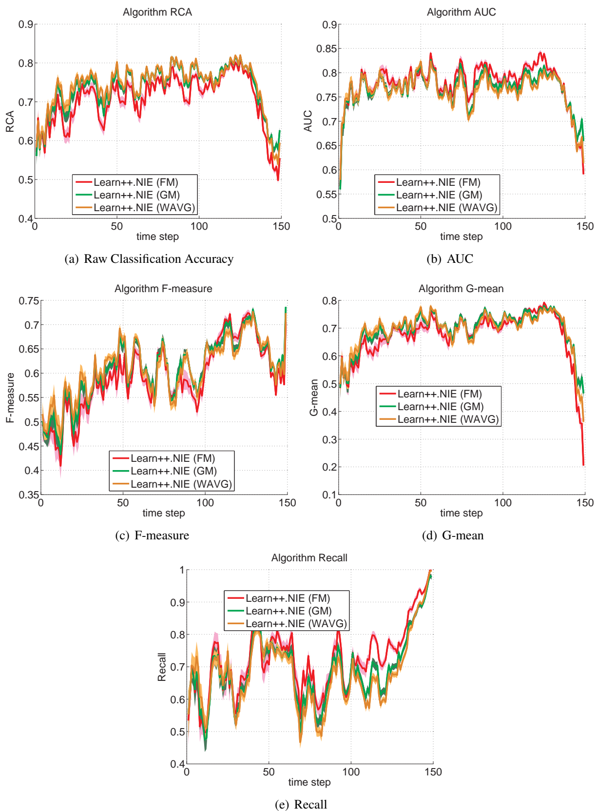
Fig. 5.35 : Learn ++ .NIE family of algorithms evaluated on the NOAA Dataset
