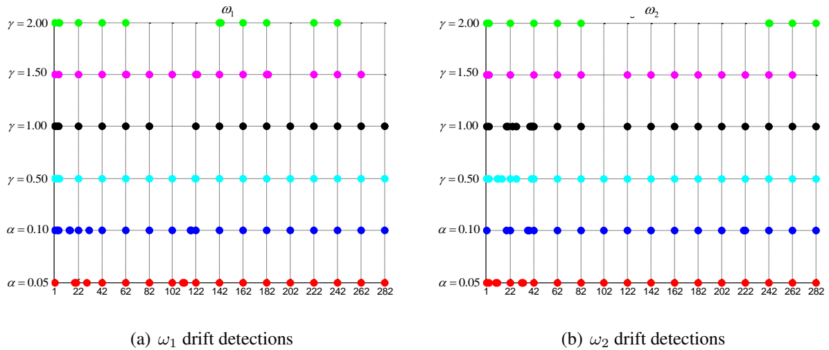
Fig. 5.48 : Drift detection locations for the rotating checkerboard problem with abrupt points of change for \omega_1 (Fig. 5.48(a)) and \omega_2 (Fig. 5.48(b))
