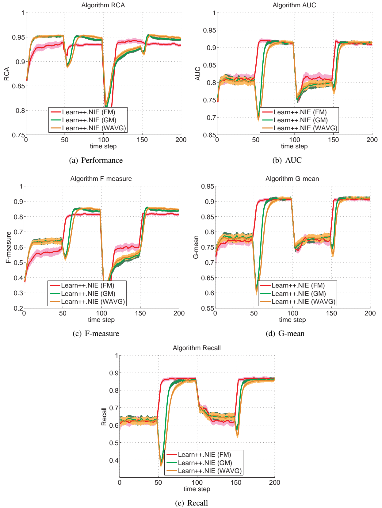
Fig. 5.25 : Learn ++ .NIE family of algorithms evaluated on a Shifting Hyperplane Dataset
