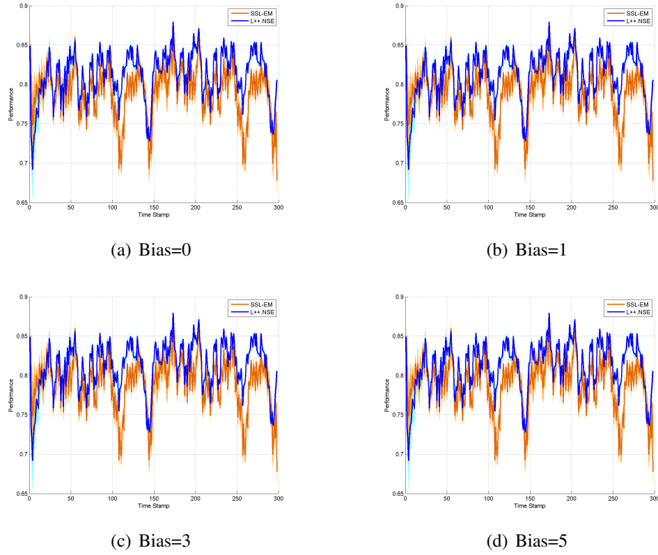
Fig. 5.42 : WEA vs. Learn ++ .NSE on NOAA Dataset
