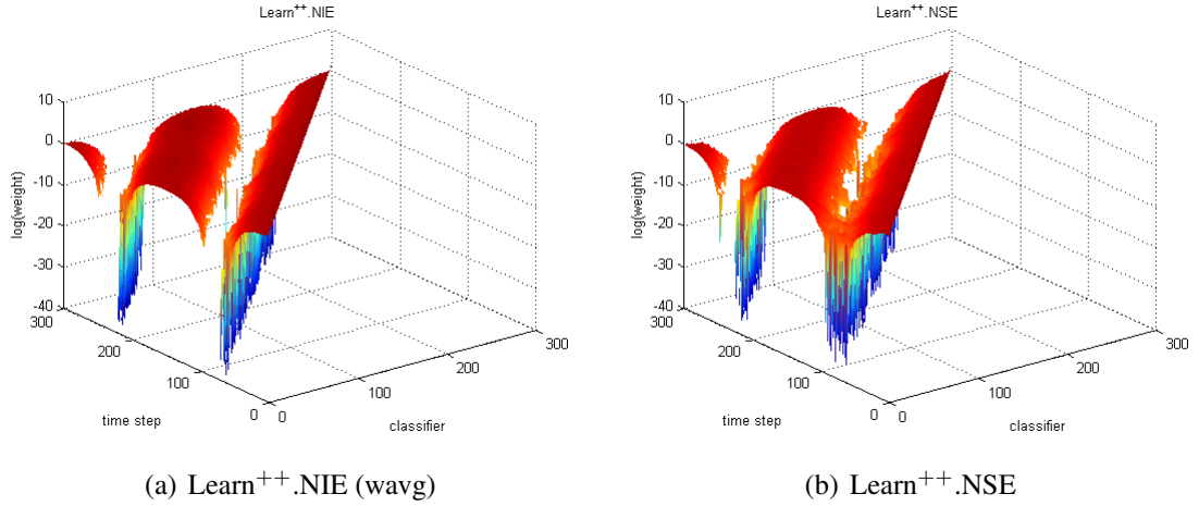
Fig. 5.17 : Learn ++ weight evolution on Spiral Data
