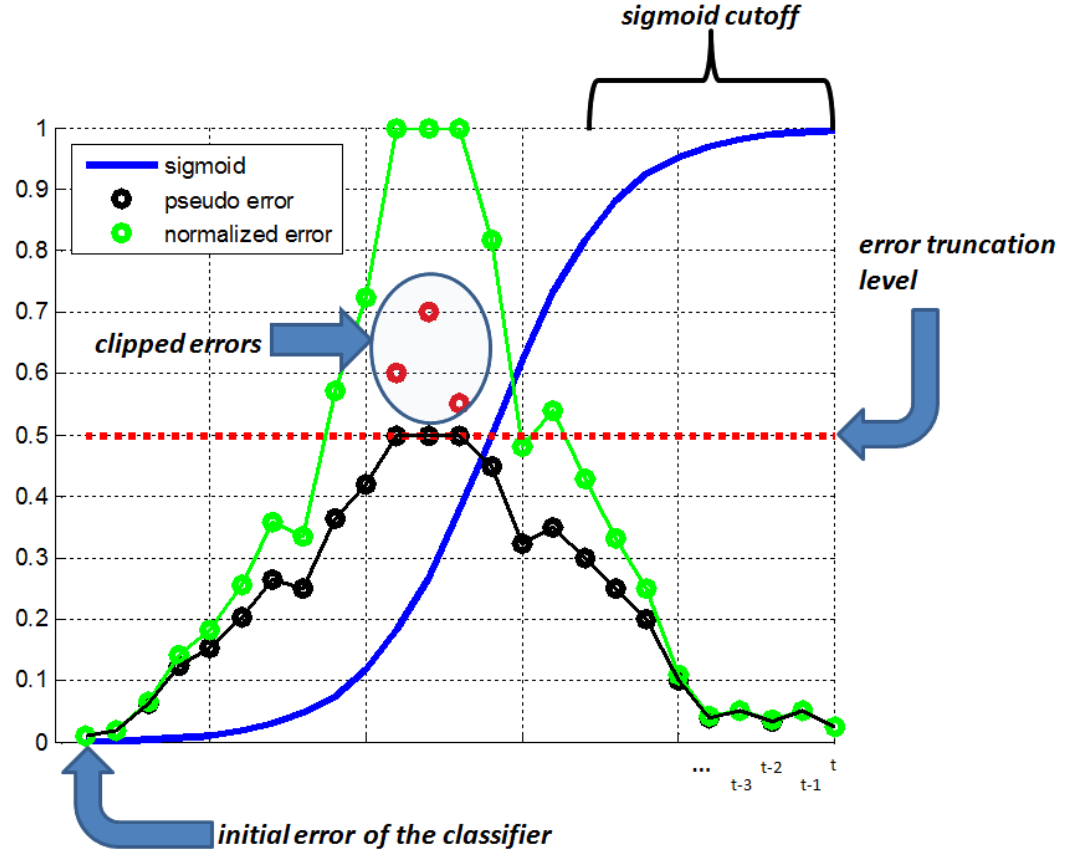
Fig. 3.19 : The more recent errors of a classifier are weighted heavier than errors ( \beta_k^{(t)} ) that have been committed a long time ago as indicated by the magnitude of the logistic function through time ( \sigma_k^{(t)} )
