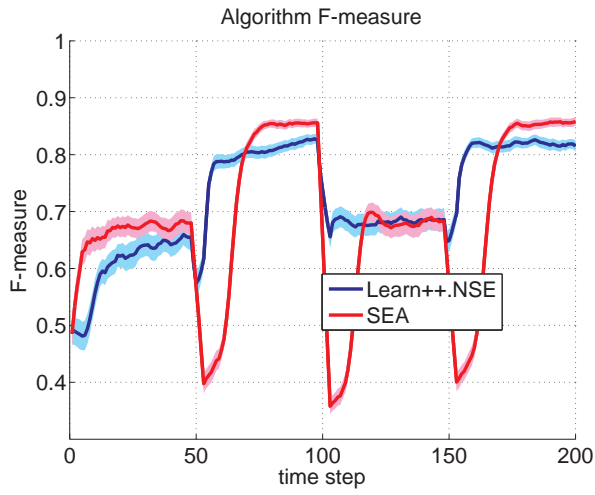
(c) F-measure
