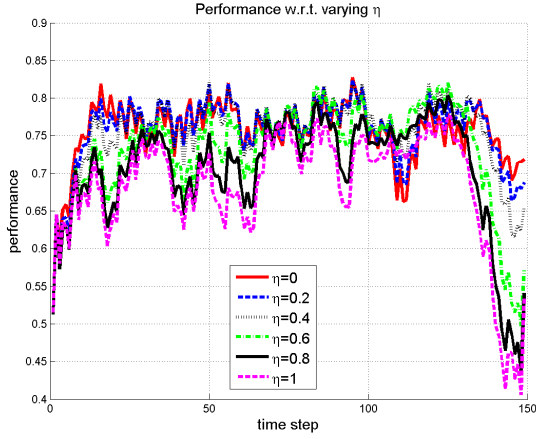
(a) Performance
