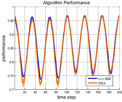
(a) Bias=0
