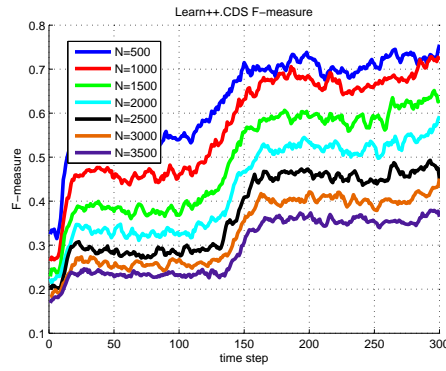
(c) F-measure
