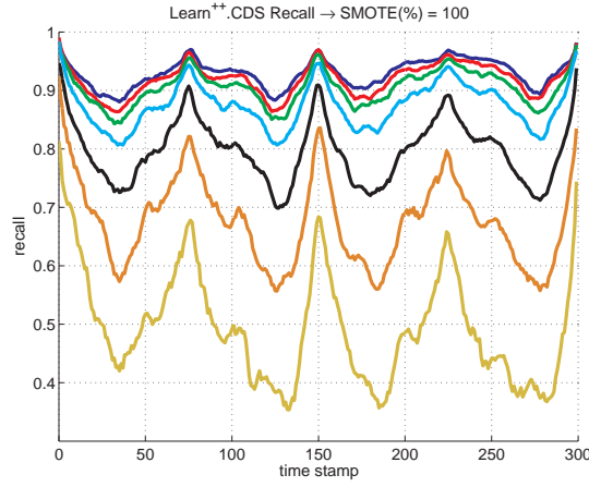
(a) SMOTE(%)=100
