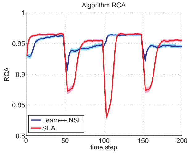
(a) Performance
