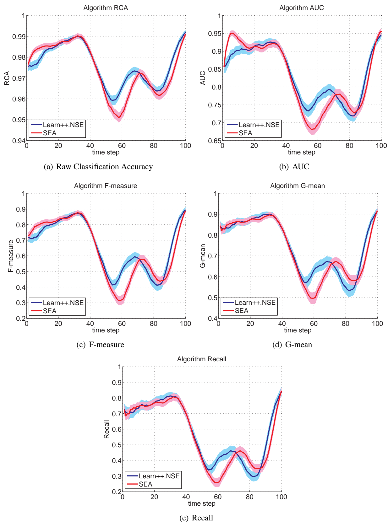
Fig. 5.19 : \text{Learn}^{++}.\text{NSE} and SEA evaluated on Gaussian data
