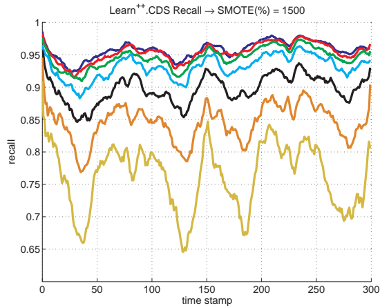
(e) SMOTE(%)=1500
