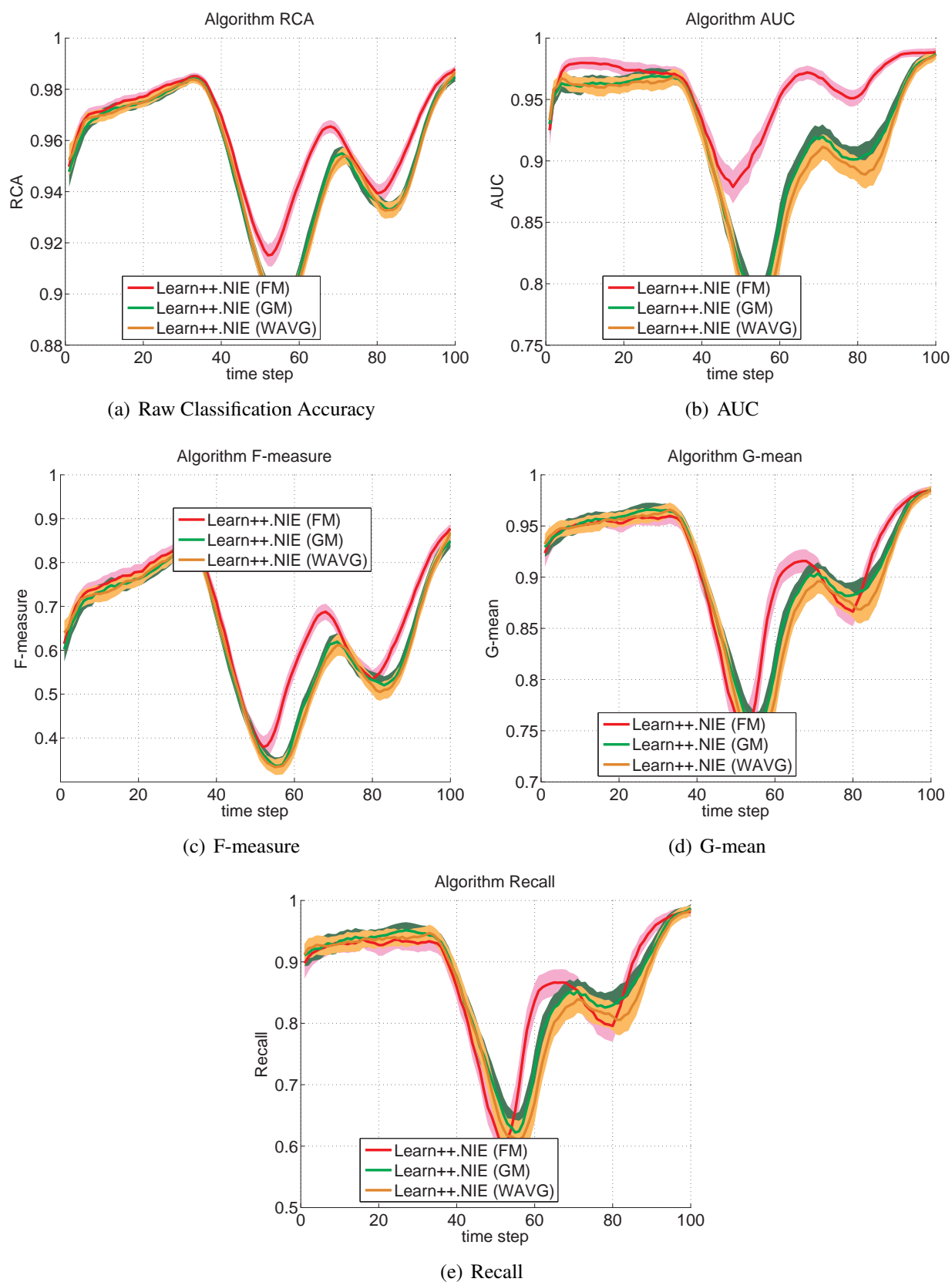
Fig. 5.20 : Learn ++ .NIE family of algorithms evaluated on Gaussian data
