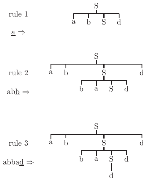
Figure 4.4: Using the input symbol to guide the parsing of the string abadd
