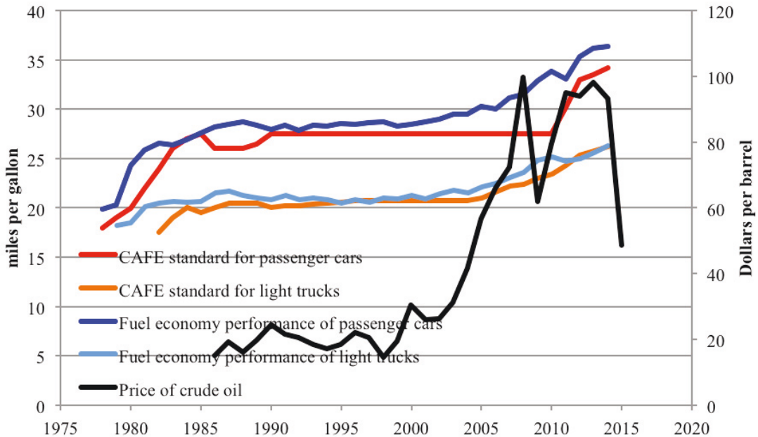
Fig. 1. CAFE requirement for fleet economy together with average fuel economy performance in the U.S. between 1978-2014. The price of crude oil has also been plotted for comparison. [29, 30]
