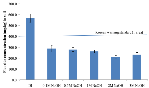
Fig. 4 Fluoride concentrations remaining in the soil after sodium hydroxide (NaOH) washing
