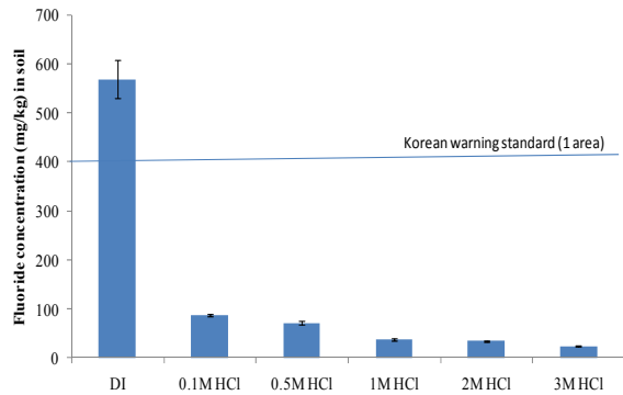
Fig. 1 Fluoride concentrations remaining in the soil after hydrochloric acid (HCl) washing
