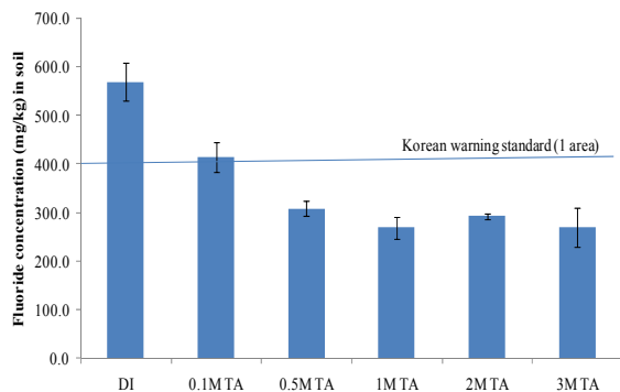
Fig. 5 Fluoride concentrations remaining in the soil after tartaric acid (C 4 H 6 O 6 ) washing
