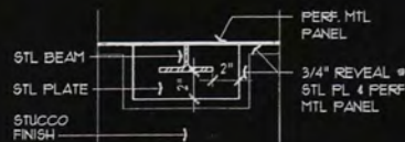
6 Elevation - Beam Penetration @ Canopy A301 SCALE: 1/8"=1'-0"
