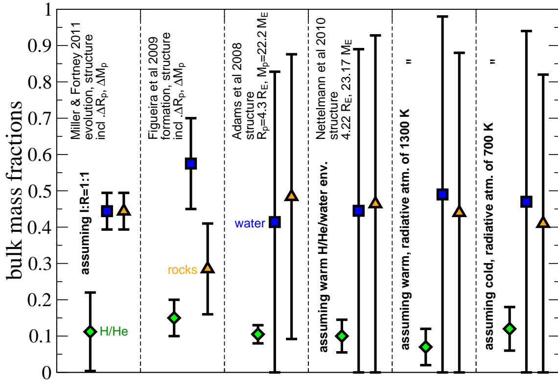
FIG. 18.— Constraints on the bulk composition of GJ 436b as determined from models of its structure, evolution, and formation. Possible compositions are shown for six different model assumptions and/or imposed constraints. For each, the sum over the displayed mass fractions of H/He (green diamonds), water (blue squares), and “rock” (includes silicates plus iron; orange triangles) equals 1. All calculations take into account the planet’s mass M_p and radius R_p as one set of constraints; the two leftmost models consider uncertainties in M_p and R_p , while the four on the right adopt specific M_p and R_p values from Torres et al. (2008). From left to right, the derived constraints are based on (i) the thermal and structural evolution models of Miller & Fortney (2011) that assume an ice:rock ratio of 1:1 and that impose constraints based on the age of the GJ 436 system; (ii) the formation, disk-planet evolution (including migration), and structural models of Figueira et al. (2009) that compute various formation paths consistent with M_p and R_p ; (iii) the structure models of Adams et al. (2008) that consider precise values for M_p , R_p , and atmospheric temperatures; (iv) the structural models of Nettelmann et al. (2010) that assume that water is mixed into the outermost H/He envelope; (v) structural models based on Nettelmann et al. (2010) that assume that a pure H/He layer resides above a water layer with a warm (1300 K) deep isothermal radiative region; (vi) a model similar to the one on the immediate left, except the isothermal radiative region is cool (700 K) and the planet is old ( > 10 Gyr). Note that the tightest constraints on the composition are imposed by the formation models, that including the uncertainties in M_p and R_p enhance the uncertainty in the H/He mass fraction by a factor of \sim 2 , and that assumptions about atmospheric temperatures affect the derived H/He mass fraction. A color version of this figure is available in the online journal.
