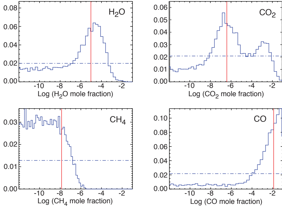
FIG. 9.— Gas mole-fraction histograms of the marginalized posterior probability distribution derived from the differential-evolution Markov-chain Monte-Carlo retrieval approach (Line et al. 2013), as applied to the GJ 436b Spitzer eclipse data of Stevenson et al. (2010). The horizontal dot-dashed blue curves represent the priors, which are assumed to be flat (uninformative). The vertical red lines represent the mole fractions that correspond to the best-fit solution. A color version of this figure is available in the online journal.
