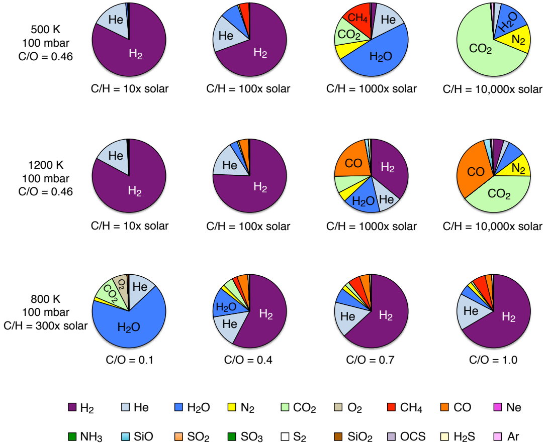
FIG. 4.— Pie charts illustrating equilibrium gas-phase compositions on generic hot Neptunes for different assumptions about atmospheric properties. The top row shows variations as a function of metallicity (10-10,000 times solar, as labeled) for an atmosphere with a solar C/O ratio, a pressure of 100 mbar, and a temperature of 500 K. The middle row is similar to the top row, except the assumed temperature is 1200 K. The bottom row shows variations as a function of the C/O ratio for an assumed metallicity of 300 times solar (i.e., protosolar abundances of all species except H, He, Ne, and O are multiplied by 300, with O being defined through the C/O ratio), a pressure of 100 mbar, and a temperature of 800 K. Note the very large variation in composition for different bulk atmospheric properties. A color version of this figure is available in the online journal.
