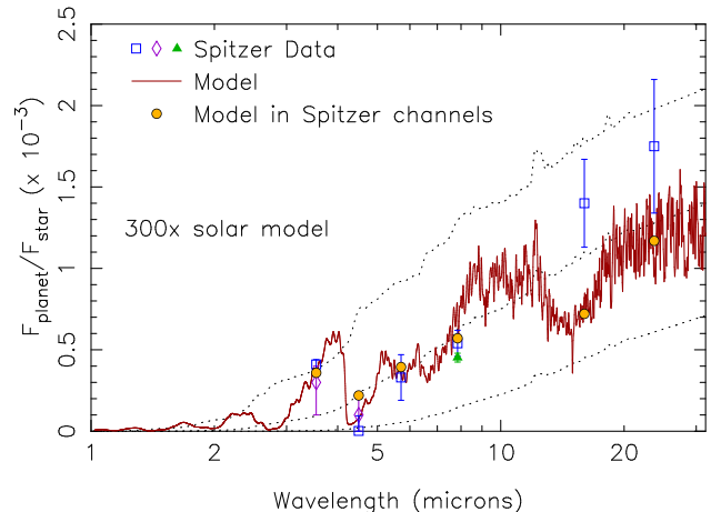
FIG. 16.— Synthetic emission spectra (dark red) for GJ 436b for our disequilibrium model that assumes a 300\times solar metallicity atmosphere, with a C/O ratio of 0.6 (see text and Fig. 15). The blue squares represent the Spitzer secondary-eclipse data analyzed by Stevenson et al. (2010), with an updated upper limit at 4.5\text{-}\mu\text{m} from Stevenson et al. (2012), the purple diamonds represent the the 3.6 and 4.5\text{-}\mu\text{m} Spitzer analysis of Beaulieu et al. (2011), and the green triangle represents additional Spitzer eclipse data at 8\text{-}\mu\text{m} as analyzed by Knutson et al. (2011). The red circles represent the model fluxes averaged over the Spitzer bandpasses. The black dotted lines represent the planetary emission assuming GJ 436b radiates as a blackbody at a temperature of 500 K (lower curve), 800 K (middle curve), or 1100 K (upper curve). See Fig. 14 for further details. A color version of this figure is available in the online journal.
