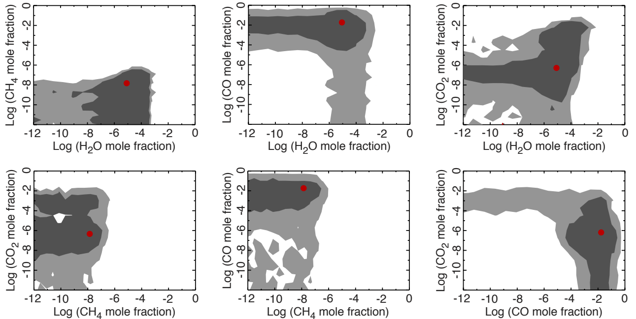
FIG. 10.— Contours of the gas-abundance constraints for GJ 436b derived from the differential-evolution MCMC posterior probability distributions, illustrating the correlations between the different gases. The dark gray regions represent the 1-sigma confidence interval and light gray regions represent the 2-sigma confidence interval. The red dot in each plot is the best-fit (maximum-likelihood) solution from the ensemble of 10^5 fits. A color version of this figure is available in the online journal.
