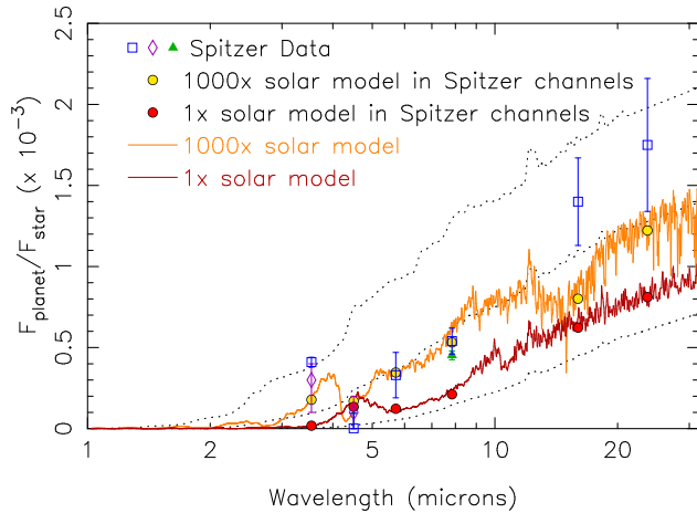
FIG. 14.— Synthetic emission spectra for GJ 436b for our disequilibrium models that assume a 1\times solar metallicity atmosphere (dark red) and a 1000\times solar metallicity atmosphere (orange), in comparison with observations (data points with error bars). The thermal profiles assumed in the models are shown in Fig. 1, and the abundance profiles are shown in Fig. 13. The blue squares represent the Spitzer secondary-eclipse data analyzed by Stevenson et al. (2010), with an updated upper limit at 4.5\text{-}\mu\text{m} from Stevenson et al. (2012), the purple diamonds represent the Beaulieu et al. (2011) analysis of the same 3.6 and 4.5\text{-}\mu\text{m} data, and the green triangle represents the analysis of 11 secondary eclipses of GJ 436b in the 8\text{-}\mu\text{m} channel by Knutson et al. (2011). The red and gold circles represent, respectively, the fluxes from the 1\times and 1000\times solar models, averaged over the Spitzer bandpasses. The black dotted lines represent the planetary emission (smoothed) assuming GJ 436b radiates as a blackbody at a temperature of 500 K (lower curve), 800 K (middle curve), or 1100 K (upper curve). The apparent emission “spikes” represent stellar absorption, as everything here is plotted in terms of the flux of the planet divided by the flux of the star. A PHOENIX stellar model (e.g., Hauschildt et al. 1999) with T_{\text{eff}} = 3350 K was assumed for the host star for all these calculations. A color version of this figure is available in the online journal.
