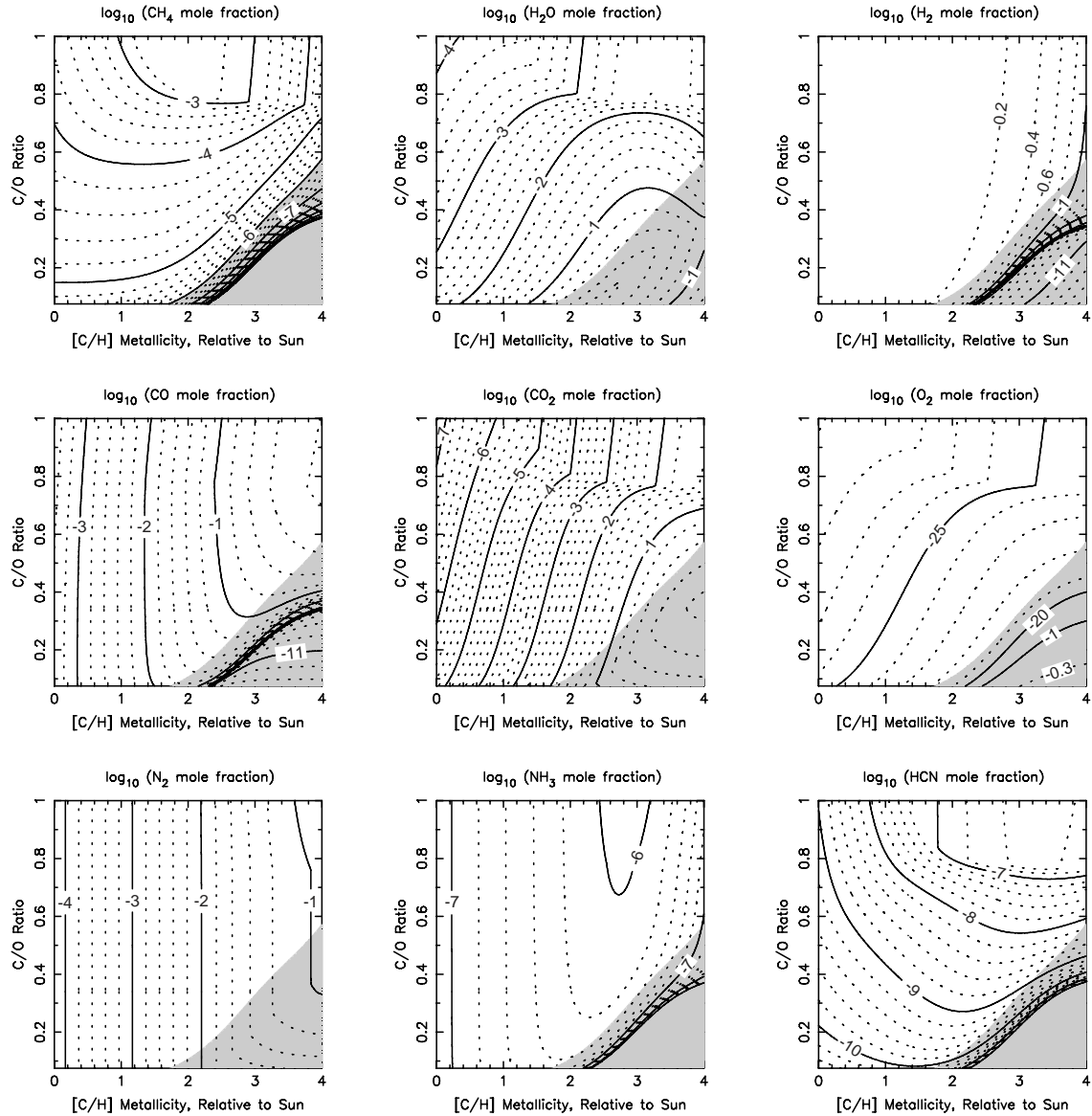
FIG. 11.— Equilibrium mole fractions for different species as a function of C/H metallicity (see text) and C/O ratio at 900 K and 10 mbar (i.e., a relatively hot, high-altitude photosphere, which may be relevant to a high-metallicity GJ 436b). The shaded region in each plot is where methane has a mole fraction below 10^{-6} , as indicated by retrievals based on the Stevenson et al. (2010) Spitzer GJ 436b secondary-eclipse data (our work, and that of Madhusudhan & Seager 2011).
