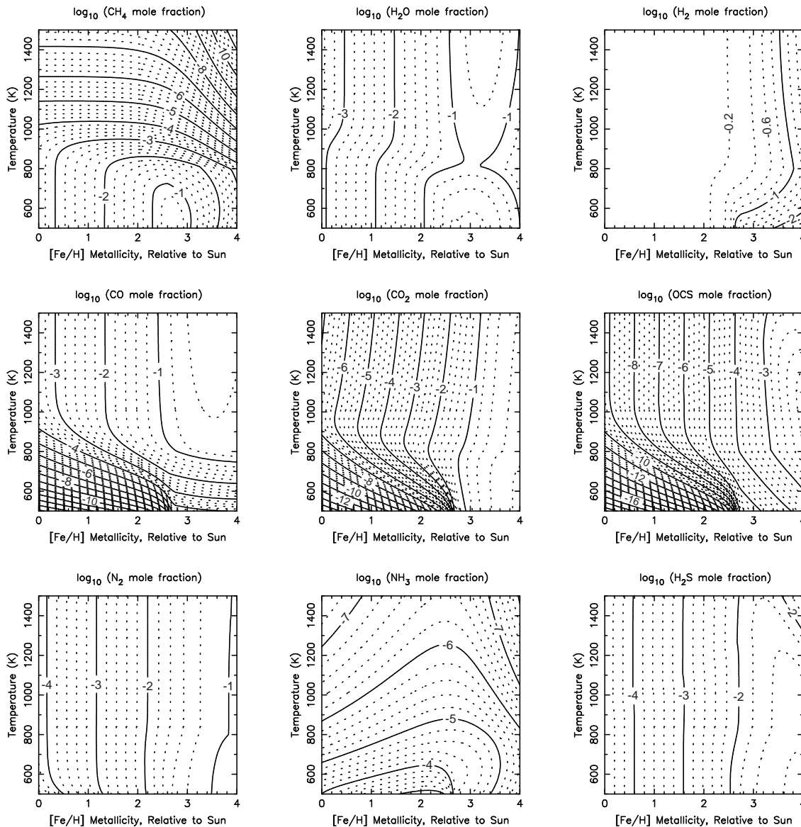
FIG. 5.— Equilibrium mole fractions for different gas-phase species as a function of temperature and metallicity for a solar ratio of elements (except H, He, and Ne remain solar at all metallicities), at a pressure of 100 mbar. When we present a metallicity [X/H] in square brackets here and in subsequent figures, we use the standard logarithmic definition; e.g., a metallicity of [Fe/H] = 3 corresponds to a heavy element enrichment of 1000\times solar.
