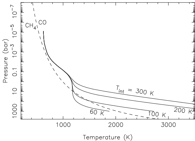
FIG. 2.— Theoretical thermal profiles for GJ 436b assuming different values for the intrinsic internal heat flux F_{int} = \sigma T_{int}^4 , from 1-D, 50\times solar metallicity, inefficient heat redistribution calculations that are based on the models of Fortney et al. (2006, 2007).
