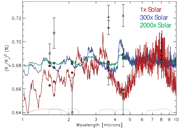
FIG. 17.— Synthetic transmission spectra for GJ 436b (in terms of the apparent transit depth, i.e., the square of the ratio of the planetary radius to the stellar radius) for our disequilibrium models that assume a 1\times (red), 300\times (blue), and 2000\times (green) solar metallicity. Scattering from molecules or hazes is not included in the calculations. Data points from various sources are shown in black, with associated error bars. In order of increasing wavelength, the squares are from the 1.1\text{--}1.9\text{ }\mu\text{m} HST/NICMOS analysis of Pont et al. (2009) plotted at 1.5\text{ }\mu\text{m} ; the ground-based H -band data of Alonso et al. (2008) plotted at 1.6\text{ }\mu\text{m} ; the ground-based K_s band data of Cáceres et al. (2009) plotted at 2.1\text{ }\mu\text{m} , as discussed by Knutson et al. (2011); and the Spitzer /IRAC analysis of Knutson et al. (2011) plotted at 3.6 , 4.5 , and 8\text{ }\mu\text{m} . The diamonds are from the Spitzer analysis of Beaulieu et al. (2011) at 3.6 , 4.5 , and 8\text{ }\mu\text{m} . The triangles are the Spitzer transits at 3.6 and 4.5\text{ }\mu\text{m} that Knutson et al. (2011) suggest are influenced by the occultation of star spots or other regions of non-uniform brightness on the star. The black dotted curves at the bottom show the response functions for the filters and/or detector channels used in the observations. The colored circles represent the corresponding model transit depths averaged over the appropriate filters/channels. A color version of this figure is available in the online journal.
