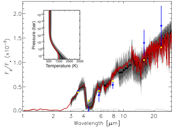
FIG. 8.— Synthetic emission spectra (flux of the planet divided by flux of the star) and thermal profile (insert) for GJ 436b derived from the differential-evolution Markov-chain Monte-Carlo retrieval method described by Line et al. (2013). The span of solutions that fit within 2-sigma (light gray) and 1-sigma (dark gray) are shown in both the temperature-profile and spectral plots, along with the median of the ensemble of fits (black curves). The red curves in both plots represent a single best-fit model. The blue diamonds with error bars are the Spitzer secondary-eclipse photometric data from Stevenson et al. (2010), and the yellow circles show the best-fit model results convolved over the Spitzer bandpasses (with the bandpass sensitivities being plotted as dotted curves near the bottom of the plot). A color version of this figure is available in the online journal.
