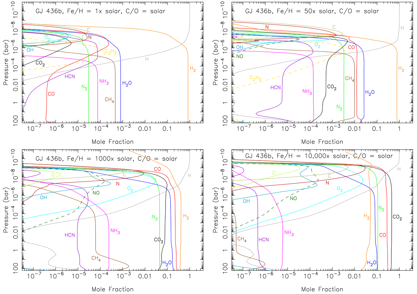
FIG. 13.— Mixing-ratio profiles for several species of interest (as labeled) in our kinetics/transport models for GJ 436b, for assumed atmospheric metallicities of 1\times solar (top left), 50\times solar (top right), 1000\times solar (bottom left), and 10,000\times solar (bottom right). The thermal profiles adopted in these models are described in section 2.2 (see Fig. 1); the profile for the 10,000\times solar model (not shown in Fig. 1) was derived from the PHOENIX model (Hauschildt et al. 1999; Allard et al. 2001; Barman et al. 2005) and is very similar to the 1000\times solar profile. The C/O ratio is assumed to be the protosolar value of Lodders et al. (2009) with 21% of the oxygen unavailable due to being bound up in condensates at deep atmospheric levels (Visscher et al. 2010a), and the eddy diffusion coefficient K_{zz} is assumed to be constant at 10^9 \text{ cm}^2 \text{ s}^{-1} . A color version of this figure is presented in the online journal.
