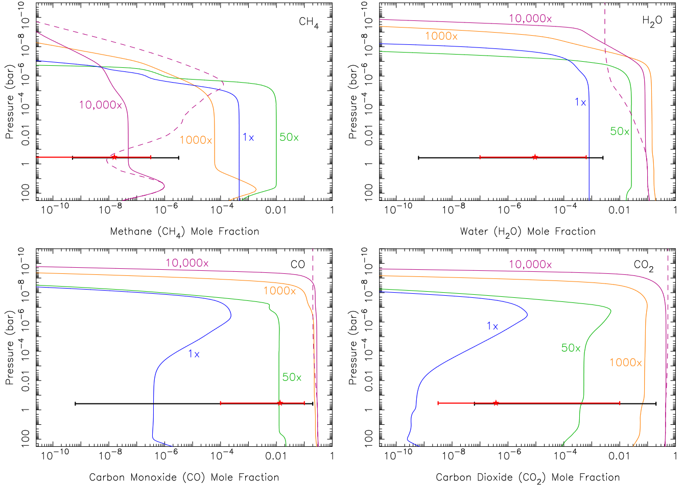
FIG. 12.— Mixing-ratio profiles for \text{CH}_4 (top left), \text{H}_2\text{O} (top right), \text{CO} (bottom left), and \text{CO}_2 (bottom right) from our kinetics/transport models for GJ 436b, for assumed atmospheric metallicities of 1\times solar (blue solid lines), 50\times solar (green solid lines), 1000\times solar (orange solid lines), and 10,000\times solar (purple solid lines), as described more fully in Fig. 13. The corresponding equilibrium solutions for the 10,000\times solar model are shown as dashed purple lines. The red horizontal bar illustrates the most-probable solutions derived from the differential-evolution MCMC approach discussed in section 3.2, with the star representing the best-fit solution. The black horizontal bar represents the model solutions from Madhusudhan & Seager (2011) that fit the Spitzer data to within \chi^2/N_{\text{obs}} \leq 1 . Note that none of the disequilibrium models for the different metallicities have mole fractions that fall within the retrieval constraints for all four species. A color version of this figure is presented in the online journal.
