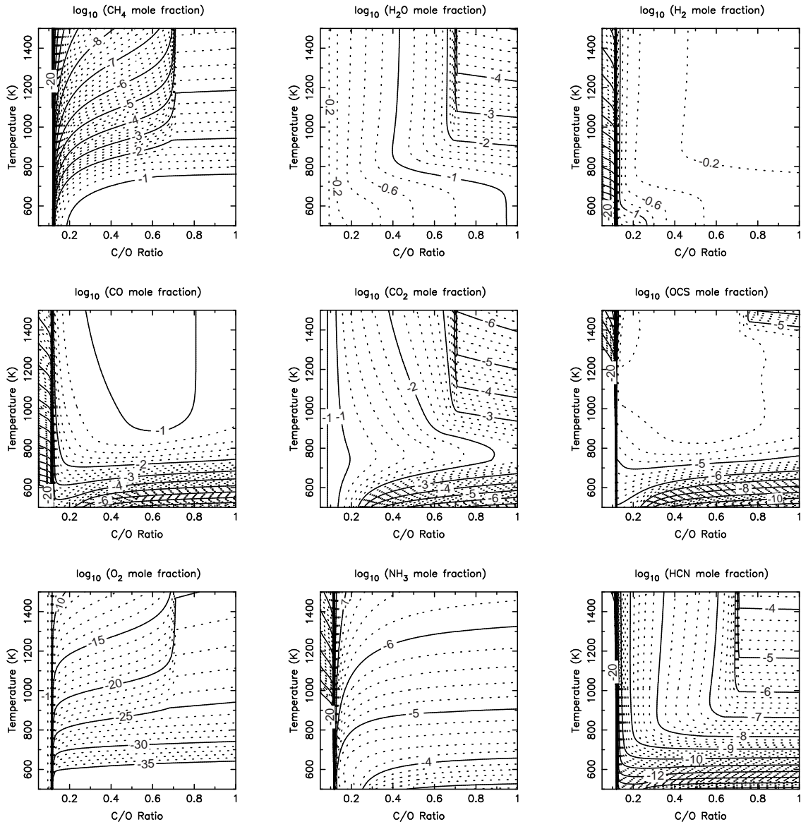
FIG. 6.— Equilibrium mole fractions for different gas-phase species as a function of temperature and C/O ratio for a 100-mbar pressure and a metallicity X/H = 300 \times solar (where X represents all elements except H, He, Ne, and O, with the O abundance being defined through the C/O ratio).
