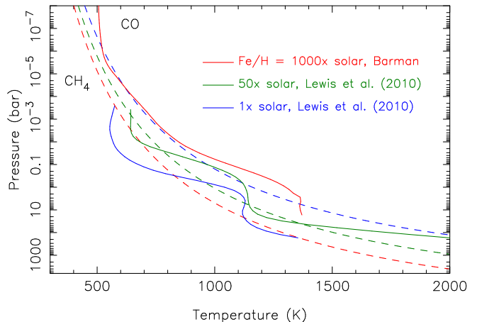
FIG. 1.— Theoretical thermal profiles (solid lines) for GJ 436b assuming various atmospheric metallicities. The profiles for 1× solar metallicity (blue) and 50× solar metallicity (green) are the atmospheric temperatures averaged over the dayside of GJ 436b at secondary-eclipse conditions from the GCMs of Lewis et al. (2010); the profile for 1000× solar metallicity (red) is from a 1-D, inefficient-heat-redistribution calculation based on Barman et al. (2005). The dashed lines represent the boundaries where CH 4 and CO have equal abundances in chemical equilibrium for the different metallicity models, with the color coding remaining the same as for the thermal profiles. Methane dominates to the lower left of these curves, and CO dominates to the upper right. A color version of this figure is available in the online journal.
