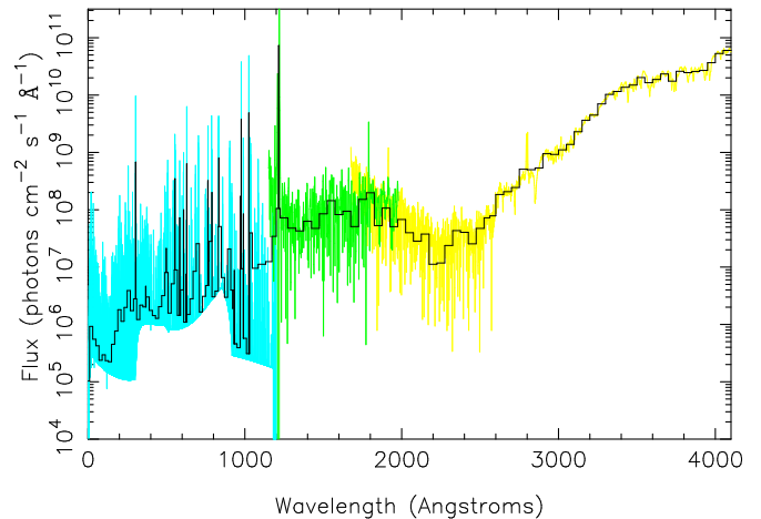
FIG. 3.— Adopted stellar ultraviolet spectrum for GJ 436 (black solid histograms) compared to NGSL spectra of GL 15B (yellow; see Heap & Lindler 2010), IUE spectra of GL 15B (green; Hubble MAST archive), and X-exoplanets theoretical spectra of GJ 436 (cyan; see Sanz-Forcada et al. 2011), all normalized to a distance of 1 AU. A color version of this figure is available in the online journal.
