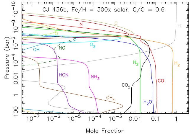
FIG. 15.— Mixing-ratio profiles for several species of interest (as labeled) in our kinetics/transport models for GJ 436b, for an assumed atmospheric metallicity of 300\times solar in carbon and nitrogen, with the oxygen elemental abundance defined through an assumed C/O ratio of 0.6 . The eddy diffusion coefficients are taken to be K_{zz} = 10^7 \text{ cm}^2 \text{ s}^{-1} at P \geq 10^{-4} bar, with K_{zz} increasing as the inverse square root of the pressure at P < 10^{-4} bar. The thermal profile is taken from Fig. 4 of Madhusudhan & Seager (2011), but we have shifted the entire profile upwards uniformly in an attempt to account for the higher-altitude photosphere with higher metallicities (see text). A color version of this figure is available in the online journal.
