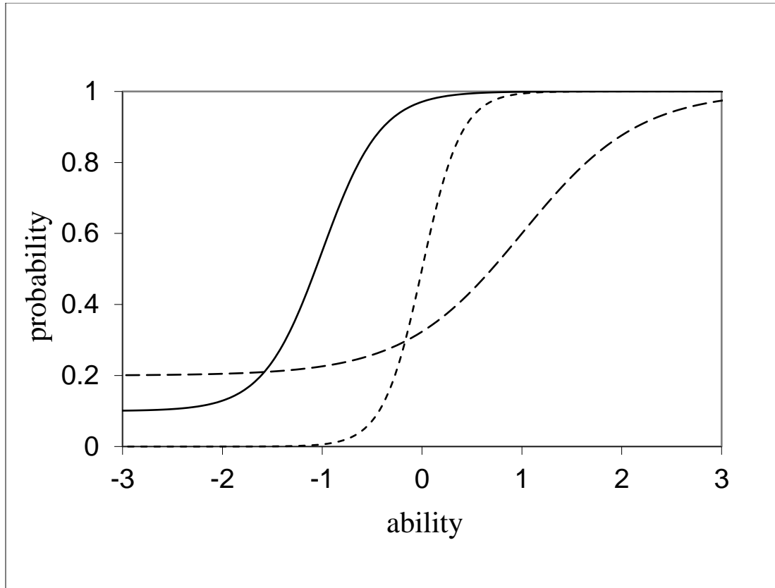
Figure 3. An example of a 3 PL model where the a , b , and c parameters differ across three items.
