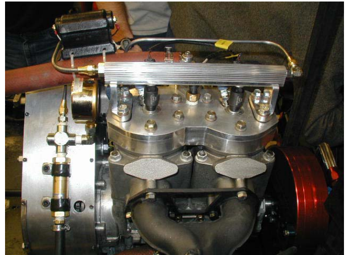
Figure 9: DFI Engine with Fuel Pump Drive on Left
