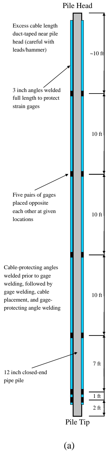
Figure 1. Placement of Strain Gages on Pipe Piles: (a) Schematic showing position of strain gage pairs, (b) Picture showing strain gages welded to pipe pile, (c) placement of strain gages on each of the three instrumented piles at the construction yard.
