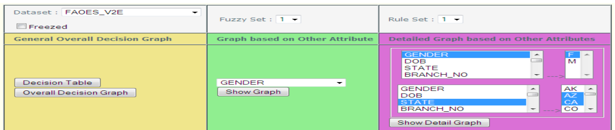
Figure 20: Analysis toolbox
