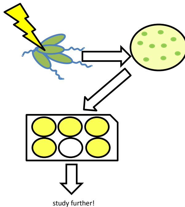
Figure 6. Representation of a transposon mutagenesis screen and high throughput \beta -Galactosidase assay. Lightning bolt represents mutagenesis of Pseudomonas cells by the mariner transposon. Mutants are then spread on PIA gentamicin, and then inoculated into 96-well plates to screen for differences in reporter activity. Those with changes were selected for further study.
