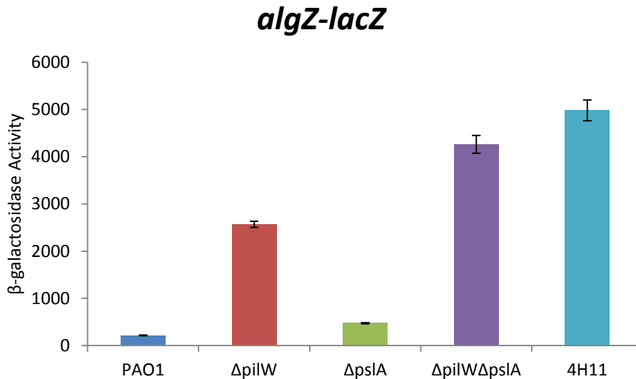
Figure 10. pslA alone is not responsible for regulation of algZ expression. β-Galactosidase assays performed in triplicate at 8 hours in LB broth. Statistical comparison of Δ pslA to PAO1 is not significant, while comparison of PAO1 as well as pilW to the pslA pilW double mutant and the transposon mutant yields p < 0.001
