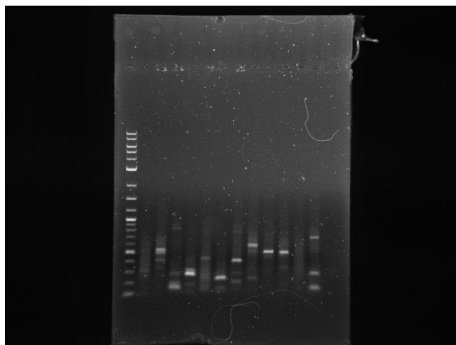
Figure 8. Gel electrophoresis of several successful arbitrary PCR products, amplified from transposon mutants.
