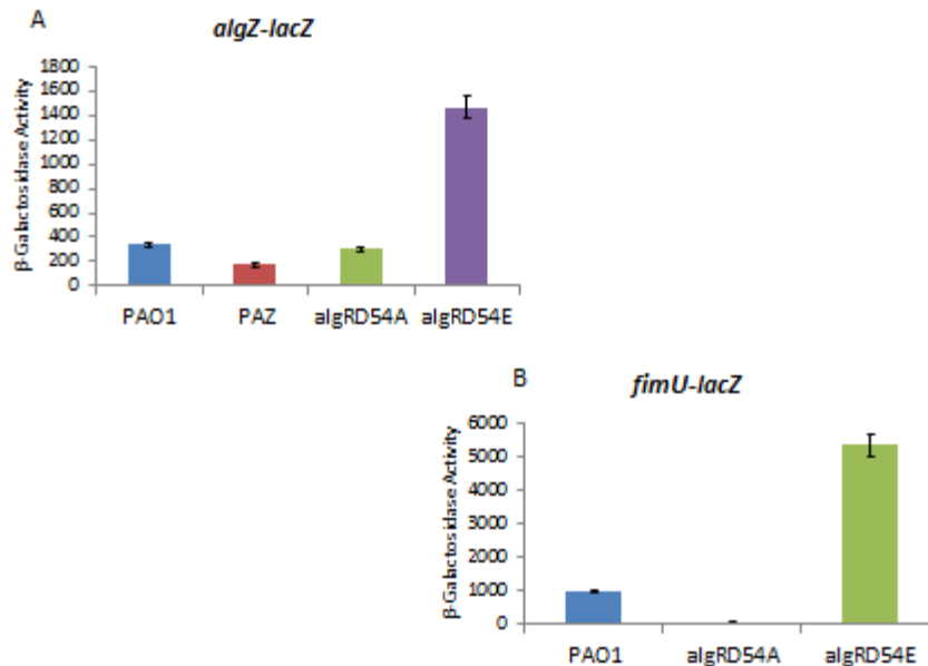
Figure 21. Phosphomimetic strains of AlgR do not influence expression of algZ or fimU to the same extent as a pilW mutant. A) Transcriptional fusion analysis of algZ . B) Transcriptional fusion analysis of fimU . \beta -Galactosidase assays performed in triplicate at 8 hours in LB broth. Statistical comparison of PAO1 versus algRD54E yields p < 0.001 in both cases, and comparison of PAO1 versus algRD54A yields p < 0.001 in the case of the fimU fusion
