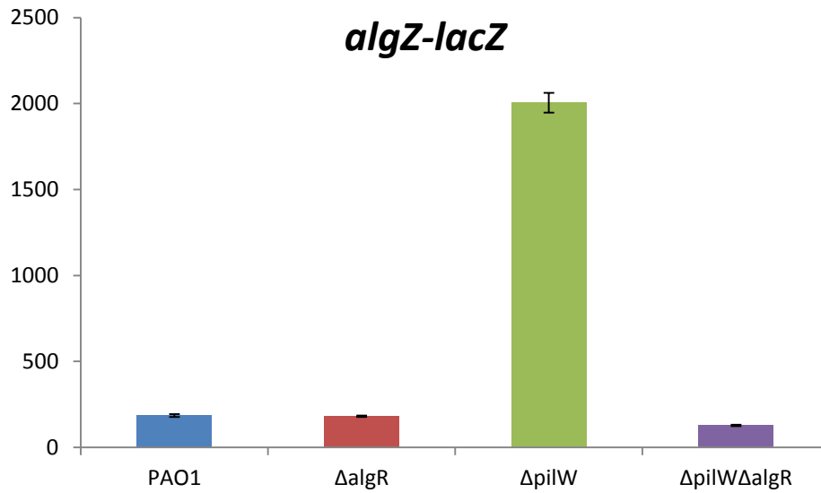
Figure 17. Expression of algZ is dependent on AlgR in the pilW mutant background. \beta -Galactosidase assays performed in triplicate at 8 hours in LB broth. Statistical comparison of \Delta pilW and \Delta pilW \Delta algR yields p < 0.001
