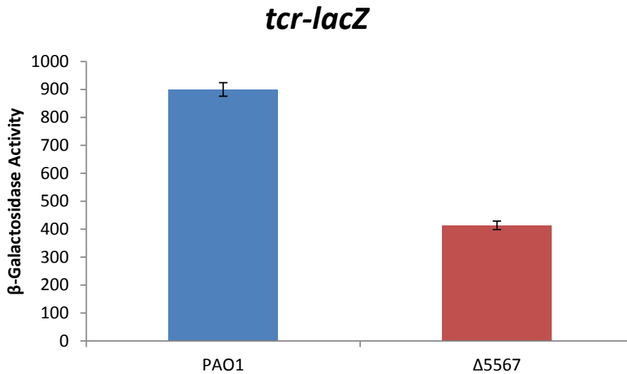
Figure 16. Activation of the tcr promoter is reduced in the PA5567 mutant, indicating a defect in this strain. β-Galactosidase assays performed in triplicate at 8 hours in LB broth. Statistical comparison of PAO1 and Δ5567 yields p < 0.001
