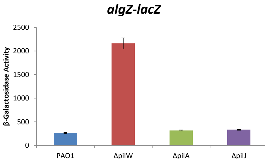
Figure 3. algZ expression is increased in a \Delta pilW strain. PAO1, \Delta pilW , \Delta pilA , and \Delta pilJ were assayed for \beta -Galactosidase activity. Assays performed in triplicate at 8 hours in LB broth. Statistical comparison of expression in PAO1 versus \Delta pilW yields p < 0.001 .
