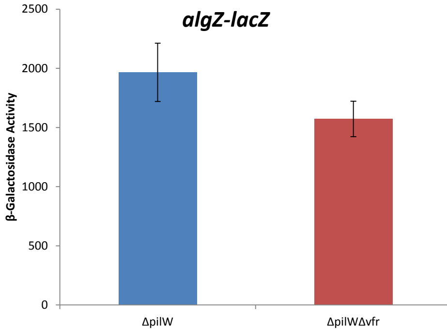
Figure 5. Vfr is not responsible for the increase in algZ expression in the pilW mutant background. β-Galactosidase assays performed in triplicate at 8 hours in LB broth.
