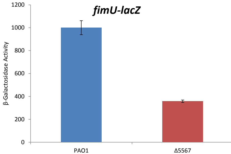
Figure 13. PA5567 regulates fimU expression through the activity of AlgR. β-Galactosidase assays performed in triplicate at 8 hours in LB broth. Statistical comparison of PAO1 and Δ5567 yields p < 0.001
