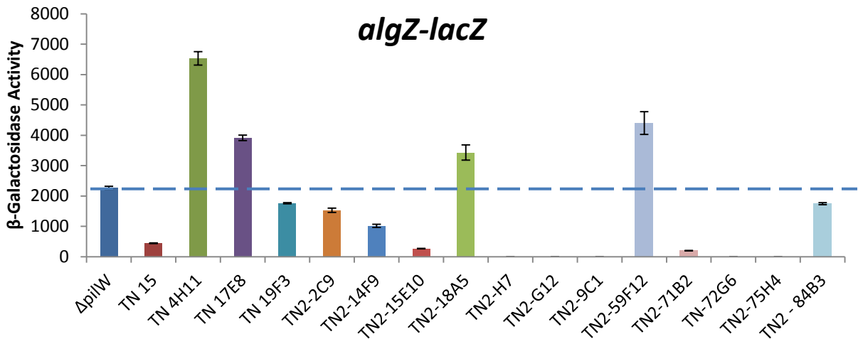
Figure 7. Transposon mutagenesis screen reveals mutants with both decreases and increases in algZ expression as compared to the pilW mutant reference strain. B-Galactosidase assays performed in triplicate at 8 hours in LB broth. Statistical comparison of expression in \Delta pilW versus transposon mutant yields p < 0.05 in each case.
