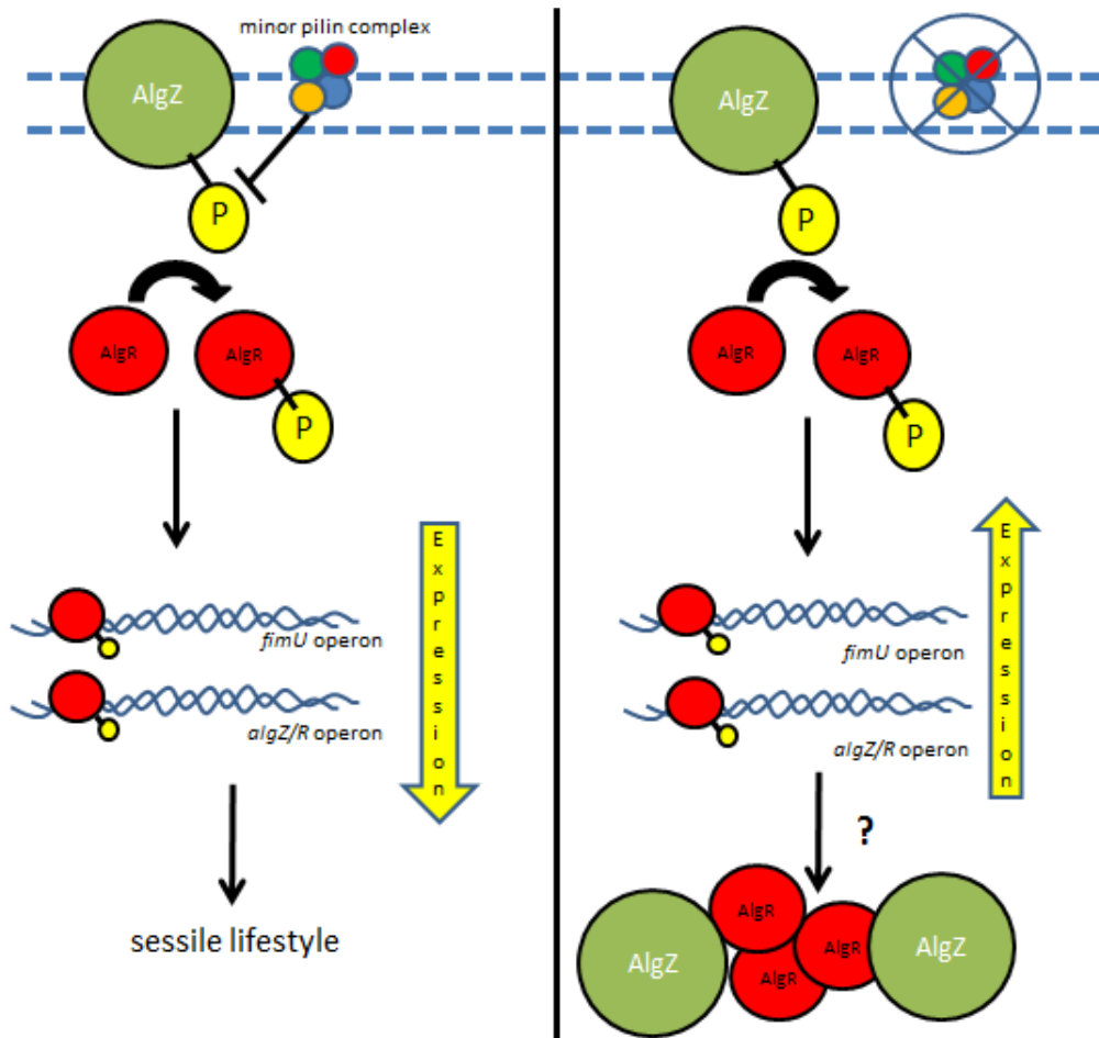
Figure 22. Proposed mechanism for the regulatory loop of AlgZ/R TCS and the minor pilin complex of TFP. In a pilated strain, bacteria can sense contact with a surface and decrease AlgR phosphorylation in preparation for surface-associated growth. In a minor pilin mutant, the signal cannot be transduced and so the bacteria continually upregulate both algZ/R and fimU in an attempt to sense their surroundings.
