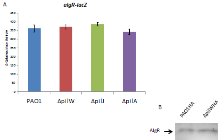
Figure 4. algR expression in the pilW mutant does not differ from wild-type. A) Transcriptional fusion analysis of algR . B) Western blot analysis of AlgR. β-Galactosidase assays performed in triplicate at 8 hours in LB.
