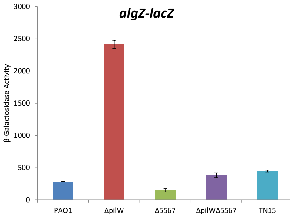
Figure 11. PA5567 regulates algZ expression independently of PilW. \beta -Galactosidase assays performed in triplicate at 8 hours in LB broth. Statistical comparison of PAO1 and \Delta 5567 yields p < 0.001 , as does comparison of \Delta pilW and the double mutant \Delta pilW\Delta 5567 .
