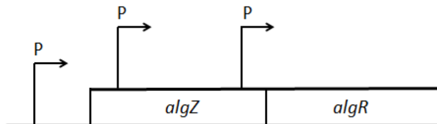
Figure 2. AlgZ/R operon. Promoters denoted with a “P” above a bent arrow.
