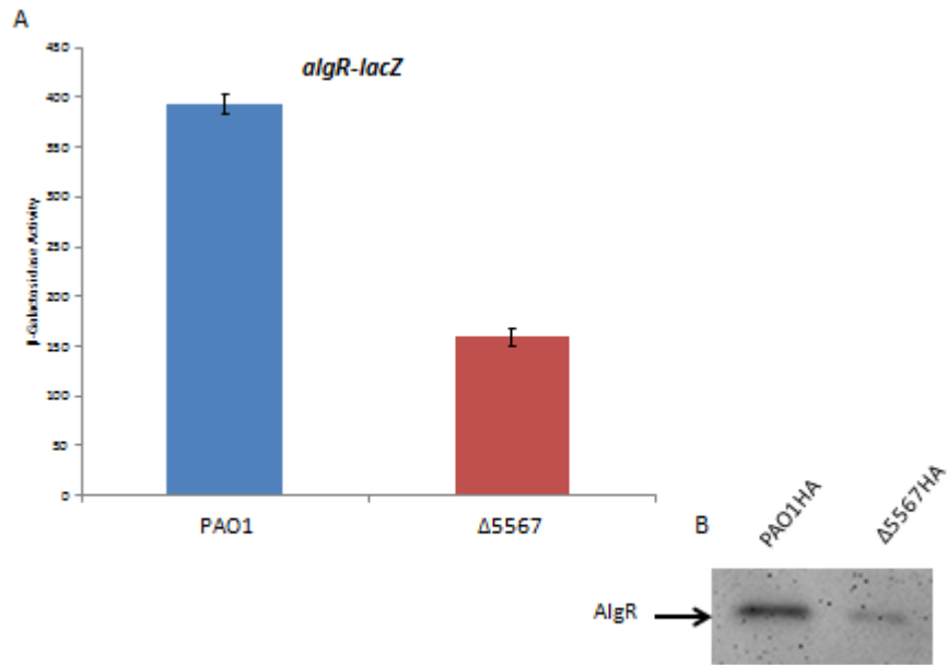
Figure 12. PA5567 influences algR expression. A) Transcriptional fusion analysis of algR . B) Western blot analysis of AlgR. Assays performed in triplicate at 8 hours in LB broth. Statistical comparison of PAO1 and Δ5567 yields p < 0.001
