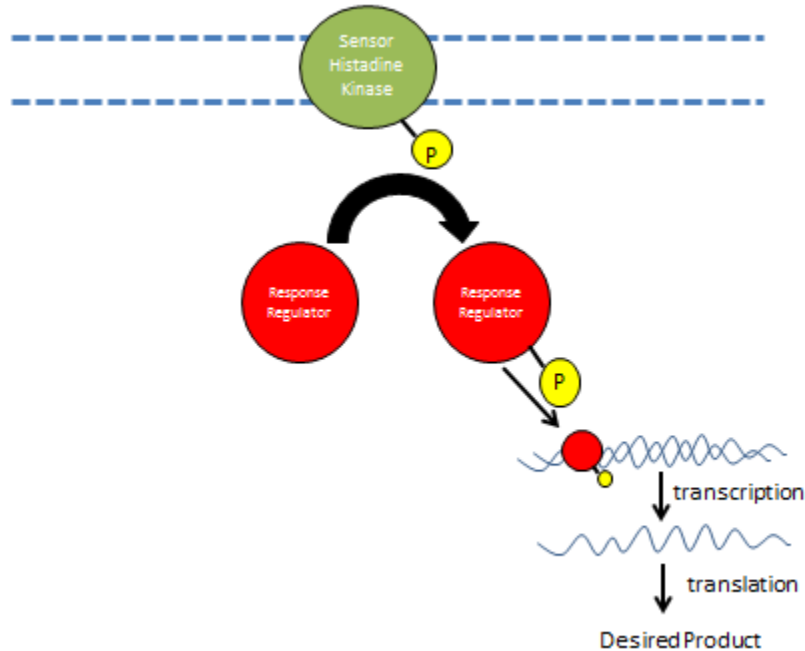
Figure 1. Diagram of a generic bacterial two-component system
