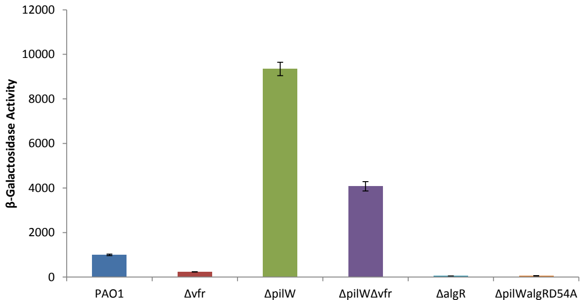
Figure 20. Phosphorylated AlgR is responsible for increase in fimU expression in the pilW mutant background. β-Galactosidase assays performed in triplicate at 8 hours in LB broth. Statistical comparison of \Delta pilW and \Delta pilW\Delta vfr , \Delta algR , and \Delta pilWalgRD54A yields p < 0.001
