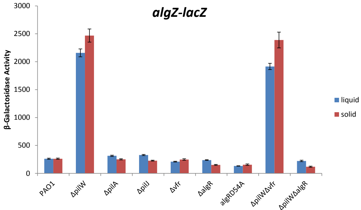
Figure 19. PilW is required for mechanosensory transduction on a solid surface. \beta -Galactosidase assays performed in triplicate at 8 hours in LB broth. Statistical comparison of PAOI and \Delta pilW and \Delta pilW\Delta vfr yields p < 0.001
