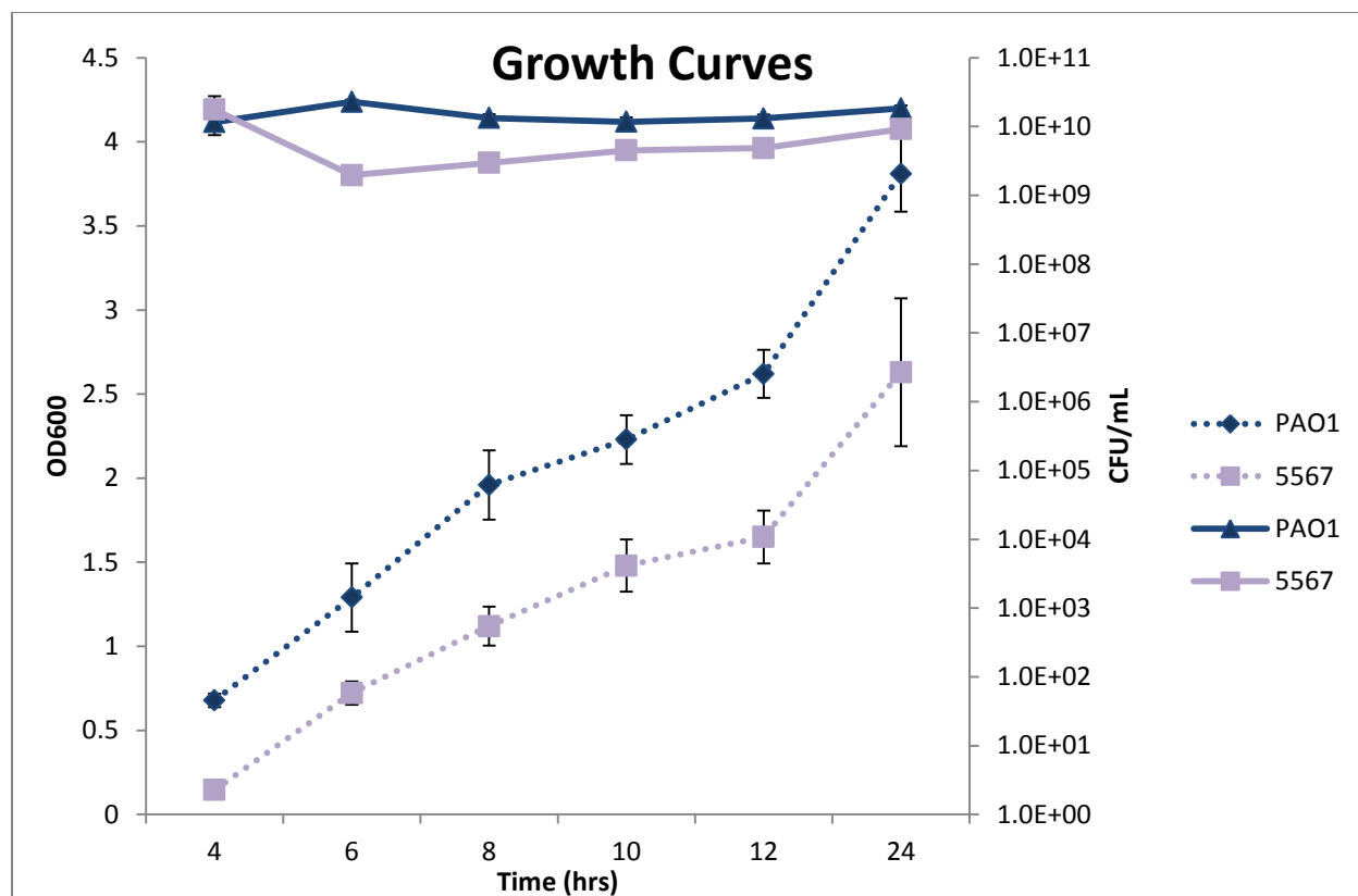
Figure 15. Growth curves of PAO1 and Δ5567. Solid lines indicate CFU/mL and correspond to the right axis of the figure. Dashed lines indicate OD600 and correspond to the left axis of the figure. Assays performed in triplicate. Statistical analysis for each time point comparing PAO1 to Δ5567 yields p > 0.05 at each time point, except for 6 hours for CFU/mL, which yields p < 0.05
