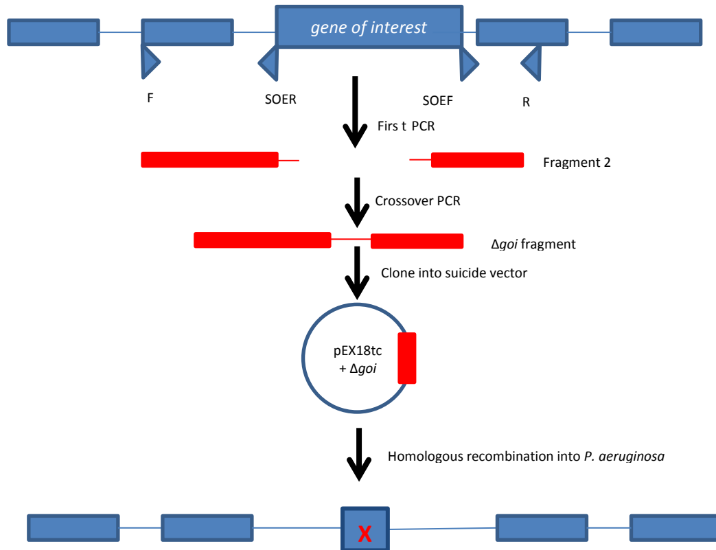
Figure 9. Diagram for construction of mutant strains. Blue triangles indicate primers utilized. Gene of interest also referred to as goi .
