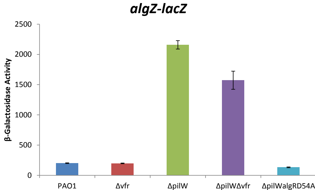
Figure 18. Increased algZ expression is due to activity of phosphorylated AlgR in the pilW mutant background. β-Galactosidase assays performed in triplicate at 8 hours in LB broth. Statistical comparison of ΔpilW and ΔpilWalgRD54A yields p < 0.001
