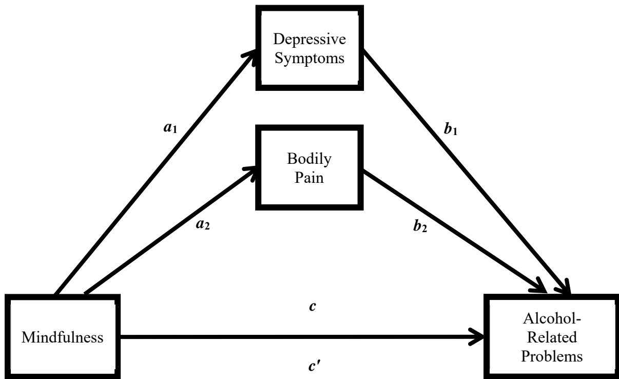
Figure 1. Graphic Illustration of a Parallel Mediation Model
