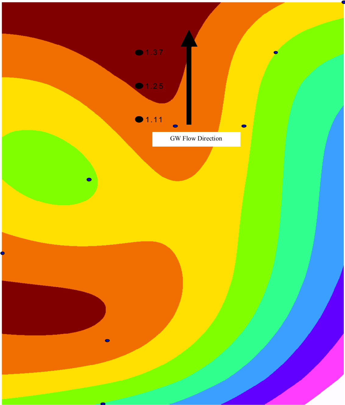
Figure 15 Interpolated 2D Map of Manganese Concentrations at Site N at T1 (<4 Weeks Post-ISCO)
