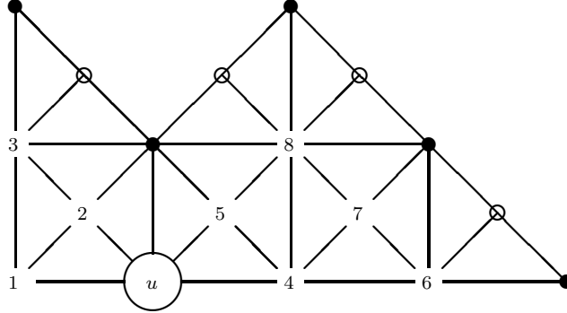
Figure 5.6. Parameterized Wavelet 6
